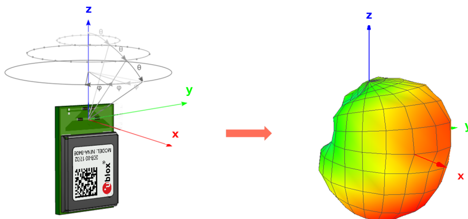
Figure 3: Measurement procedure for determining radiation patterns
