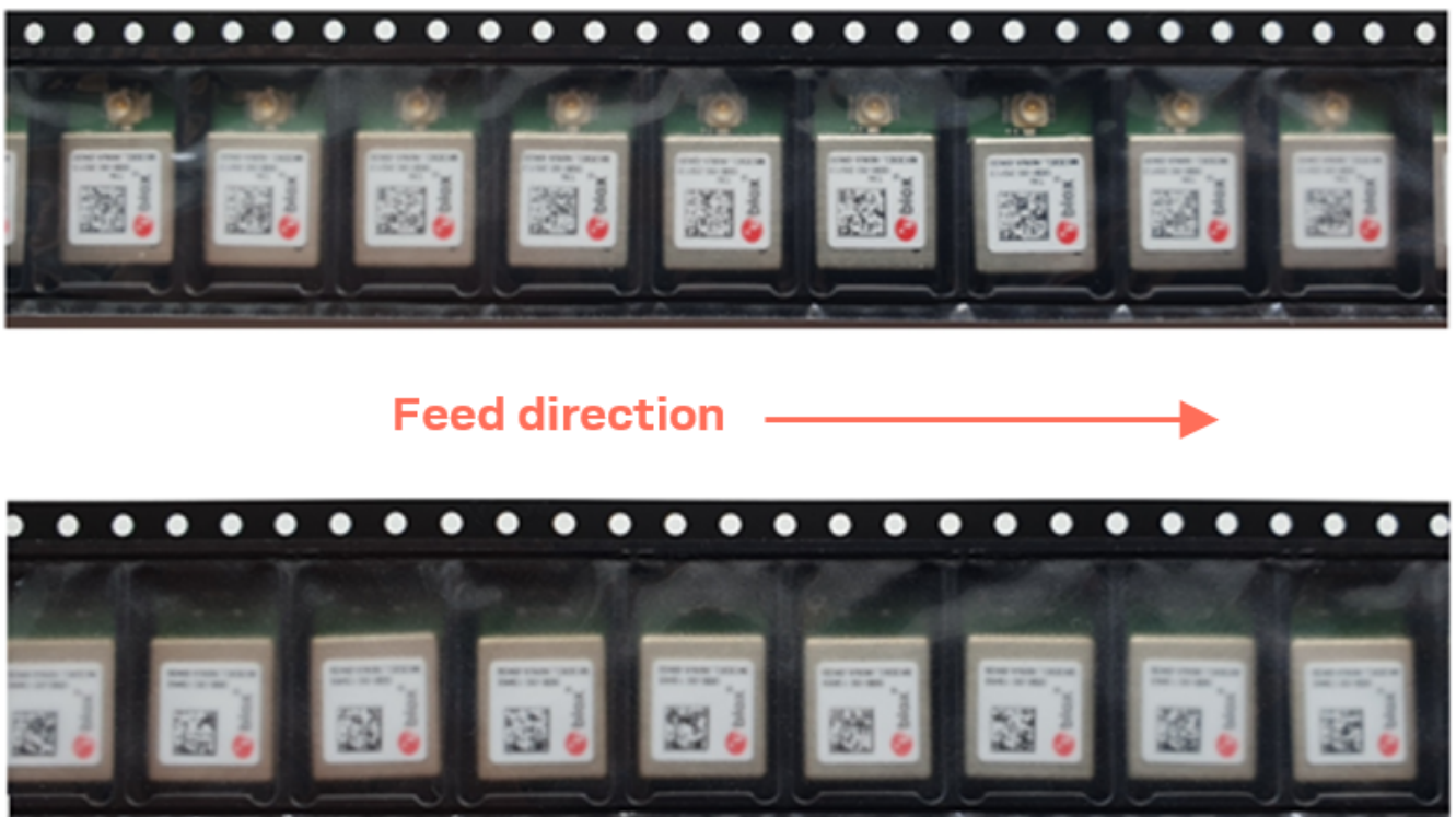
Figure 7: Orientation of NINA-B41 modules on tape
