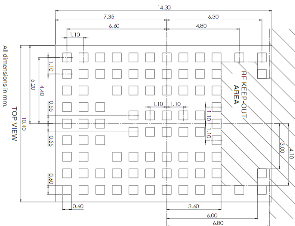
The suggested stencil layout for the MAYA-W2 module should follow the copper pad layout, as shown in Figure 14 . The “RF KEEP_OUT AREA” is only applicable on MAYA-W266 and MAYA-W276 when using the internal PCB antenna. The “RF KEEP_OUT AREA” can be omitted for the other module variants.
