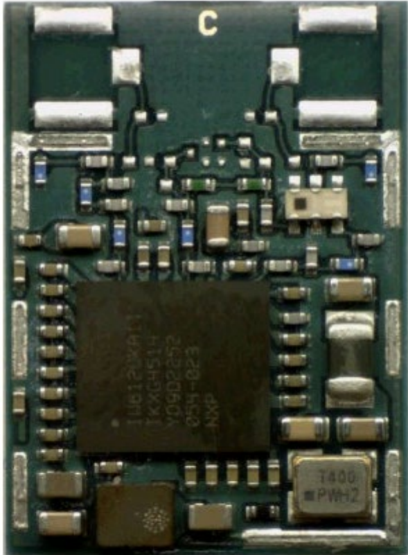
Figure 1: M2-MAYA-W271 internal photo
