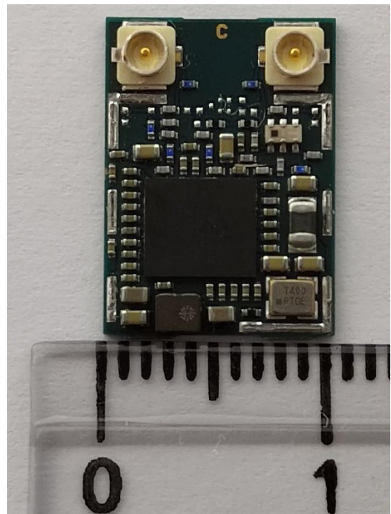
Figure 13 : MAYA-W260-00B top view width
