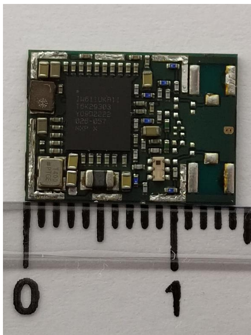
Figure 8 : MAYA-W261-00B top view length
