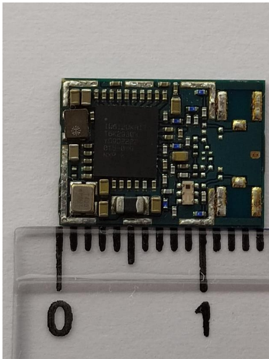
Figure 10 : MAYA-W271-00B top view length
