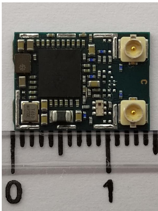
Figure 12 : MAYA-W260-00B top view length
