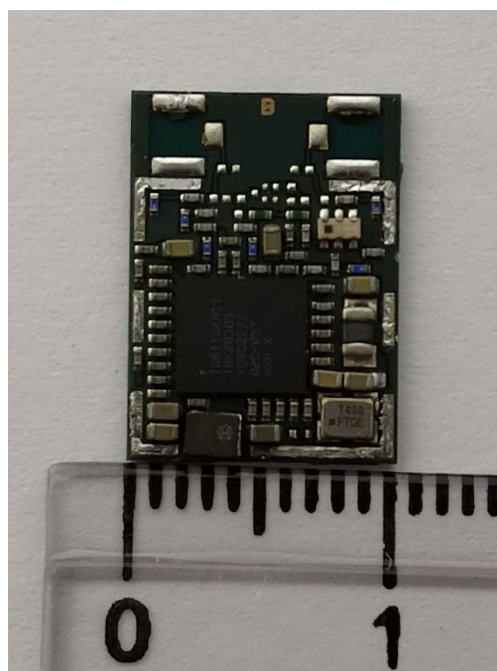
Figure 9 : MAYA-W261-00B top view width
