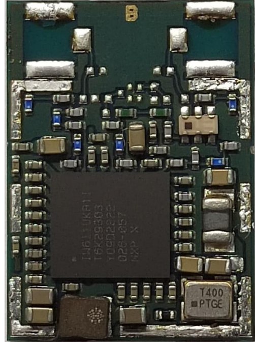
Figure 2: MAYA-W261-00B internal photo
