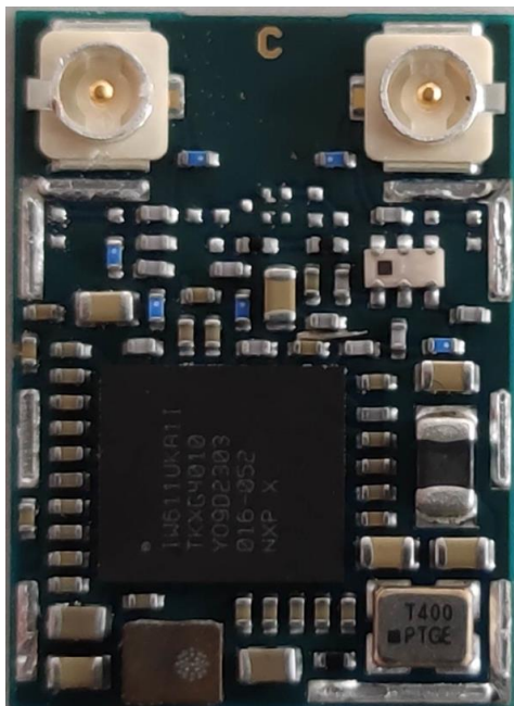
Figure 3: MAYA-W260-00B internal photo
