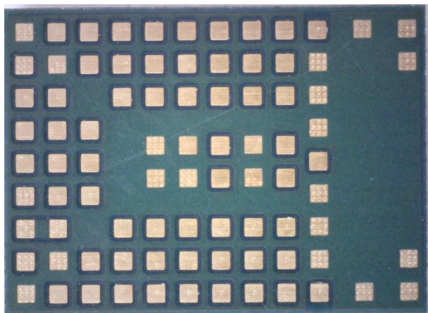
Figure 7: Bottom view of MAYA-W271-00B, MAYA-W261-00B and MAYA-W260-00B
