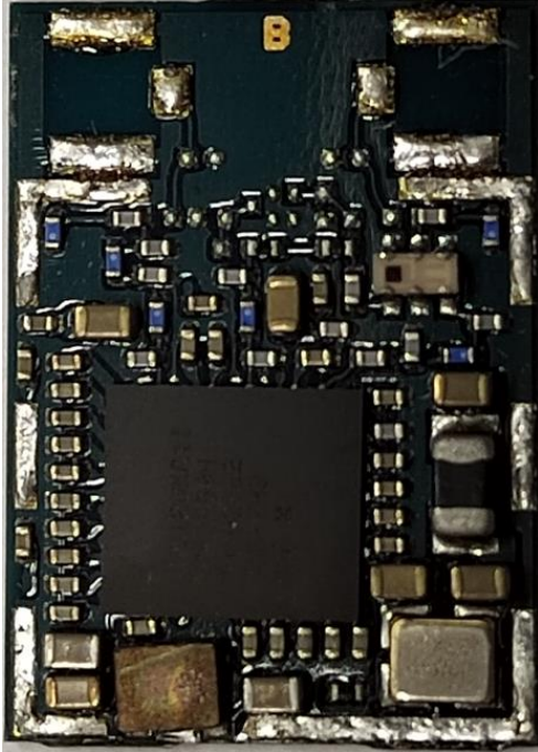
Figure 1: MAYA-W271-00B internal photo
