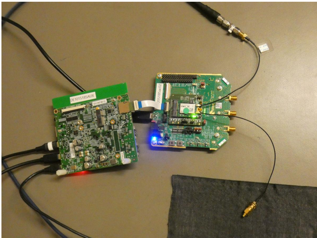
Photo 6: Test setup for conducted measurement EUT detail
