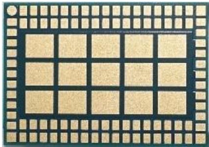
Figure 5: Bottom view of JODY-W562-00A module
