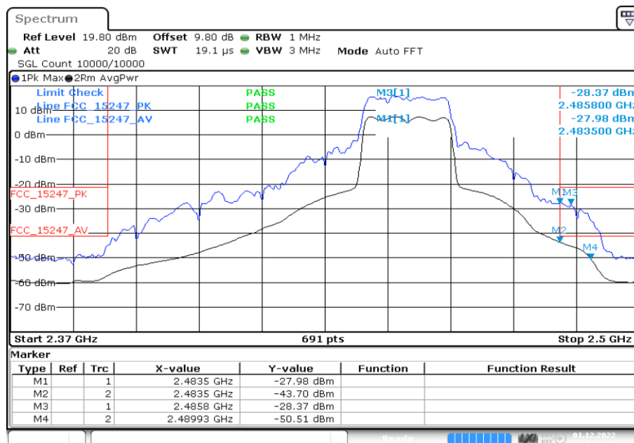
Channel 9 at power setting 16 dBm
