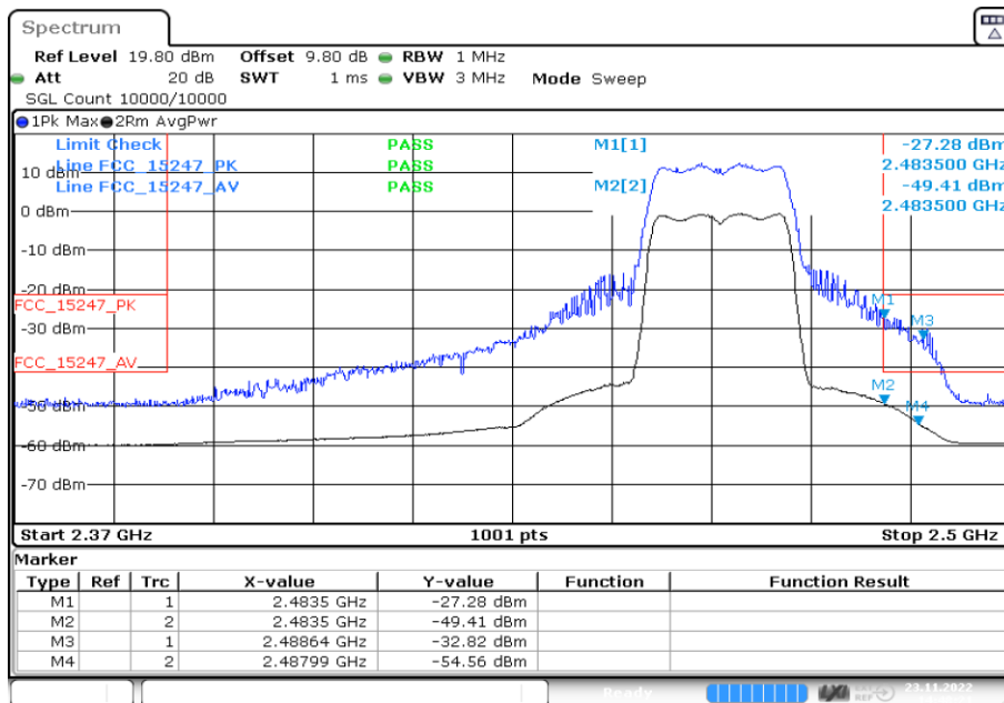
Channel 11 at power setting 12 dBm
