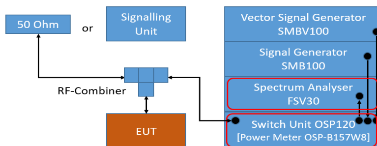
TS8997; Output Power
