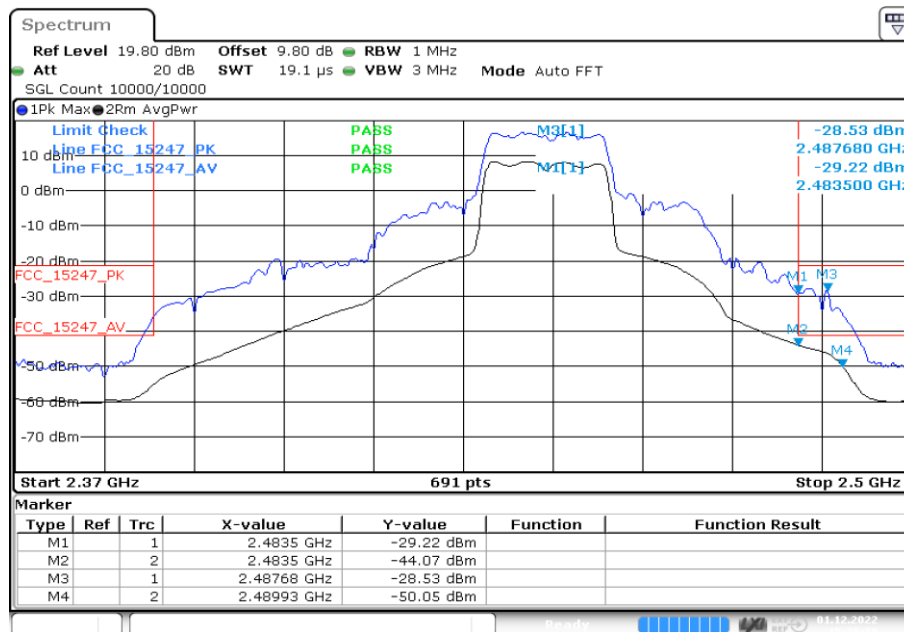
Channel 8 at power setting 17 dBm
