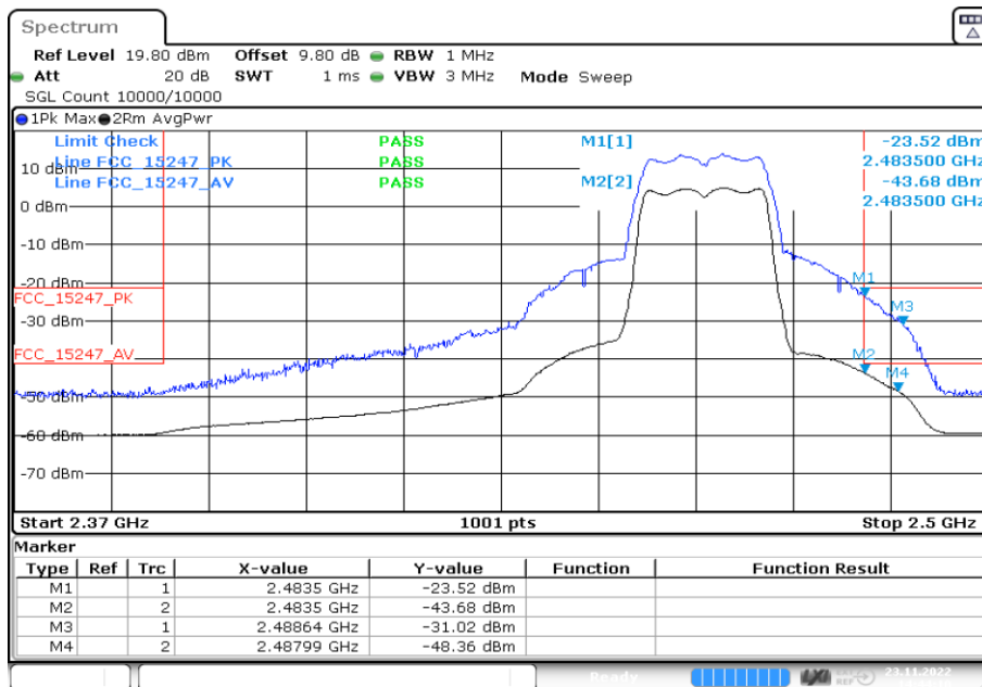
Channel 10 at power setting 15 dBm
