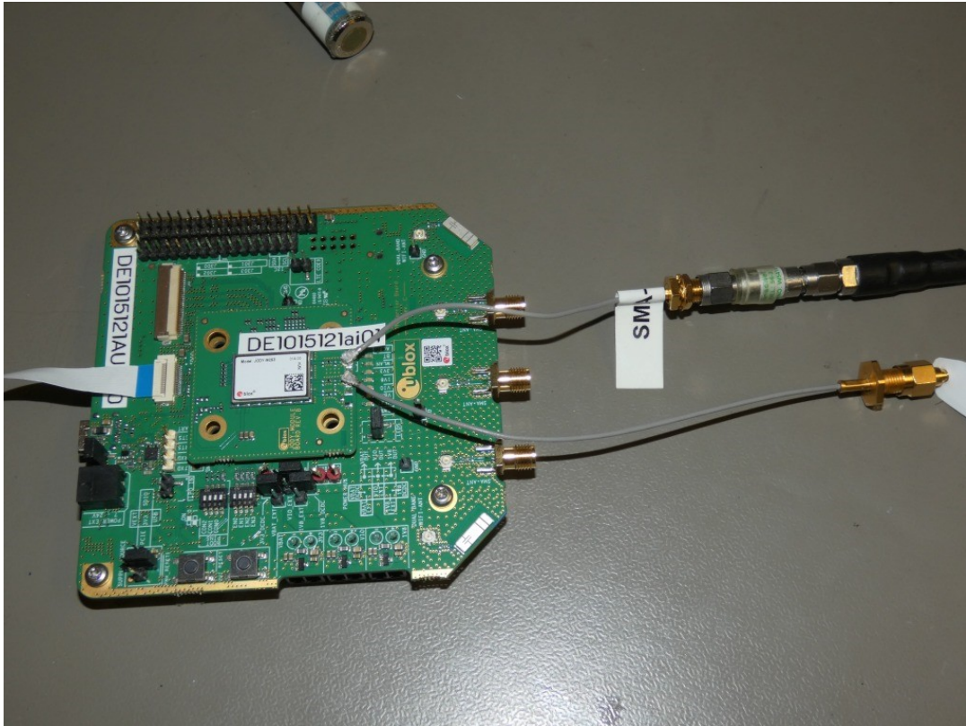
Photo 7: Test setup for conducted measurements EUT Detail
