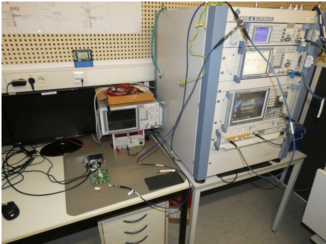
Photo 6: Test setup for conducted measurements
