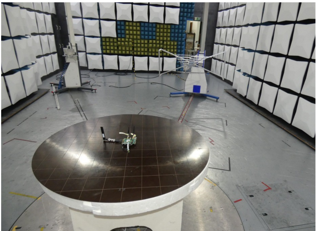
Photo 2: Test setup for radiated measurements below 1 GHz
