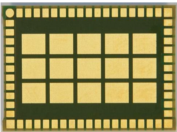
Figure 2: Bottom view for all module variants
