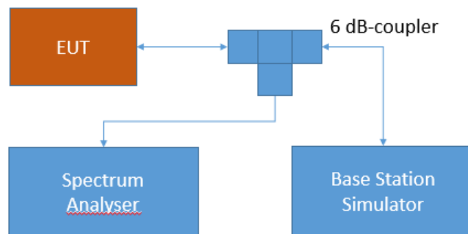
Test Setup FCC Part 22/24/27/90 Cellular;
