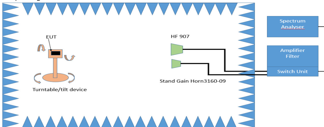
Test Setup; Spurious Emission Radiated (FAC), 1 GHz-26.5 GHz
