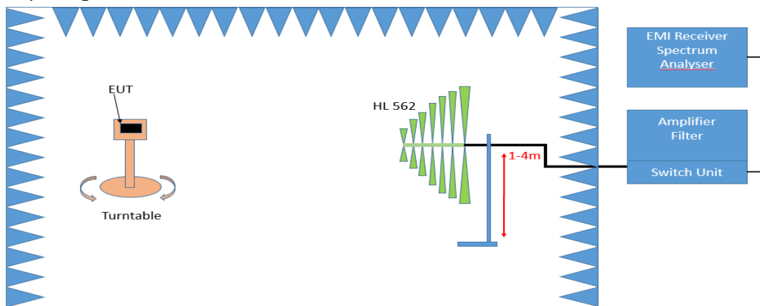
Test Setup; Spurious Emission Radiated (SAC), 30 MHz- 1GHz
