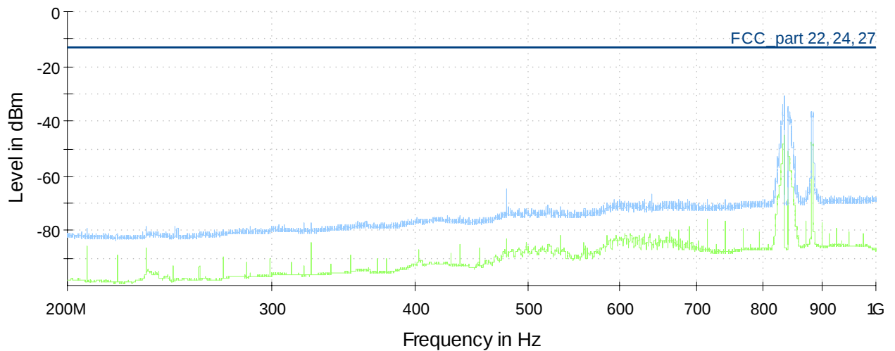
Results 200 MHz to 1 GHz
