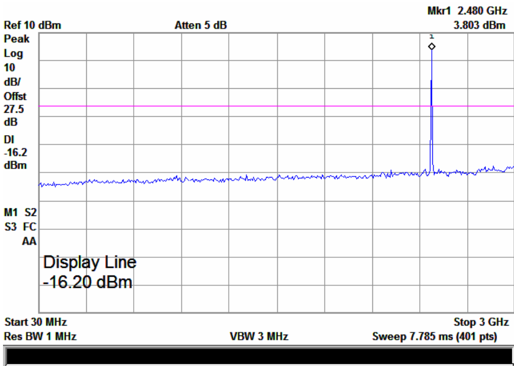
(Plot 9 Channel 78: 30MHz-3GHz)
