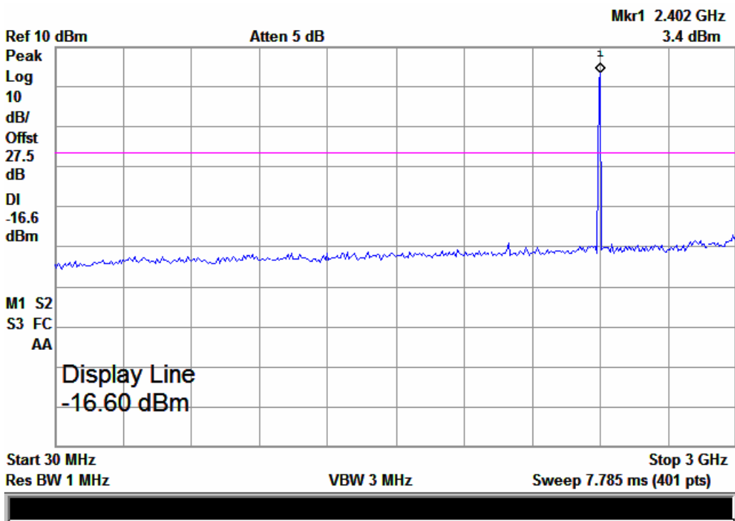
(Plot 5 Channel 0: 30MHz-3GHz)
