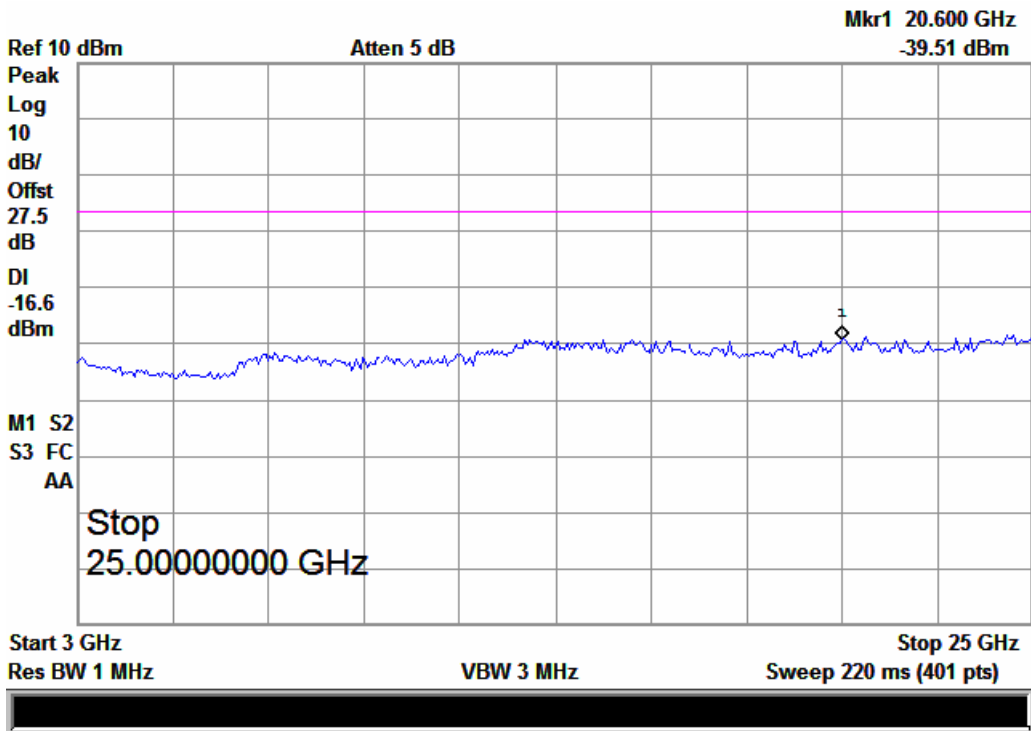
(Plot 6 Channel 0: 3GHz -25GHz)
