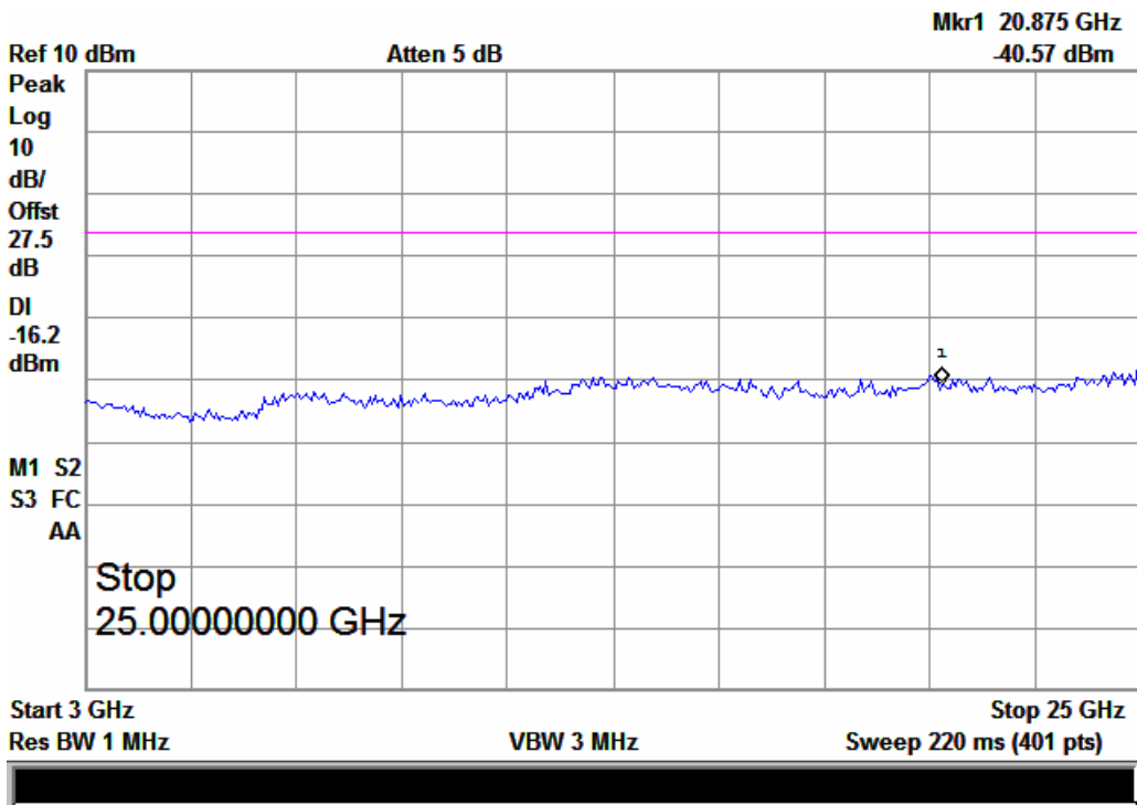
(Plot 8 Channel 39: 3GHz -25GHz)
