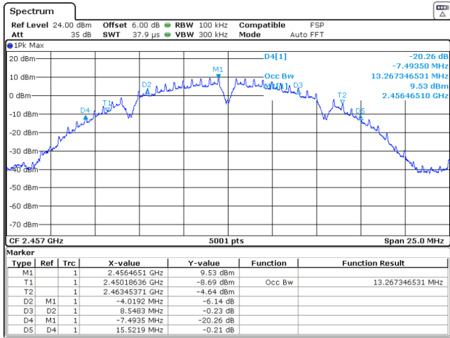
Figure 4.2.2 (i) Example Intentional Emission Bandwidth Plots.
