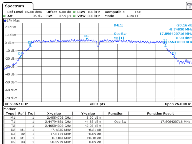
Figure 4.2.2 (iii) Example Intentional Emission Bandwidth Plots.
