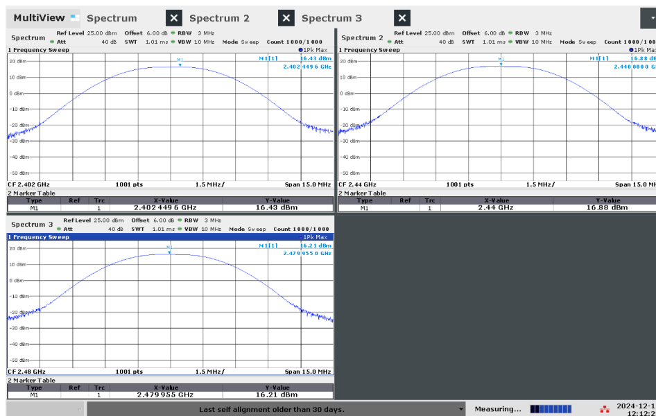
Figure 4.2.3 (ii) Conducted RF Power Plots
