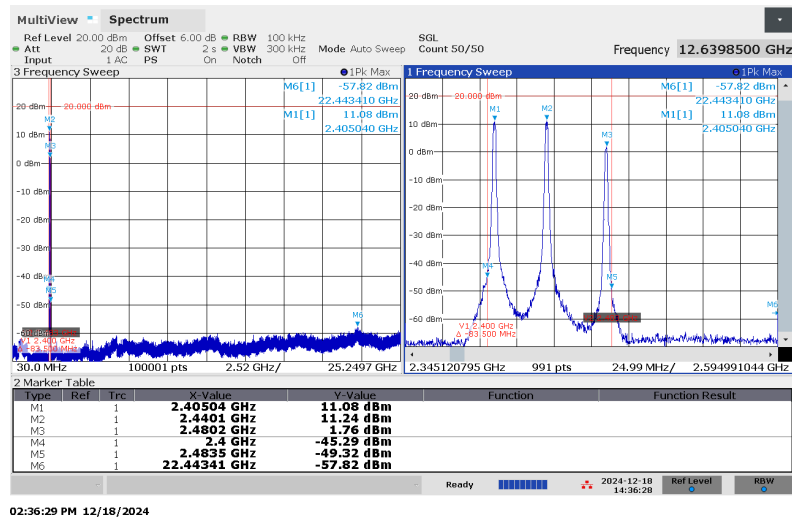
Figure 4.3.2 (ii) Worst Case Transmitter OOB Emissions Measured.
