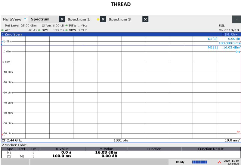
Figure 4.2.1 (iii) Example Pulsed Emission Characteristics (Duty Cycle).
