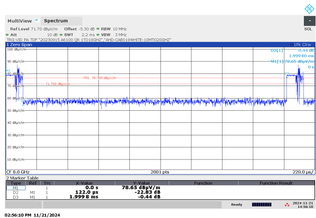
Figure 4.2.1 (ii) Example Pulsed Emission Characteristics (Duty Cycle).
