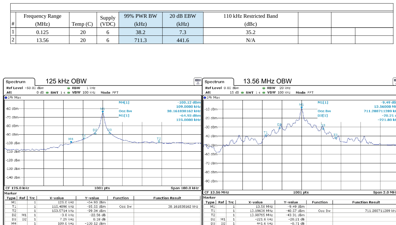
Figure 8: Intentional Emission Bandwidth.
