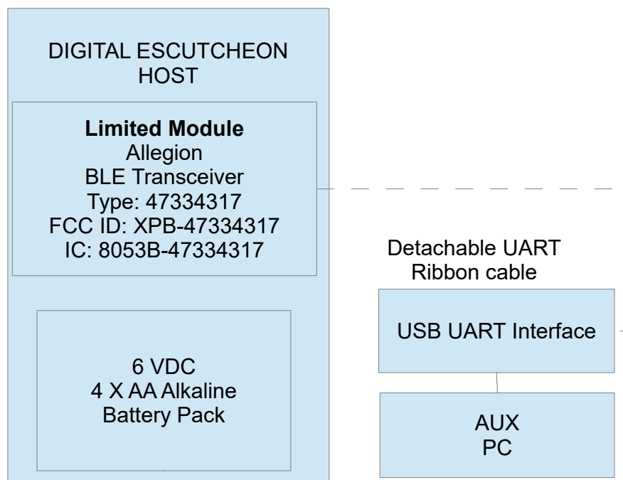
Figure 3.1.1 EUT Test Configuration Diagram.
