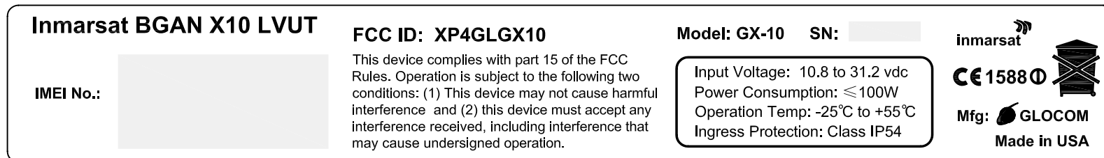
Fig.2 Chassis Label (dimensions: 200mm x 28.5mm)
