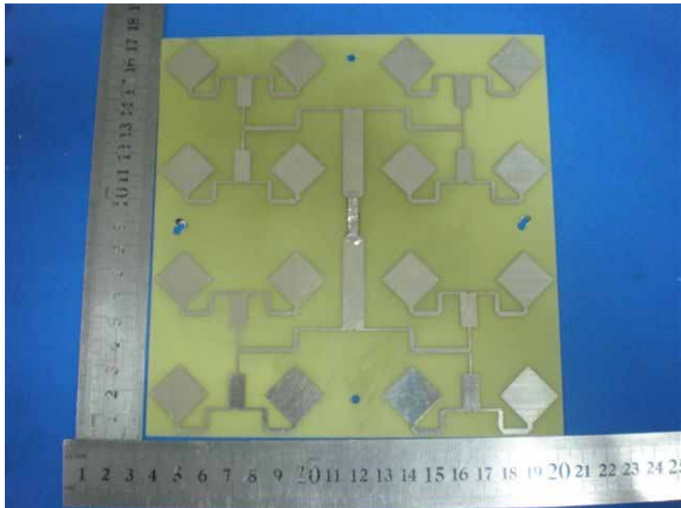
Photo 9 General Appearance of the EUT ( 5G Antenna )
