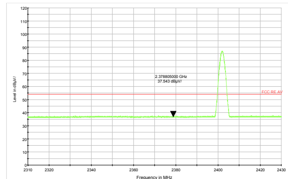
BLE(1Mbps) Channel 0 Average
