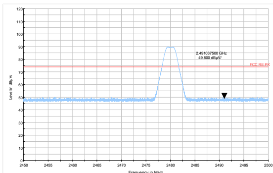
BLE(1Mbps) Channel 39 Peak
