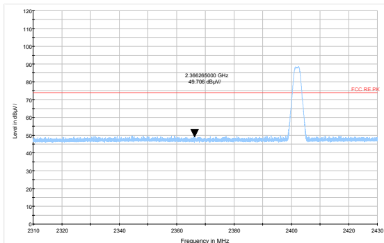
BLE(1Mbps) Channel 0 Peak
