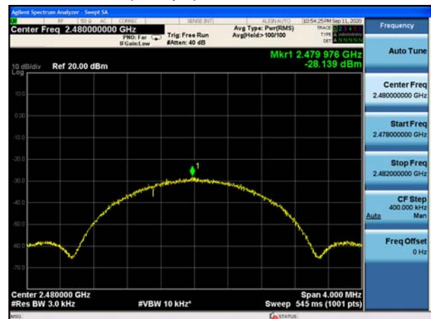
BLE(2Mbps), Channel No.: 39
