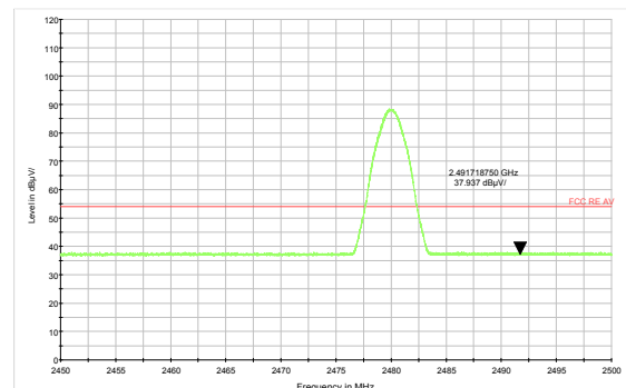
BLE(1Mbps) Channel 39 Average
