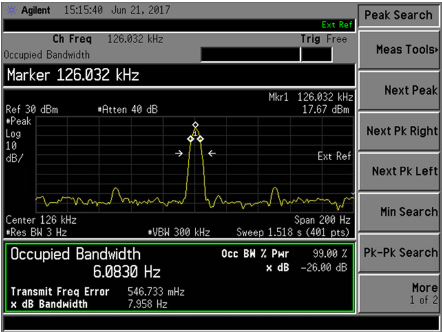
Figure 2 - Emission Bandwidth
