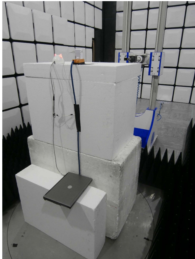
Figure 3 – Radiated Disturbance - 18 GHz to 25 GHz
