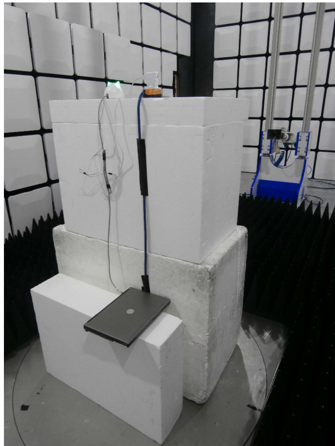
Figure 2 – Radiated Disturbance - 1 GHz to 18 GHz
