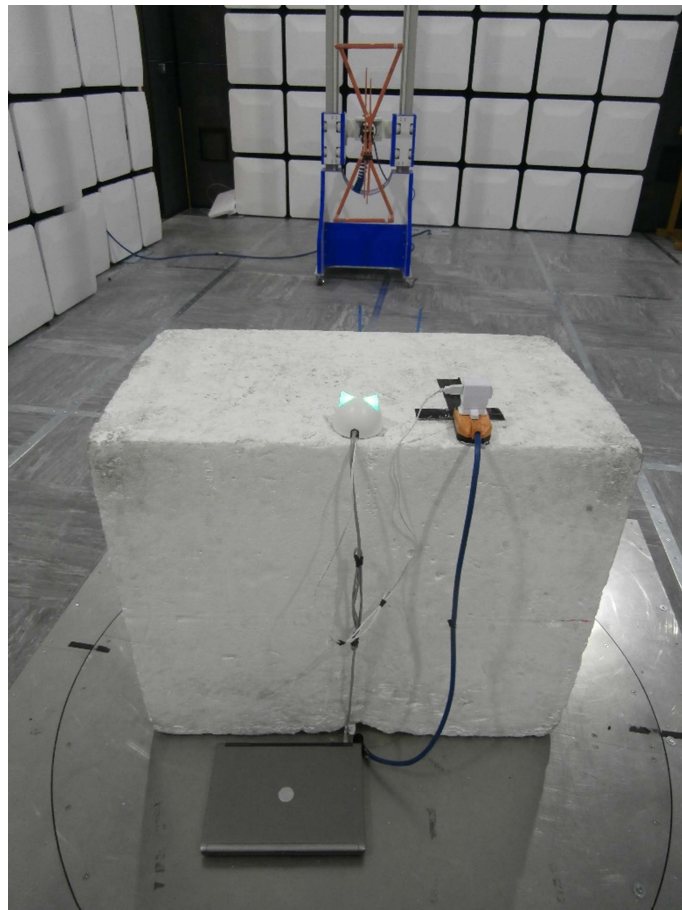
Figure 1 – Radiated Disturbance - 30 MHz to 1 GHz
