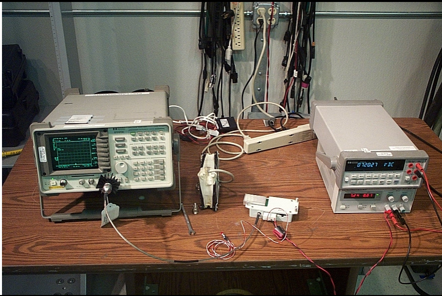
Frequency vs Voltage Stability Photo 9.
