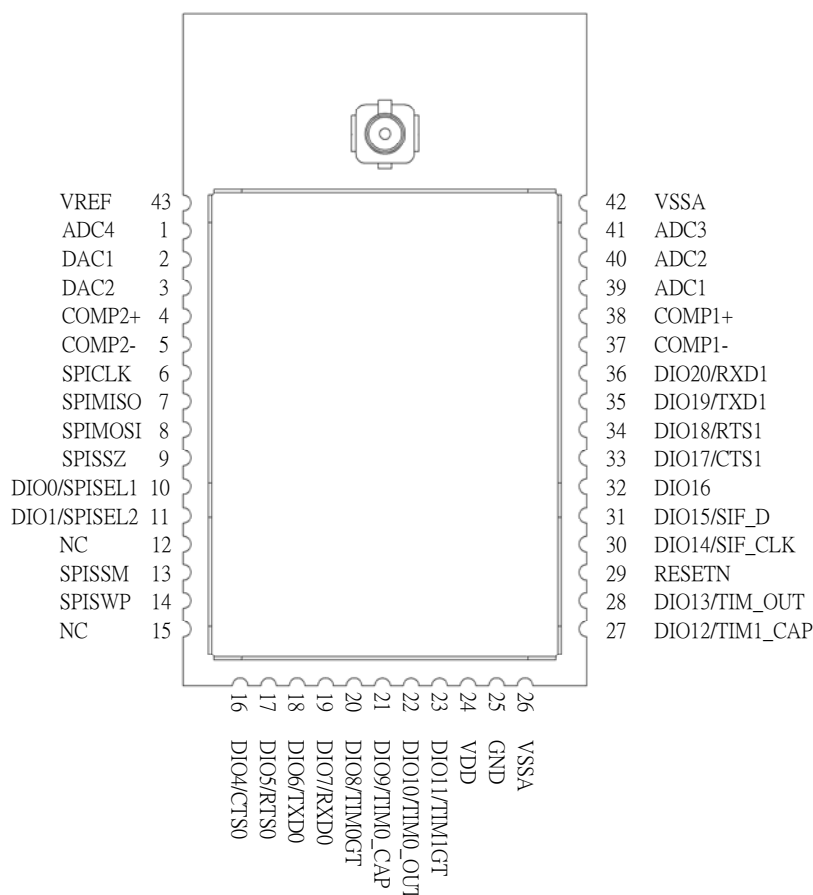
Figure: MD-120FC-5148A Pin Configuration (Top View)
