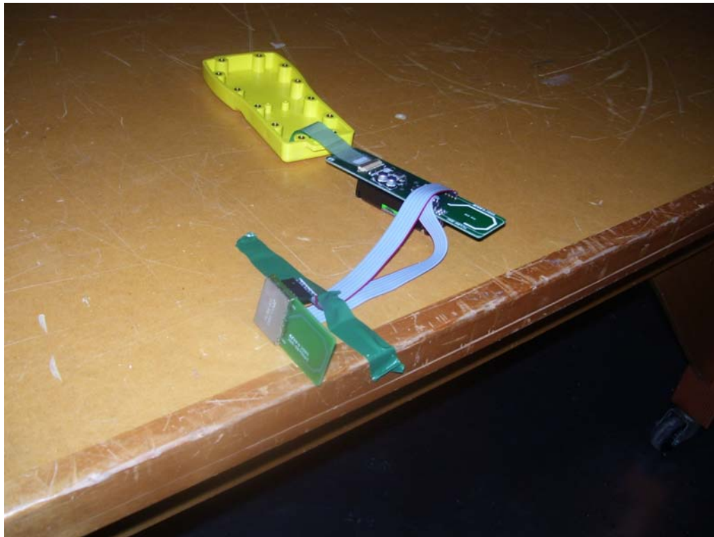
Figure 3 - Radiated Emissions Test Setup, Vertical Position
