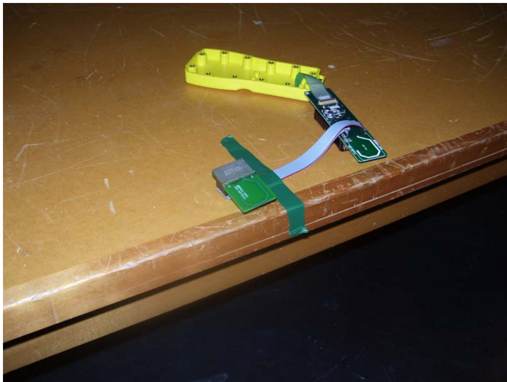
Figure 1 - Radiated Emissions Test Setup, Horizontal Position
