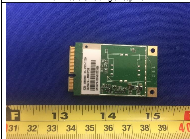
Main Board Shielding on bottom View
