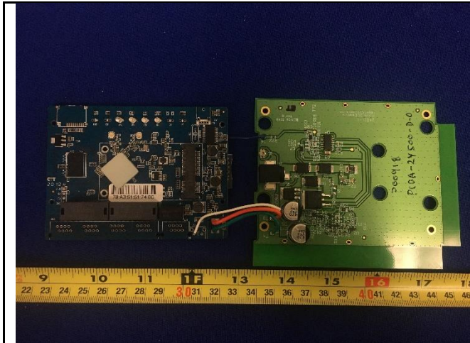
Main board and Antenna board view 1
