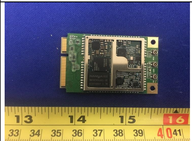
Main Board Shielding off top View
