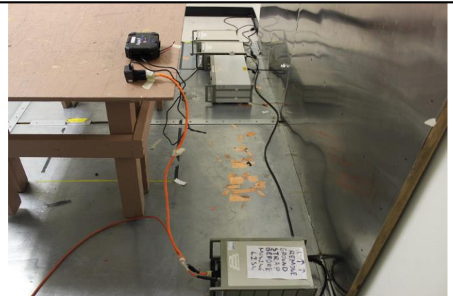
AC conducted emissions – Side View
