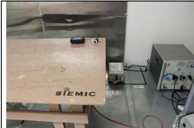
AC conducted emissions – Front View
