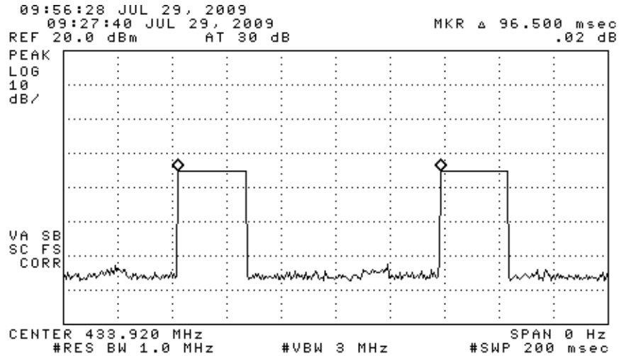
Figure 6.1. Transmission characteristics, (top) single packet length, (bottom) minimum packet period when the DUT is automatically for a second transmission
