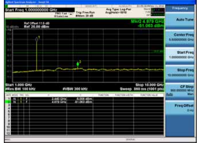
2441MHz(1GHz – 10GHz)
