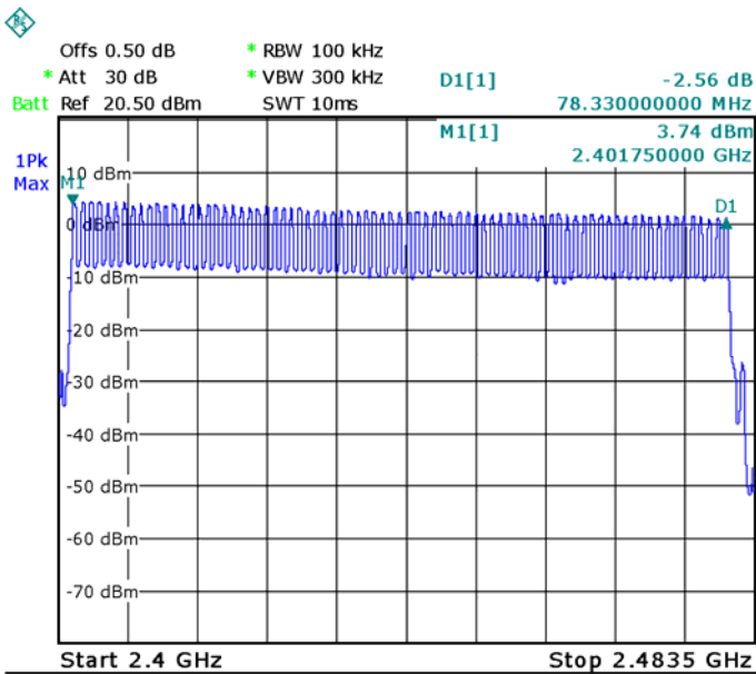
Modulation: GFSK
