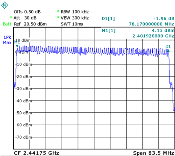
Modulation: 8DPSK
