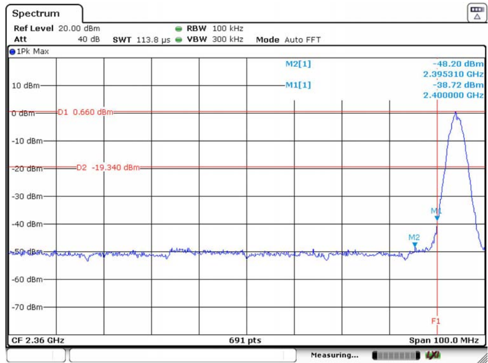
GFSK Low Channel ANT A1
