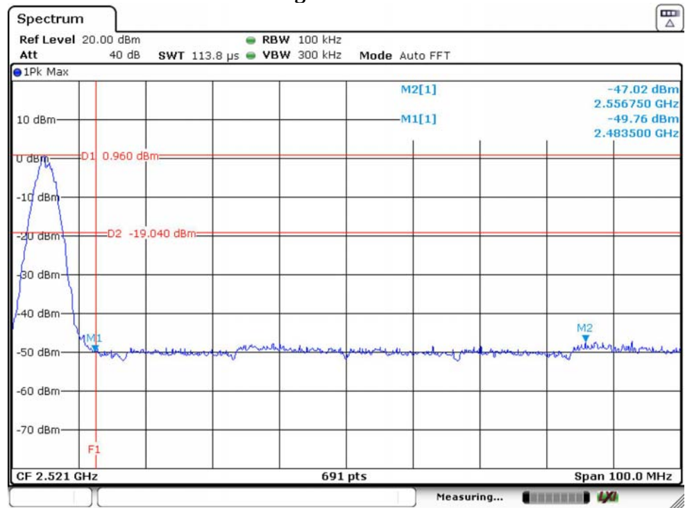
GFSK High Channel ANT A1
