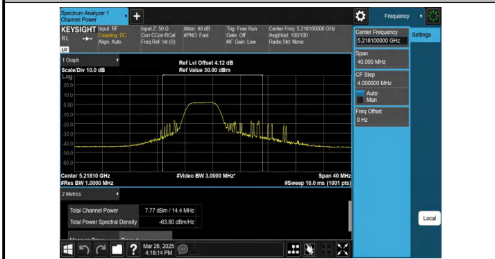
11AX20MIMO-Ant1-5220-106Tone-RU53-PASS
