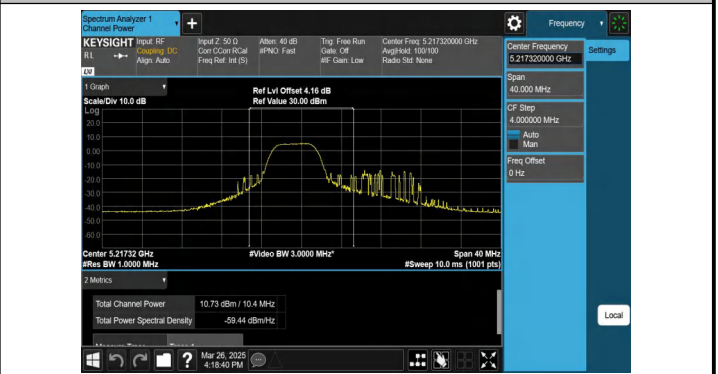
11AX20MIMO-Ant2-5220-106Tone-RU53-PASS
