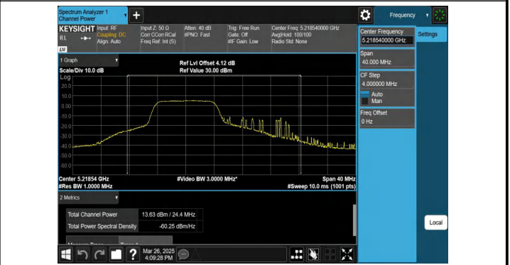
11AX20MIMO-Ant2-5240-26Tone-RU8-PASS
