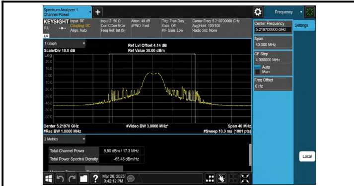
11AX20MIMO-Ant1-5220-52Tone-RU39-PASS
