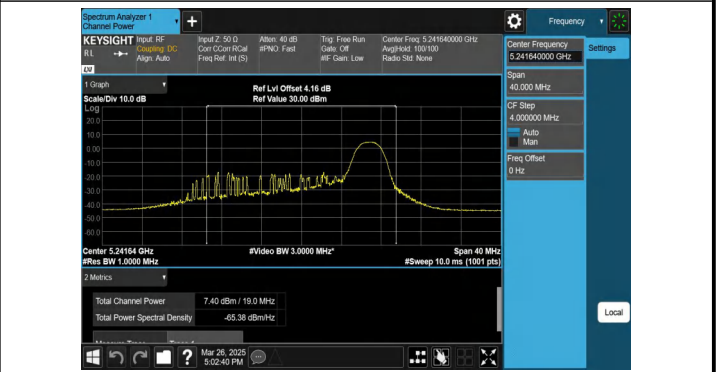
11AX20MIMO-Ant2-5240-52Tone-RU40-PASS
