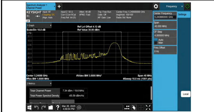
11AX20MIMO-Ant1-5240-52Tone-RU40-PASS
