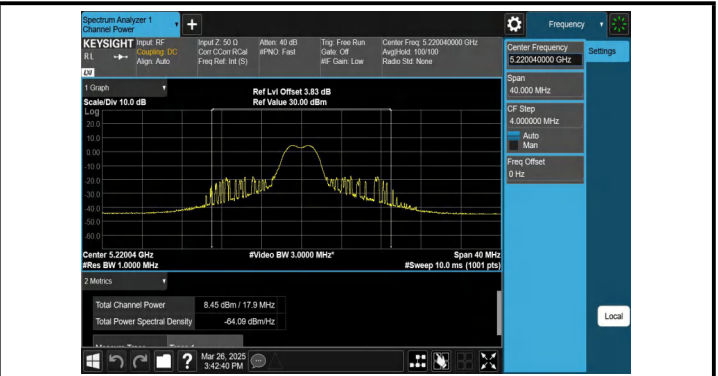
11AX20MIMO-Ant2-5220-52Tone-RU39-PASS
