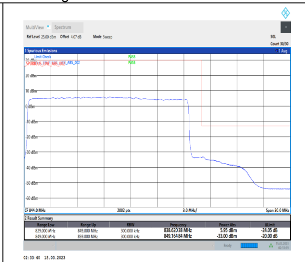
1-N5-PC3-15-20-H-3-DFT-PI2BPSK-Outer_Full-100@0-Ant1-1-seegraph-PASS-see graph
