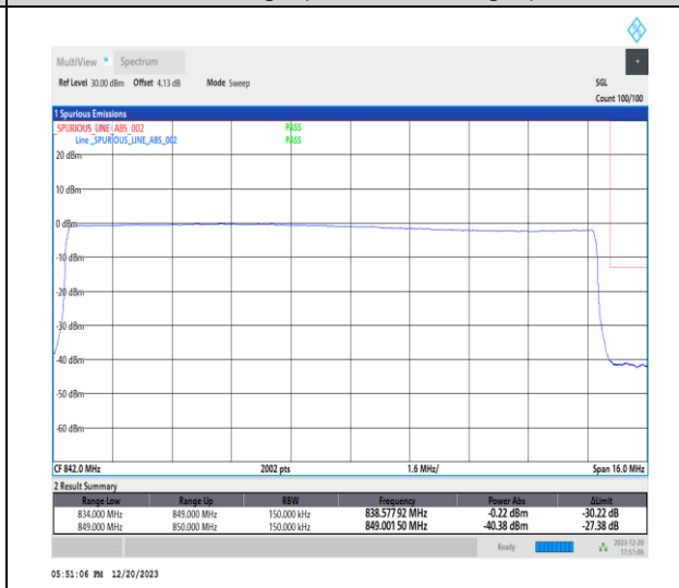
1-N515-15-H-6-CP-QPSK-Outer_Full-79@0-Ant1-1-seegraph-PASS-see graph
