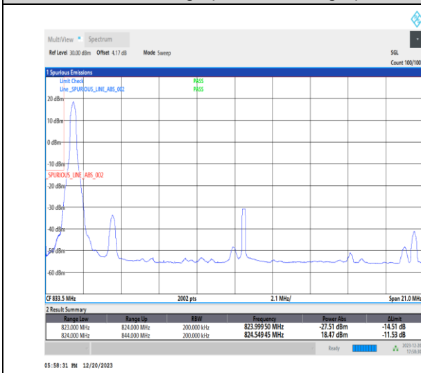
1-N515-20-L-4-CP-QPSK-Edge_1RB_Left-1@0-Ant1-1-seegraph-PASS-see graph
