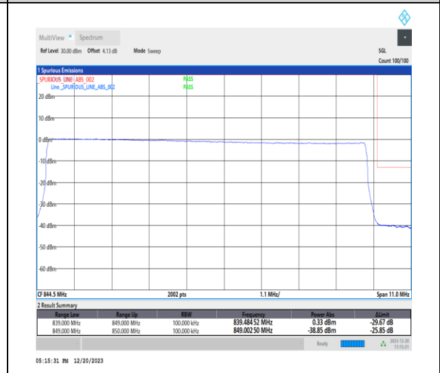
1-N515-10-H-6-CP-QPSK-Outer_Full-52@0-Ant1-1-seegraph-PASS-see graph
