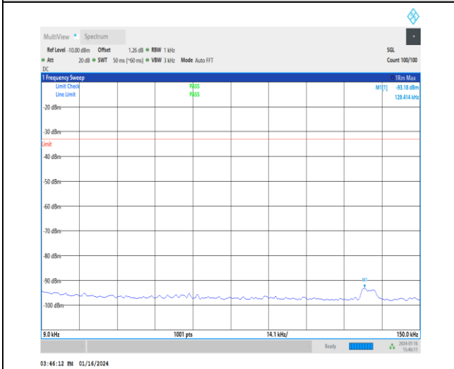
1-N5-15-20-H-1-DFT-PI2BPSK-Inner_1RB_Left-1@1 -0.009-0.15-Ant1-0.13--93.18--33-PASS
