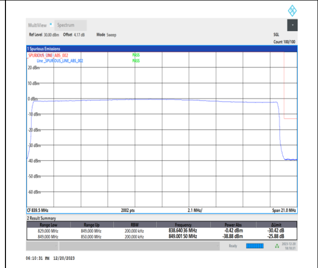
1-N515-20-H-6-CP-QPSK-Outer_Full-106@0-Ant1 -1-seegraph-PASS-see graph
