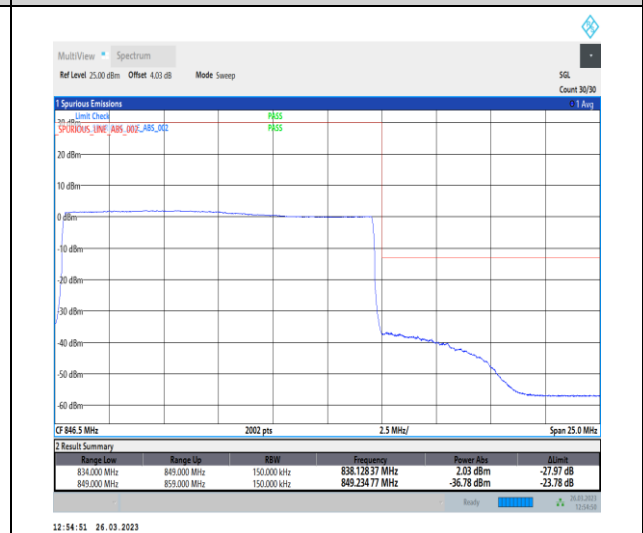
1-N5-PC3-15-15-H-6-CP-QPSK-Outer_Full-79@0-Ant1-1-seegraph-PASS-see graph
