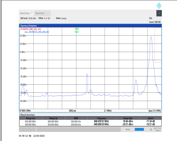
1-N515-20-H-5-CP-QPSK-Edge_1RB_Right-1@105-A nt1-1-seegraph-PASS-see graph
