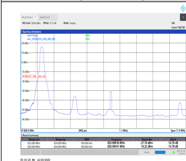
1-N515-10-L-4-CP-QPSK-Edge_1RB_Left-1@0-Ant1- 1-seegraph-PASS-see graph
