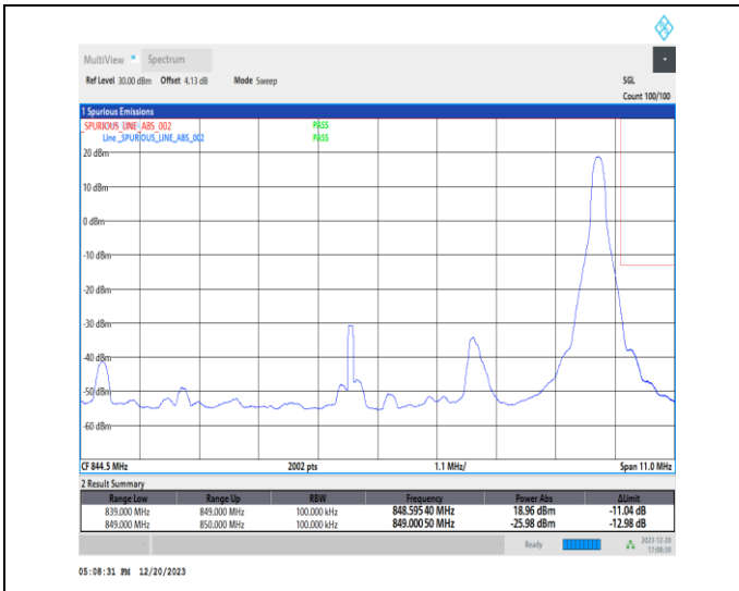
1-N515-10-H-2-DFT-PI2BPSK-Edge_1RB_Right-1@51-Ant1-1-seegraph-PASS-see graph
