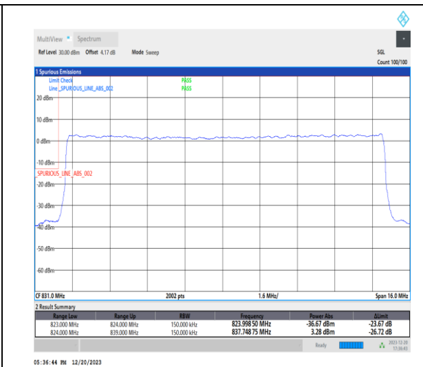
1-N515-15-L-3-DFT-PI2BPSK-Outer_Full-75@0-An t1-1-seegraph-PASS-see graph
