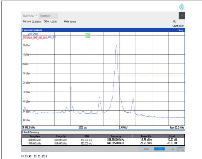
1-N5-PC3-15-15-H-2-DFT-PI2BPSK-Edge_1RB_Right-1@78-Ant1-1-seegraph-PASS-see graph
