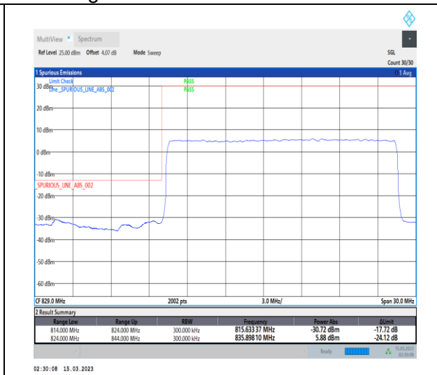
1-N5-PC3-15-20-L-3-DFT-PI2BPSK-Outer_Full-10 @0-Ant1-1-seegraph-PASS-see graph
