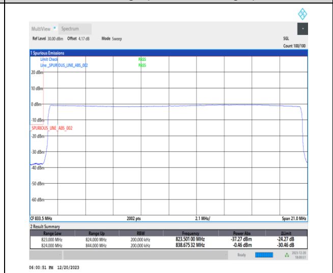
1-N515-20-L-6-CP-QPSK-Outer_Full-106@0-Ant1-1-seegraph-PASS-see graph
