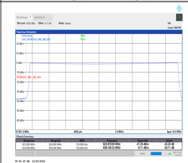
1-N515-15-L-6-CP-QPSK-Outer_Full-79@0-Ant1- -seegraph-PASS-see graph
