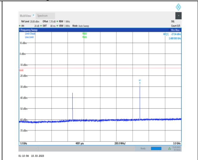
1-N5-PC3-15-20-H-1-DFT-PI2BPSK-Inner_1RB_Left -1@1-1000-3000-Ant1-2489.50--27.54--13-PASS
