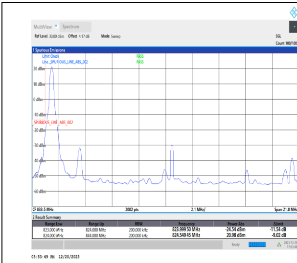
1-N515-20-L-1-DFT-PI2BPSK-Edge_1RB_Left-1@0-Ant1-1-seegraph-PASS-see graph
