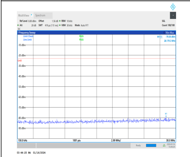
1-N5-15-20-M-1-DFT-PI2BPSK-Inner_1RB_Left-1@ 1-0.15-30-Ant1-1.46--79.54--23-PASS
