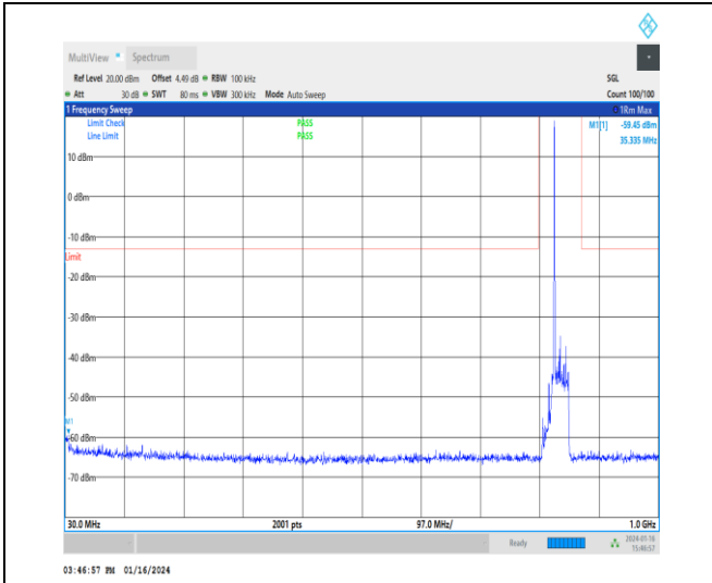
1-N5-15-20-H-1-DFT-PI2BPSK-Inner_1RB_Left-1@1 -30-1000-Ant1-32.91--59.45--13-PASS
