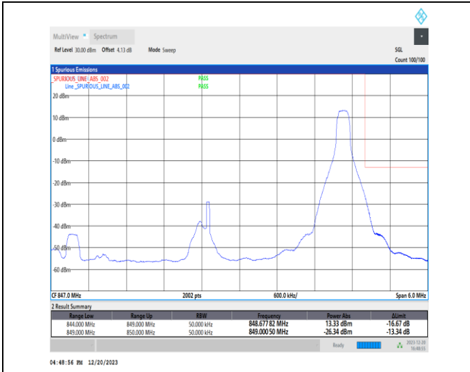
1-N515-5-H-2-DFT-PI2BPSK-Edge_1RB_Right-1@24-Ant1-1-seegraph-PASS-see graph
