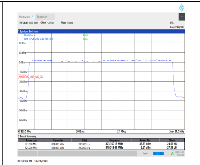
1-N515-20-L-3-DFT-PI2BPSK-Outer_Full-100@0-Ant1-1-seegraph-PASS-see graph
