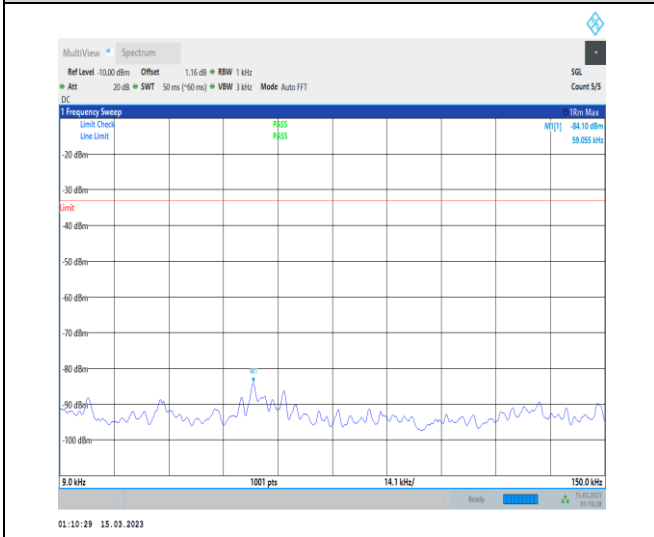
1-N5-PC3-15-20-H-1-DFT-PI2BPSK-Inner_1RB_Left -1@1-0.009-0.15-Ant1-0.06--84.10--33-PASS
