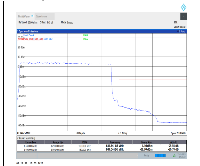
1-N5-PC3-15-15-H-3-DFT-PI2BPSK-Outer_Full-75@0-Ant1-1-seegraph-PASS-see graph
