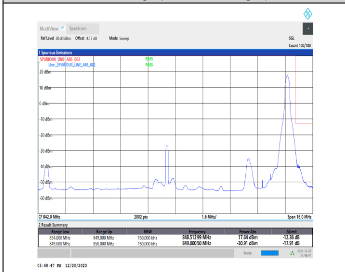
1-N515-15-H-5-CP-QPSK-Edge_1RB_Right-1@78-Ant1-1-seegraph-PASS-see graph
