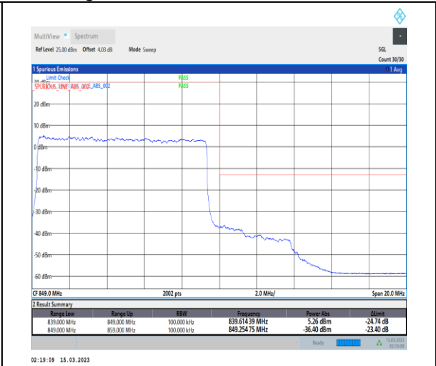
1-N5-PC3-15-10-H-3-DFT-PI2BPSK-Outer_Full-50@0-Ant1-1-seegraph-PASS-see graph
