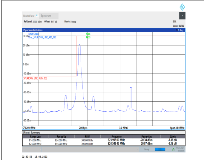
1-N5-PC3-15-20-L-4-CP-QPSK-Edge_1RB_Left-1 @0-Ant1-1-seegraph-PASS-see graph
