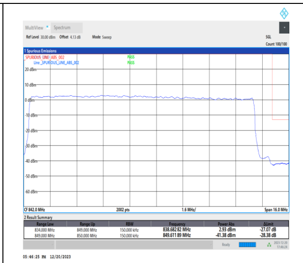
1-N515-15-H-3-DFT-PI2BPSK-Outer_Full-75@0-Ant1-1-seegraph-PASS-see graph
