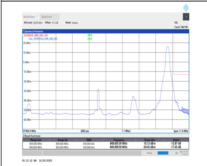
1-N515-10-H-5-CP-QPSK-Edge_1RB_Right-1@51-Ant1-1-seegraph-PASS-see graph
