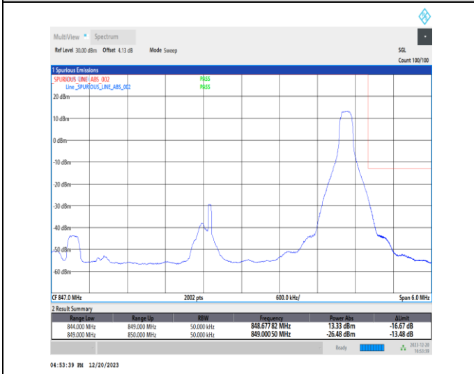
1-N515-5-H-5-CP-QPSK-Edge_1RB_Right-1@24-Ant1-1-seegraph-PASS-see graph
