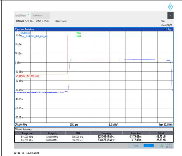
1-N5-PC3-15-20-L-6-CP-QPSK-Outer_Full-106 @0-Ant1-1-seegraph-PASS-see graph
