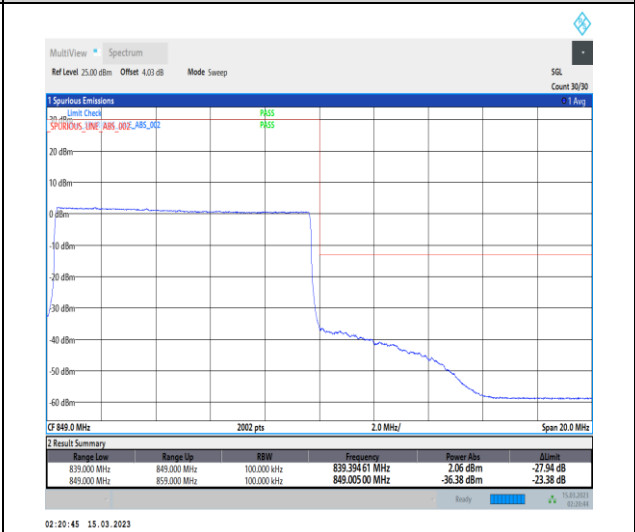
1-N5-PC3-15-10-H-6-CP-QPSK-Outer_Full-52@0-Ant1-1-seegraph-PASS-see graph
