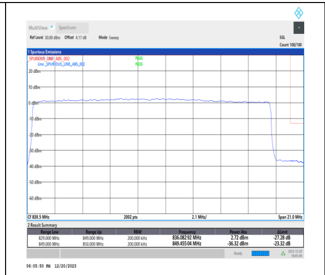
1-N515-20-H-3-DFT-PI2BPSK-Outer_Full-100@0- Ant1-1-seegraph-PASS-see graph
