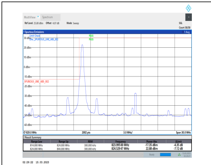
1-N5-PC3-15-20-L-1-DFT-PI2BPSK-Edge_1RB_Left-1 @0-Ant1-1-seegraph-PASS-see graph
