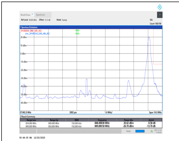
1-N515-15-H-2-DFT-PI2BPSK-Edge_1RB_Right-1@78-Ant1-1-seegraph-PASS-see graph
