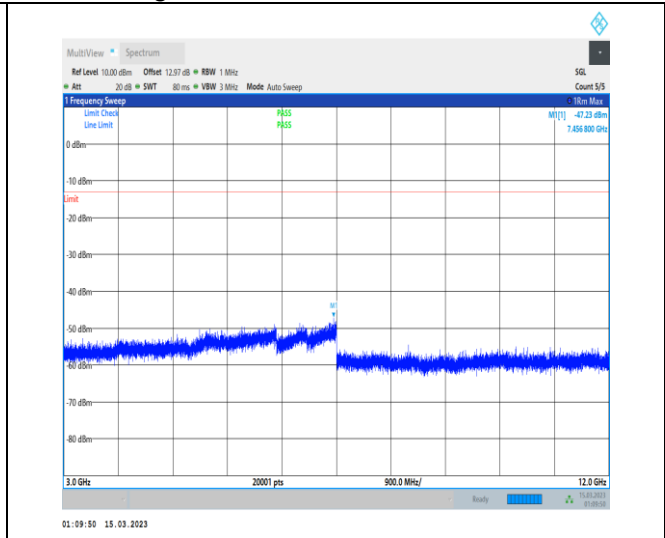
1-N5-PC3-15-20-M-1-DFT-PI2BPSK-Inner_1RB_Left -1@1-3000-12000-Ant1-7456.80--47.23--13-PASS
