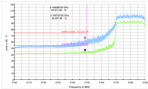
802.11ax HE20 -Channel 36: Peak + Average
