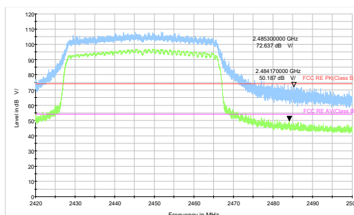
802.11ax HE40-Channel 8 Peak+ Average
