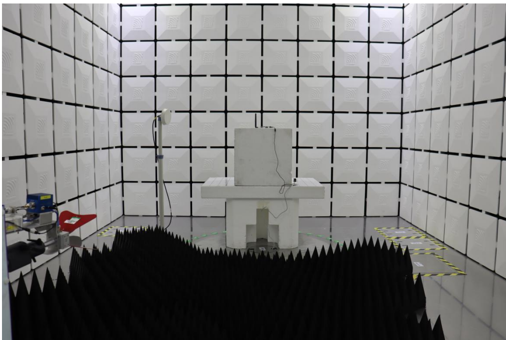
Above 1GHz
