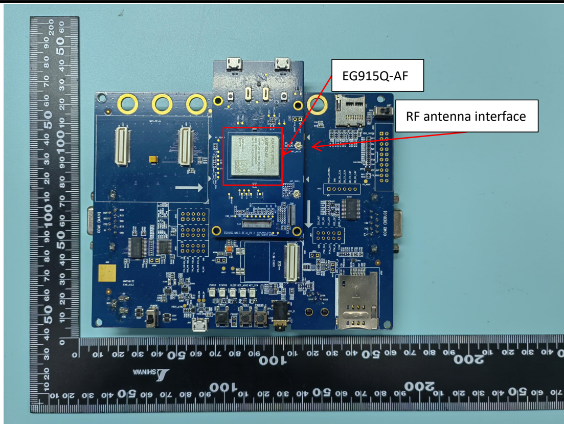
EG915Q-AF + EVB_Top
