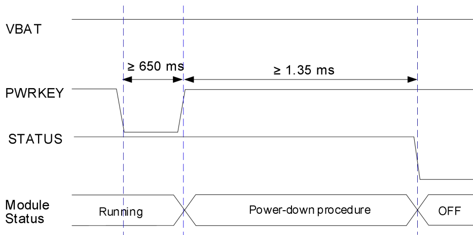
Figure 15: Power-down Timing with PWRKEY
