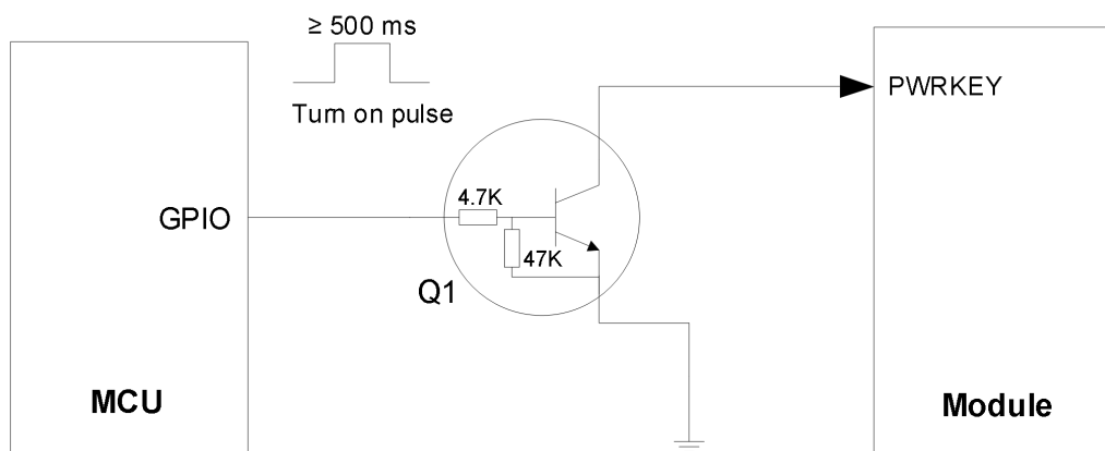
Figure 17: Reference Design of PWRKEY with Driving Circuit
