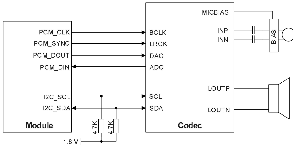
Figure 27: Reference Design of PCM and I2C Interfaces
