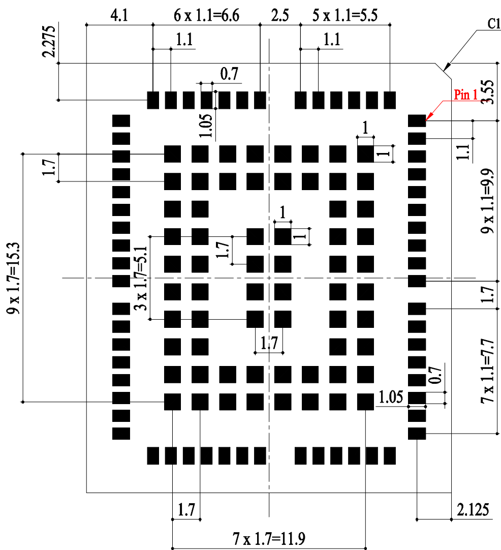
Figure 42: EG916Q-GL Bottom Dimension (Bottom View, Unit: mm)
