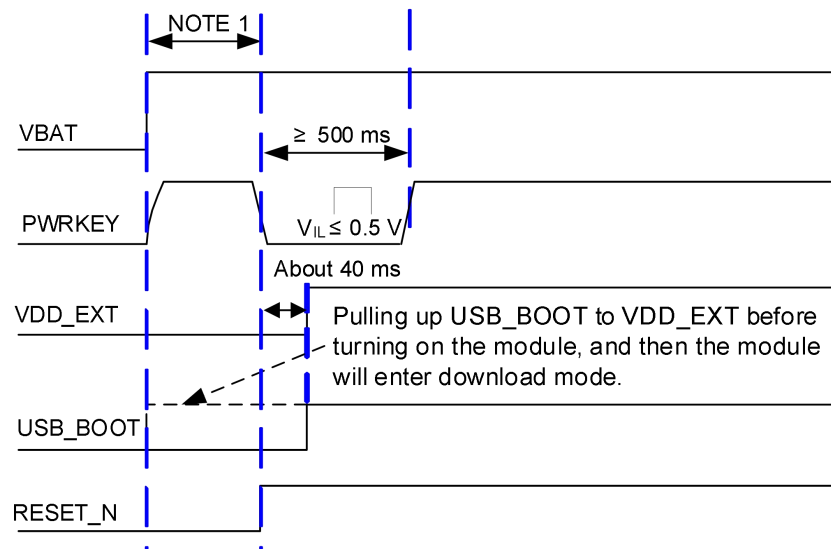
Figure 21: Timing of Entering Download Mode
