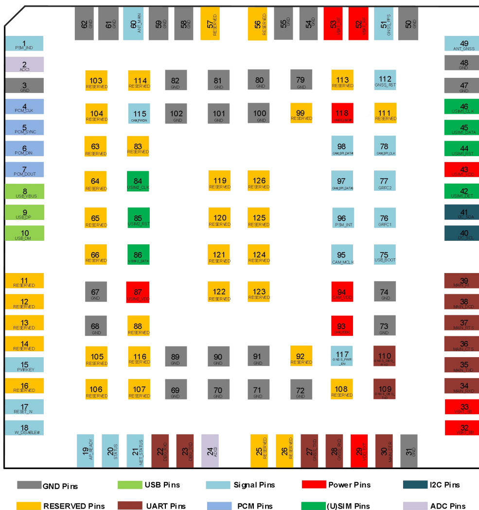
Figure 1: EG915Q Series Pin Assignment (Top View)
