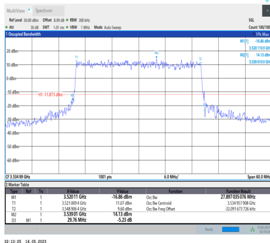
1-N78-3450-3550-PC1-30-30-H-7-CP-16QAM-Outer_Full-78@0-Ant0-27.897-29.760-≤30-PASS
