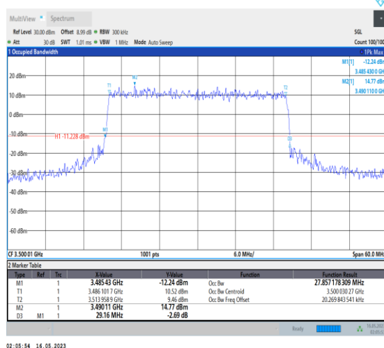
1-N78-3450-3550-PC1-30-30-M-6-CP-QPSK-Oute r_Full-78@0-Ant0-27.857-29.160-≤30-PASS
