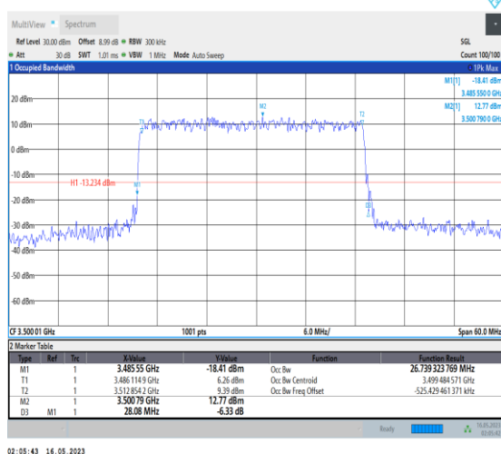
1-N78-3450-3550-PC1-30-30-M-5-DFT-256QAM-Ou ter_Full-75@0-Ant0-26.739-28.080-≤30-PASS
