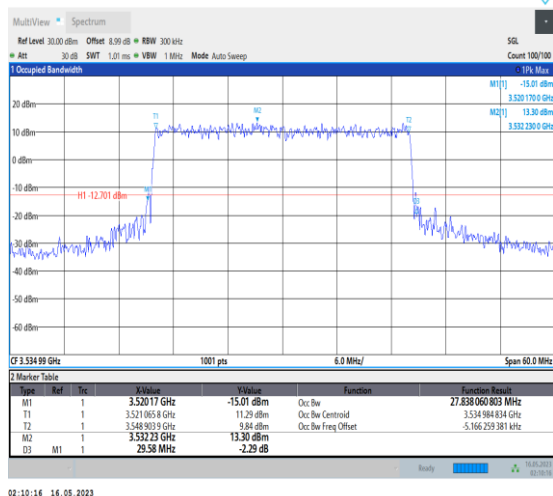
1-N78-3450-3550-PC1-30-30-H-6-CP-QPSK-Outer_Full-78@0-Ant0-27.838-29.580-≤30-PASS
