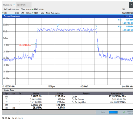
1-N78-3450-3550-PC1-30-30-M-3-DFT-16QAM-Out er_Full-75@0-Ant0-26.75-28.260-≤30-PASS
