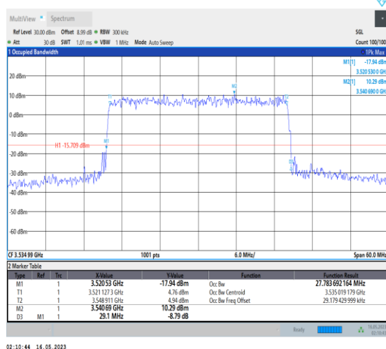
1-N78-3450-3550-PC1-30-30-H-9-CP-256QAM-Outer_Full-78@0-Ant0-27.784-29.100-≤30-PASS
