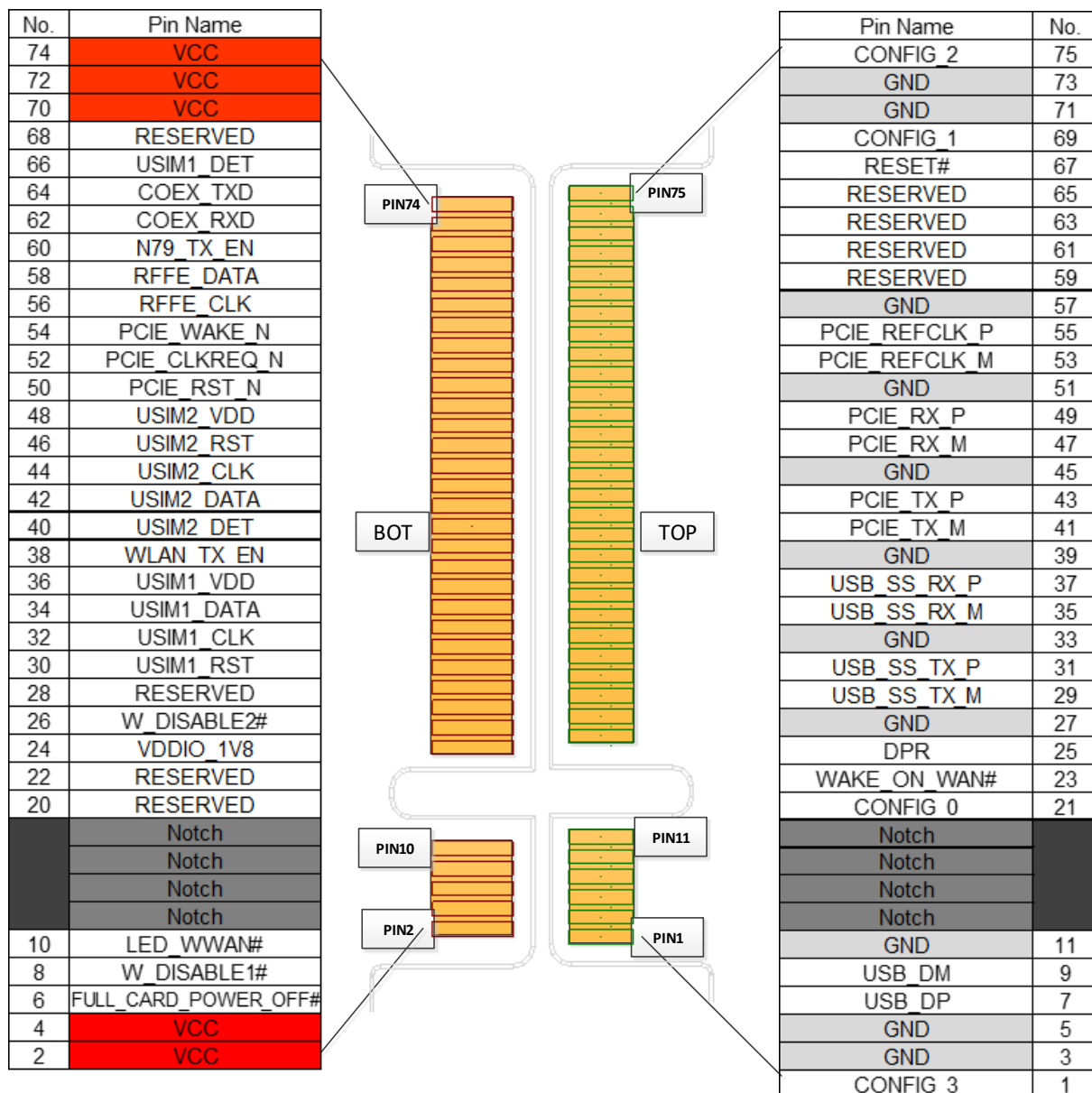
Figure 2: Pin Assignment
