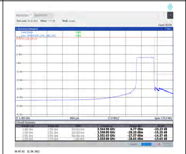
1-N78-3450-3550--30-20-H-6-CP-QPSK-Outer_Fu ll-51@0-Ant1-PASS-see graph
