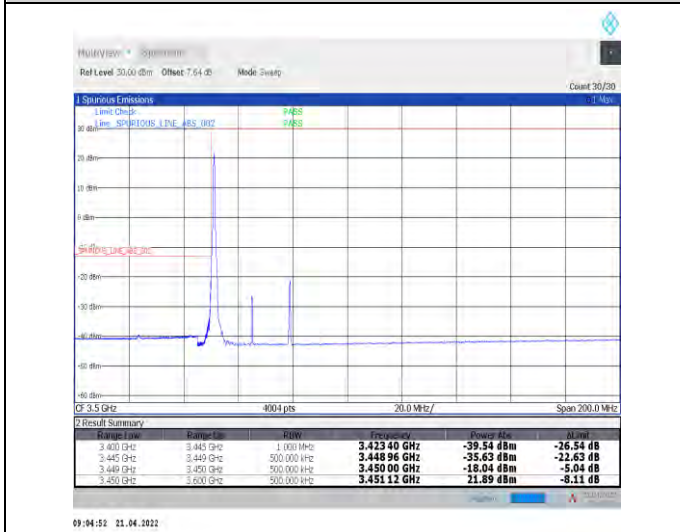
1-N78-3450-3550--30-30-L-4-CP-QPSK-Edge_1RB_L_eft-1@0-Ant1-PASS-see graph
