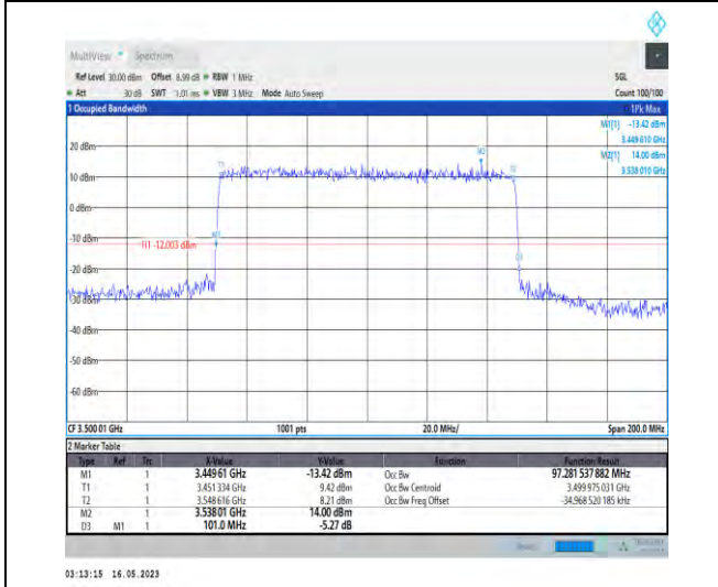
1-N78-3450-3550-PC1-30-100-H-7-CP-16QAM-Outer_Full-273@0-Ant1-97.282-101.000-≤100-PASS
