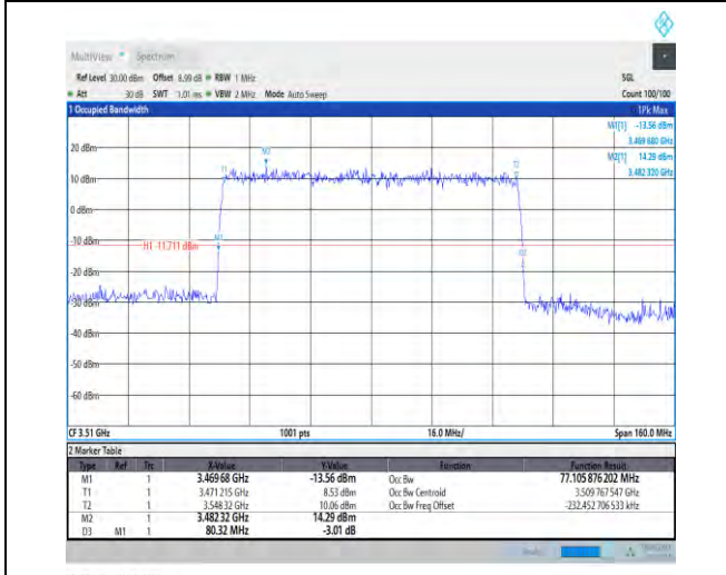
1-N78-3450-3550-PC1-30-80-H-5-DFT-256QAM-Outer_Full-216@0-Ant1-77.106-80.320-≤80-PASS
