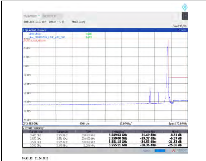
1-N78-3450-3550--30-20-H-2-DFT-PI2BPSK-Edge_1R_B_Right-1@50-Ant1-PASS-see graph
