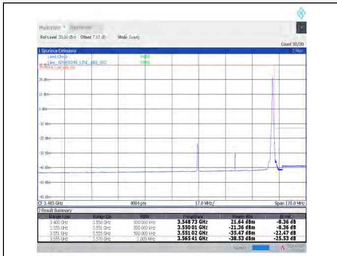
1-N78-3450-3550--30-50-H-2-DFT-PI2BPSK-Edge_1R_B_Right-1@132-Ant1-PASS-see graph
