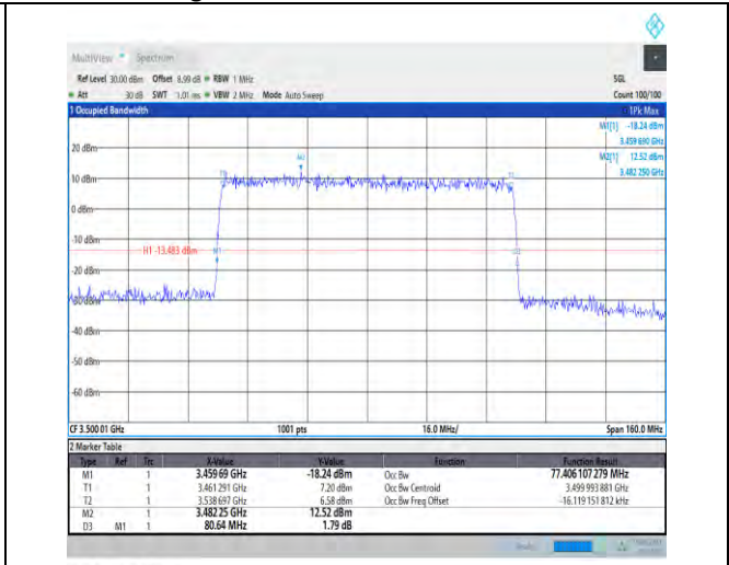
1-N78-3450-3550-PC1-30-80-M-9-CP-256QAM-Outer_Full-217@0-Ant1-77.406-80.640-≤80-PASS
