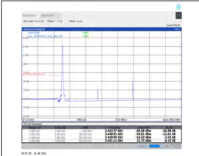
1-N78-3450-3550--30-90-L-1-DFT-PI2BPSK-Edge_1R_B_Left-1@0-Ant1-PASS-see graph
