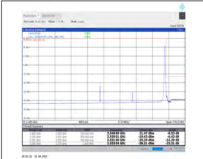
1-N78-3450-3550--30-70-H-2-DFT-PI2BPSK-Edge_1R_B_Right-1@188-Ant1-PASS-see graph
