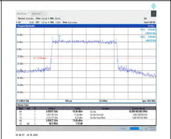
1-N78-3450-3550-PC1-30-70-L-3-DFT-16QAM-Outer_Full-180@0-Ant1-63.895-66.500-≤70-PASS
