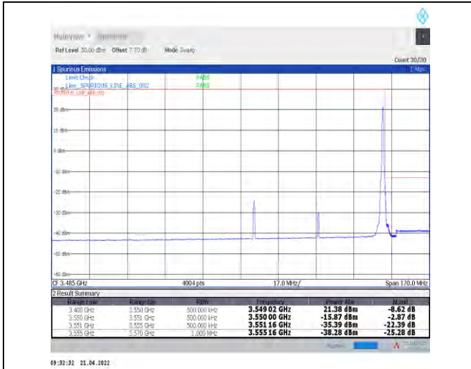
1-N78-3450-3550--30-60-H-2-DFT-PI2BPSK-Edge_1R_B_Right-1@161-Ant1-PASS-see graph
