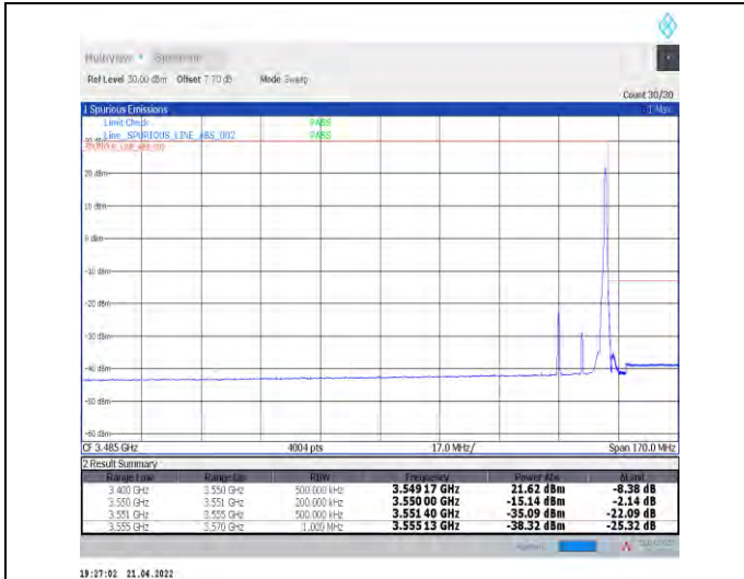
1-N78-3450-3550--30-15-H-2-DFT-PI2BPSK-Edge_1R_B_Right-1@37-Ant1-PASS-see graph
