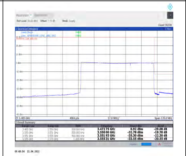
1-N78-3450-3550--30-80-H-6-CP-QPSK-Outer_Fu ll-217@0-Ant1-PASS-see graph
