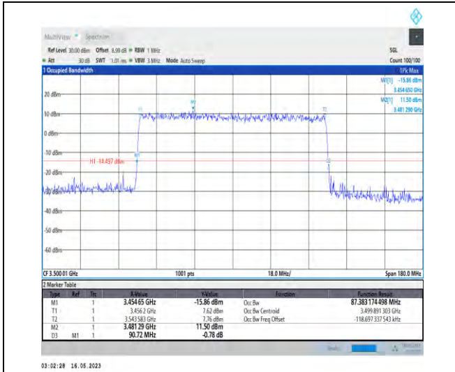
1-N78-3450-3550-PC1-30-90-M-9-CP-256QAM-Out er_Full-245@0-Ant1-87.383-90.720-≤90-PASS
