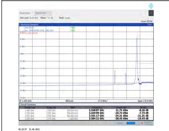
1-N78-3450-3550--30-30-H-5-CP-QPSK-Edge_1RB_Right-1@77-Ant1-PASS-see graph
