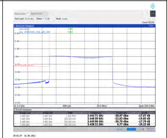
1-N78-3450-3550--30-90-L-6-CP-QPSK-Outer_Ful_I-245@0-Ant1-PASS-see graph
