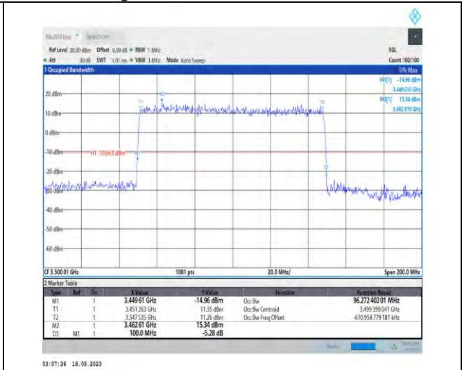
1-N78-3450-3550-PC1-30-100-L-4-DFT-64QAM-Out er_Full-270@0-Ant1-96.272-100.000-≤100-PASS
