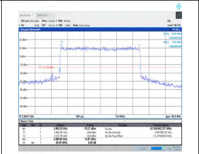
1-N78-3450-3550-PC1-30-70-M-6-CP-QPSK-Out_Full-189@0-Ant1-67.435-69.440-≤70-PASS
