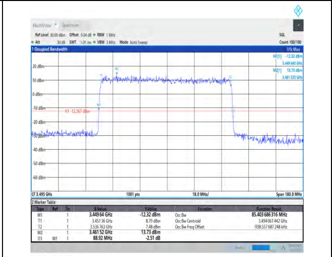
1-N78-3450-3550-PC1-30-90-L-3-DFT-16QAM-Outer_Full-240@0-Ant1-85.701-88.920-≤90-PASS
