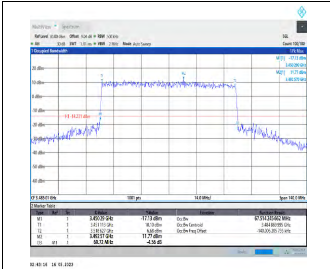
1-N78-3450-3550-PC1-30-70-L-8-CP-64QAM-Outer _Full-189@0-Ant1-67.514-69.720-≤70-PASS
