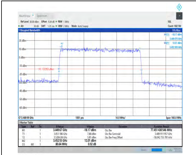
1-N78-3450-3550-PC1-30-80-L-9-CP-256QAM-Outer_Full-217@0-Ant1-77.451-80.640-≤80-PASS
