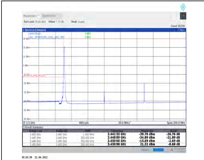
1-N78-3450-3550--30-100-L-1-DFT-PI2BPSK-Edge_1 RB_Left-1@0-Ant1-PASS-see graph
