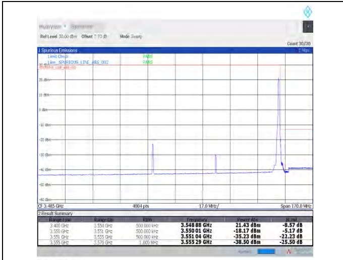
1-N78-3450-3550--30-80-H-2-DFT-PI2BPSK-Edge_1R_B_Right-1@216-Ant1-PASS-see graph
