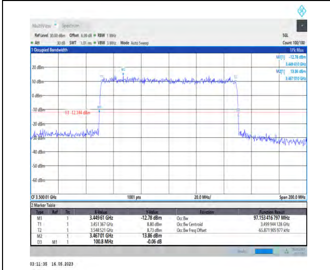
1-N78-3450-3550-PC1-30-100-M-8-CP-64QAM-Outer_Full-273@0-Ant1-97.153-100.800-≤100-PASS
