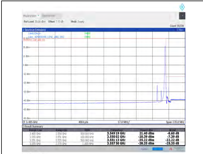
1-N78-3450-3550--30-10-H-2-DFT-PI2BPSK-Edge_1R_B_Right-1@23-Ant1-PASS-see graph
