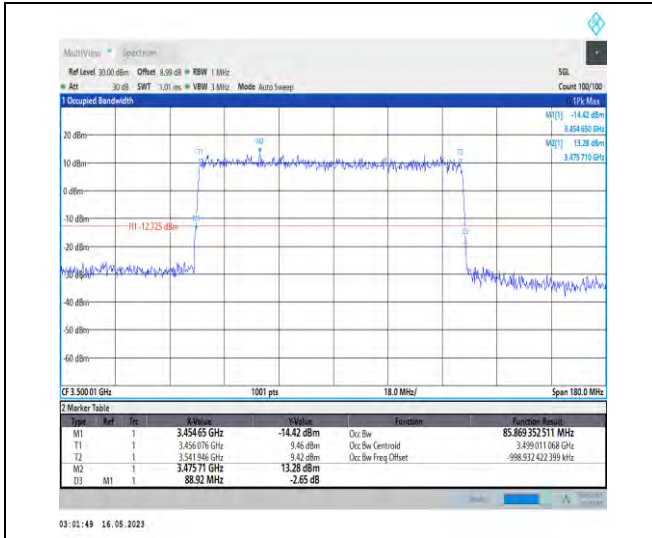
1-N78-3450-3550-PC1-30-90-M-5-DFT-256QAM-Outer_Full-240@0-Ant1-85.869-88.920-≤90-PASS
