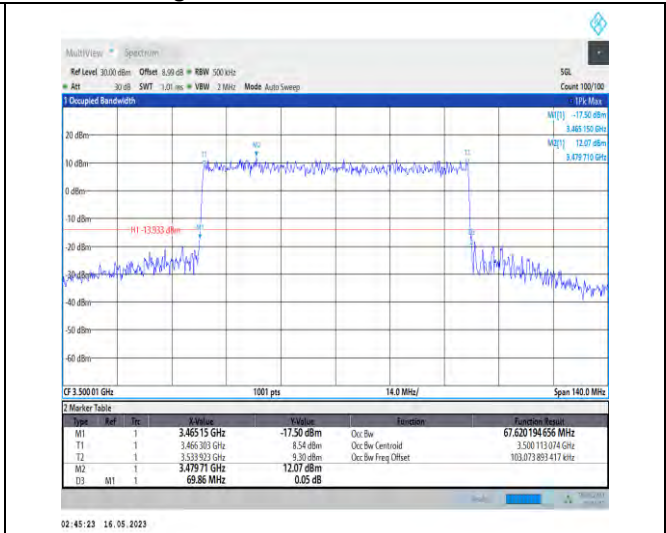
1-N78-3450-3550-PC1-30-70-M-8-CP-64QAM-Outer_Full-189@0-Ant1-67.62-69.860-≤70-PASS
