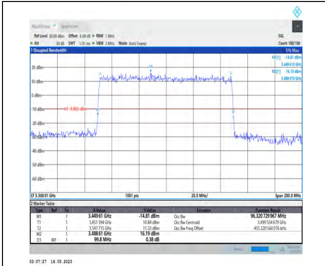
1-N78-3450-3550-PC1-30-100-L-3-DFT-16QAM-Out er_Full-270@0-Ant1-96.321-99.800-≤100-PASS
