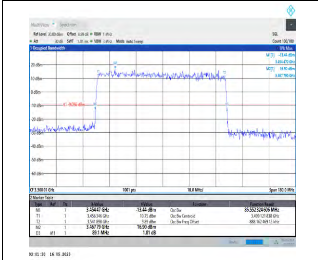
1-N78-3450-3550-PC1-30-90-M-3-DFT-16QAM-Outer_Full-240@0-Ant1-85.552-89.100-≤90-PASS
