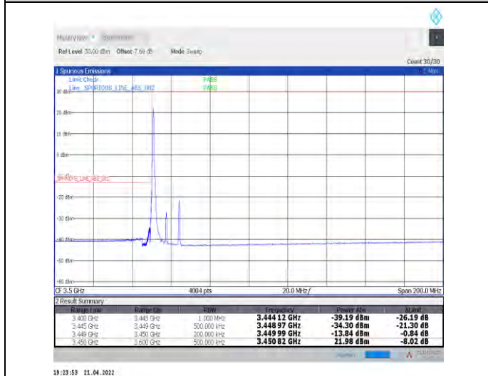
1-N78-3450-3550--30-15-L-4-CP-QPSK-Edge_1RB_L_eff-1@0-Ant1-PASS-see graph
