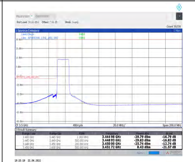
1-N78-3450-3550--30-15-L-6-CP-QPSK-Outer_Ful l-38@0-Ant1-PASS-see graph
