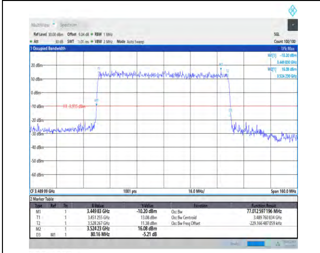
1-N78-3450-3550-PC1-30-80-L-1-DFT-QPSK-Outer_Full-216@0-Ant1-76.897-80.320-≤80-PASS
