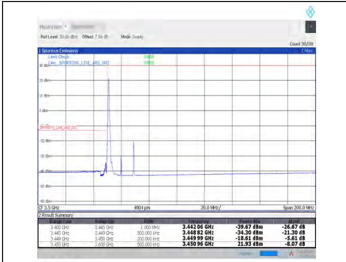
1-N78-3450-3550--30-20-L-1-DFT-PI2BPSK-Edge_1R_B_Left-1@0-Ant1-PASS-see graph
