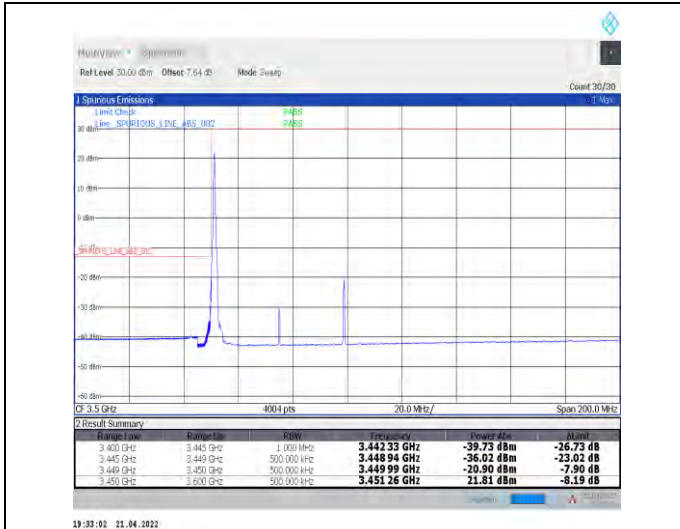
1-N78-3450-3550--30-50-L-1-DFT-PI2BPSK-Edge_1R_B_Left-1@0-Ant1-PASS-see graph
