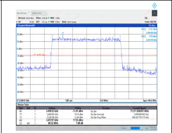
1-N78-3450-3550-PC1-30-80-M-1-DFT-QPSK-Outer_Full-216@0-Ant1-77.176-80.320-≤80-PASS
