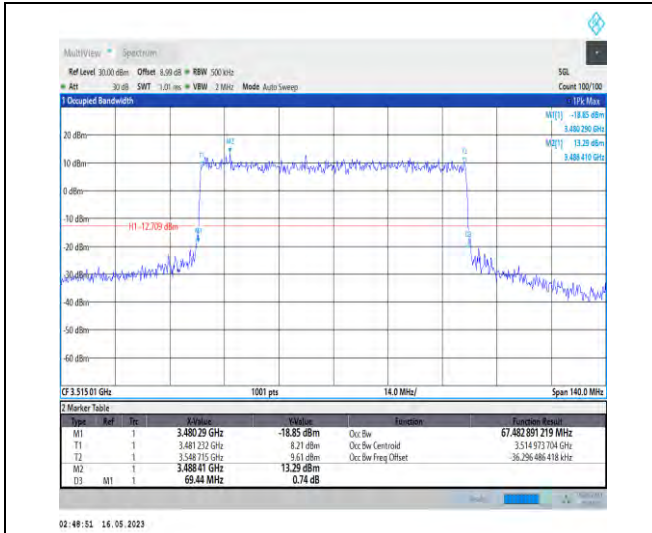
1-N78-3450-3550-PC1-30-70-H-6-CP-QPSK-Outer_Full-189@0-Ant1-67.483-69.440-≤70-PASS
