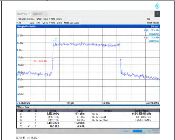
1-N78-3450-3550-PC1-30-70-L-5-DFT-256QAM-Outer_Full-180@0-Ant1-64.344-66.500-≤70-PASS
