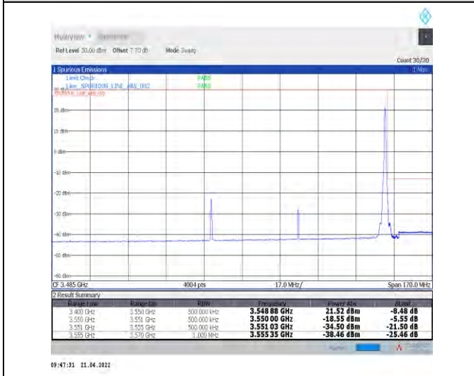
1-N78-3450-3550--30-80-H-5-CP-QPSK-Edge_1RB_R ight-1@216-Ant1-PASS-see graph
