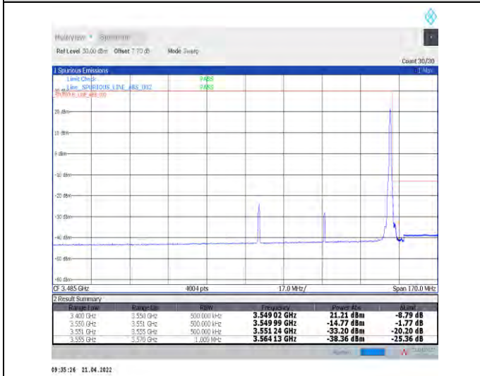
1-N78-3450-3550--30-60-H-5-CP-QPSK-Edge_1RB_R ight-1@161-Ant1-PASS-see graph
