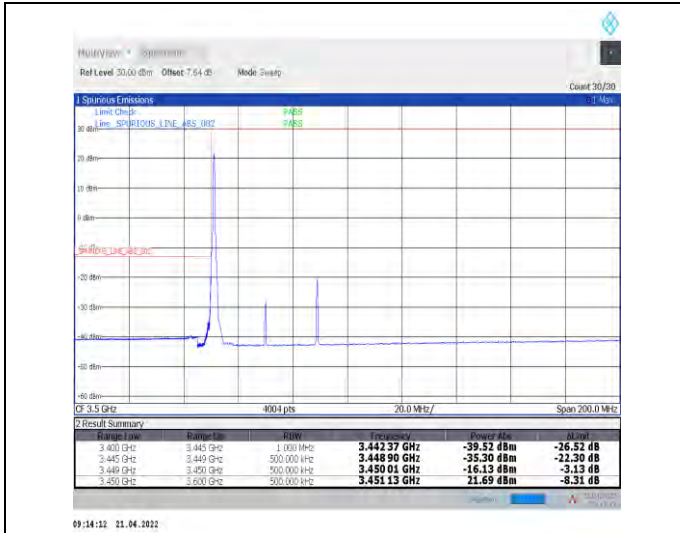
1-N78-3450-3550--30-40-L-1-DFT-PI2BPSK-Edge_1R_B_Left-1@0-Ant1-PASS-see graph
