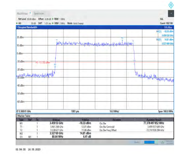
1-N78-3450-3550-PC1-30-80-M-7-CP-16QAM-Outer_Full-217@0-Ant1-77.378-80.640-≤80-PASS
