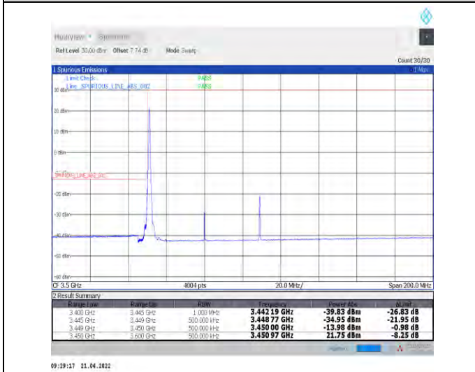
1-N78-3450-3550--30-60-L-4-CP-QPSK-Edge_1RB_L_eft-1@0-Ant1-PASS-see graph
