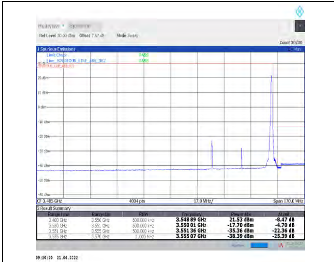
1-N78-3450-3550--30-40-H-2-DFT-PI2BPSK-Edge_1R_B_Right-1@105-Ant1-PASS-see graph
