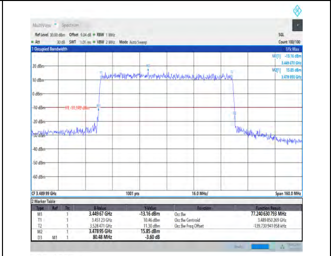
1-N78-3450-3550-PC1-30-80-L-2-DFT-PI2BPSK-Out_er_Full-216@0-Ant1-77.115-80.480-≤80-PASS
