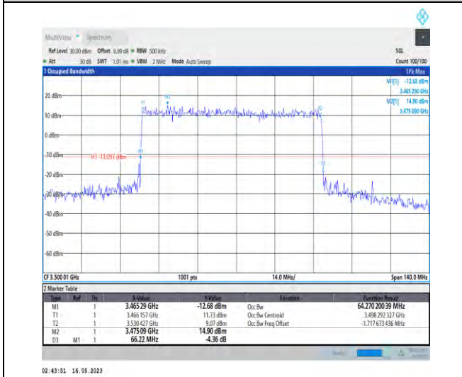
1-N78-3450-3550-PC1-30-70-M-1-DFT-QPSK-Outer _Full-180@0-Ant1-64.27-66.220-≤70-PASS
