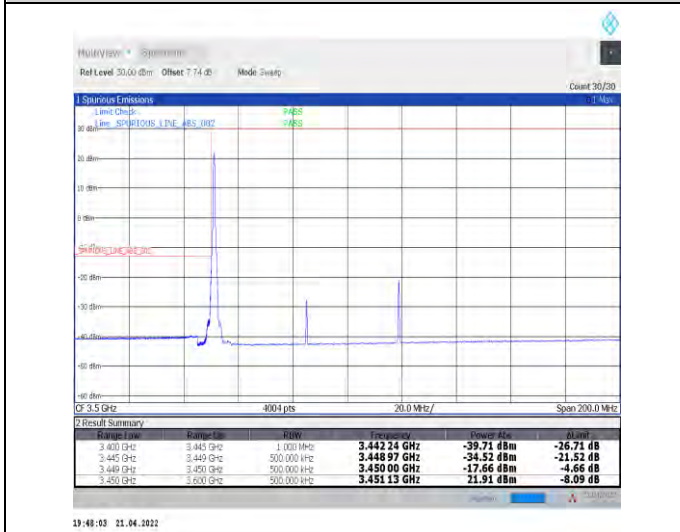
1-N78-3450-3550--30-70-L-4-CP-QPSK-Edge_1RB_L_eft-1@0-Ant1-PASS-see graph
