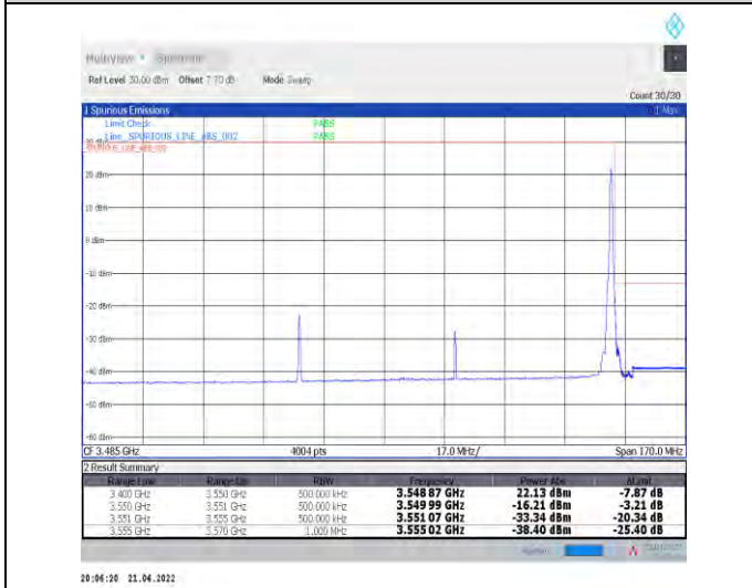
1-N78-3450-3550--30-90-H-5-CP-QPSK-Edge_1RB_R ight-1@244-Ant1-PASS-see graph
