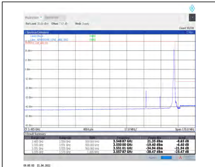
1-N78-3450-3550--30-30-H-2-DFT-PI2BPSK-Edge_1R_B_Right-1@77-Ant1-PASS-see graph
