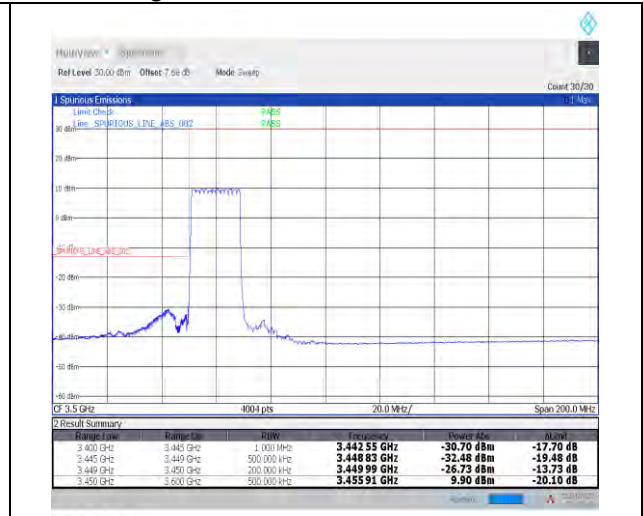
1-N78-3450-3550--30-20-L-3-DFT-PI2BPSK-Outer_Full-50@0-Ant1-PASS-see graph
