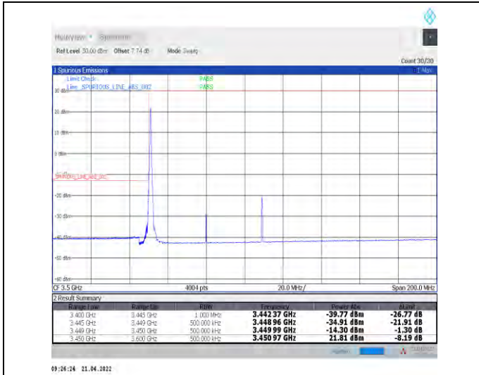
1-N78-3450-3550--30-60-L-1-DFT-PI2BPSK-Edge_1R_B_Left-1@0-Ant1-PASS-see graph
