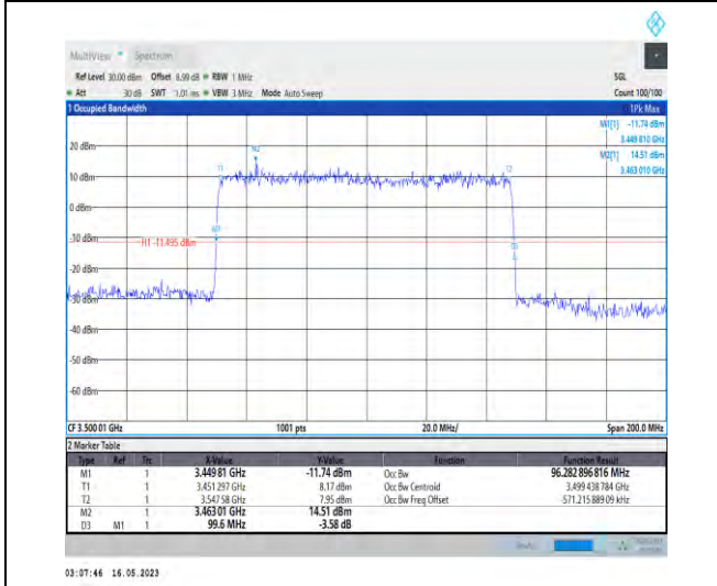
1-N78-3450-3550-PC1-30-100-L-5-DFT-256QAM-Out uter_Full-270@0-Ant1-96.283-99.600-≤100-PASS
