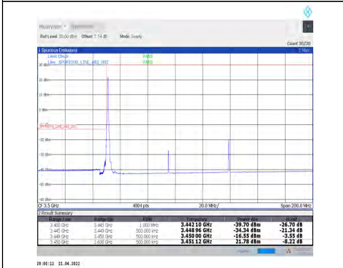
1-N78-3450-3550--30-90-L-4-CP-QPSK-Edge_1RB_L_eft-1@0-Ant1-PASS-see graph
