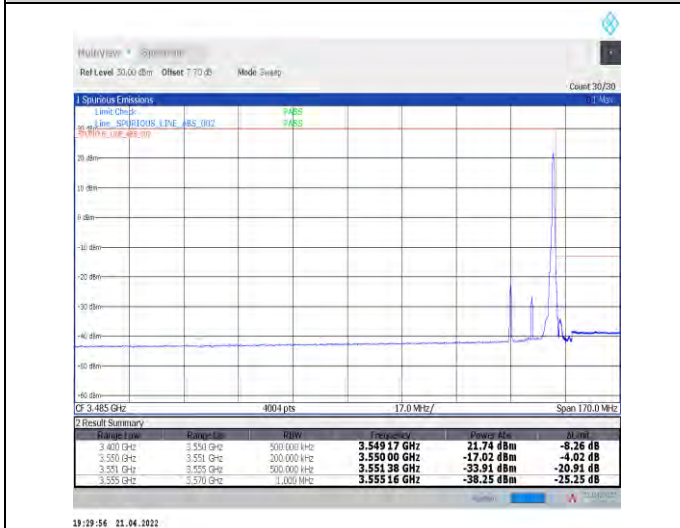
1-N78-3450-3550--30-15-H-5-CP-QPSK-Edge_1RB_R ight-1@37-Ant1-PASS-see graph
