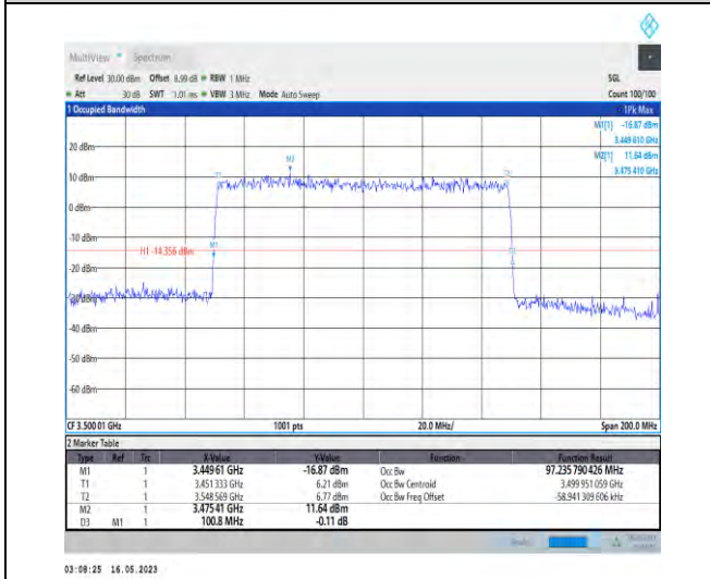
1-N78-3450-3550-PC1-30-100-L-9-CP-256QAM-Outer_Full-273@0-Ant1-97.236-100.800-≤100-PASS
