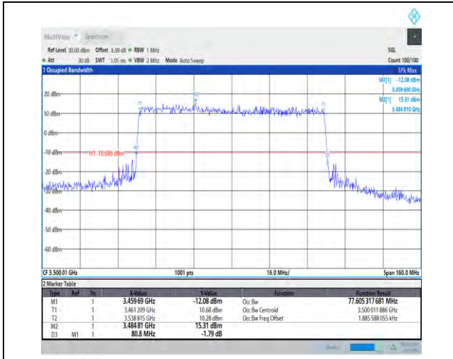
1-N78-3450-3550-PC1-30-80-M-8-CP-64QAM-Outer_Full-217@0-Ant1-77.605-80.800-≤80-PASS
