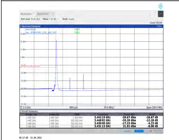
1-N78-3450-3550--30-40-L-4-CP-QPSK-Edge_1RB_L eft-1@0-Ant1-PASS-see graph
