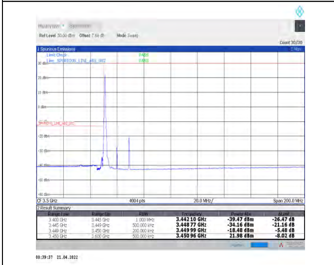
1-N78-3450-3550--30-20-L-4-CP-QPSK-Edge_1RB_L_eft-1@0-Ant1-PASS-see graph
