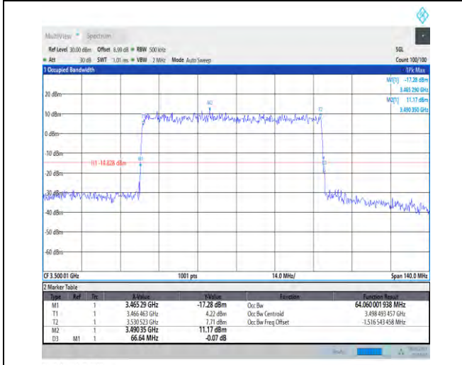
1-N78-3450-3550-PC1-30-70-M-5-DFT-256QAM-Out_Full-180@0-Ant1-64.06-66.640-≤70-PASS
