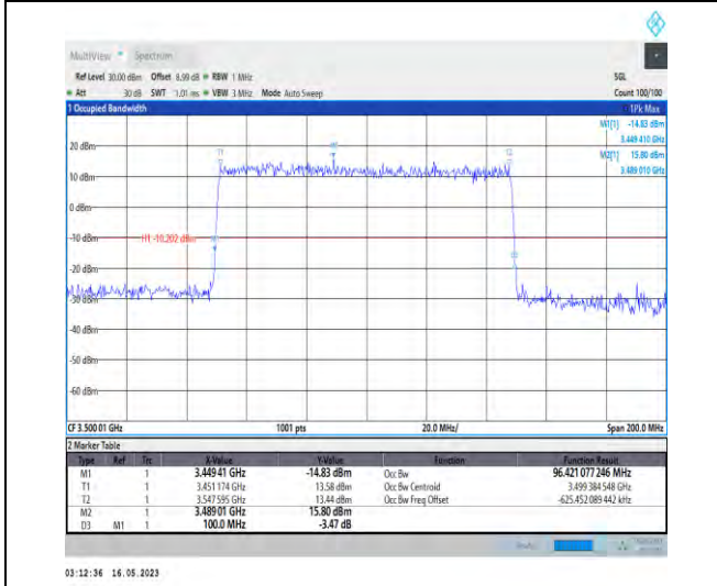
1-N78-3450-3550-PC1-30-100-H-3-DFT-16QAM-Outer_Full-270@0-Ant1-96.421-100.000-≤100-PASS
