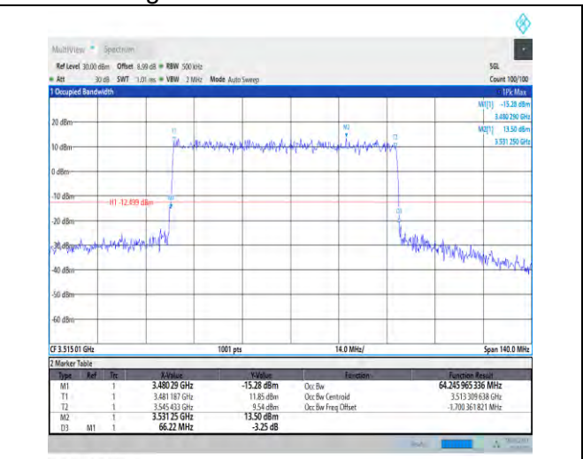
1-N78-3450-3550-PC1-30-70-H-3-DFT-16QAM-Outer_Full-180@0-Ant1-64.246-66.220-≤70-PASS
