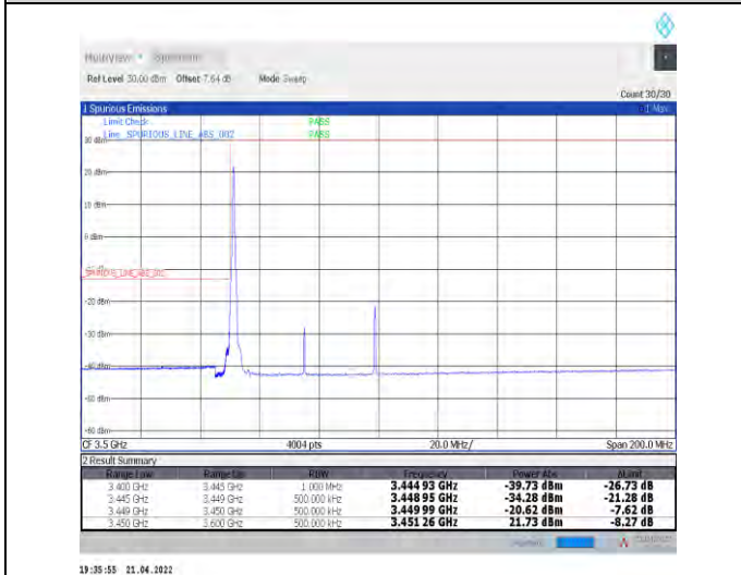
1-N78-3450-3550--30-50-L-4-CP-QPSK-Edge_1RB_L eft-1@0-Ant1-PASS-see graph
