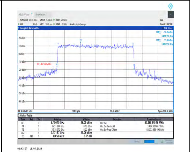
1-N78-3450-3550-PC1-30-70-L-7-CP-16QAM-Outer_Full-189@0-Ant1-67.288-69.580-≤70-PASS
