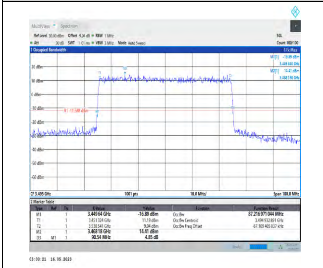
1-N78-3450-3550-PC1-30-90-L-8-CP-64QAM-Outer_Full-245@0-Ant1-87.217-90.540-<math>\leq 90</math>-PASS
