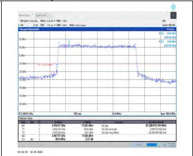
1-N78-3450-3550-PC1-30-90-M-6-CP-QPSK-Outer_Full-245@0-Ant1-87.29-90.900-≤90-PASS
