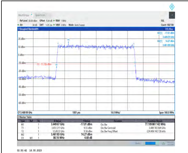
1-N78-3450-3550-PC1-30-80-L-5-DFT-256QAM-Out_er_Full-216@0-Ant1-77.11-80.160-<math>\leq 80</math>-PASS
