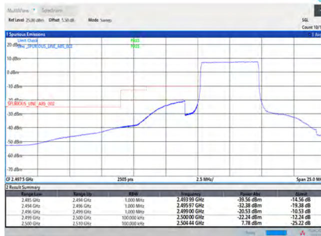
Band7-5MHz-QPSK-20775-25RB#0
