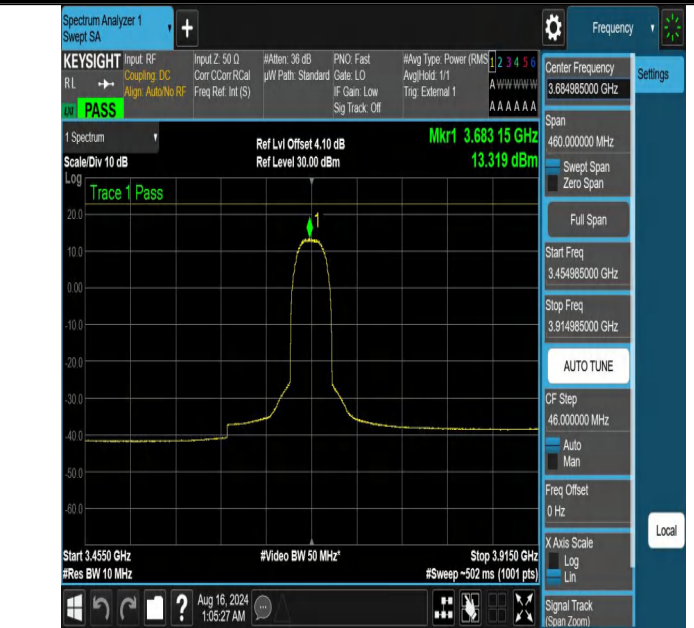
NTNV-DC_13A_n48A-PC3-30-5+30-M+H-N/A-N/A-DFT-256QAM-Outer_Full-3454.985-3914.985-PASS
