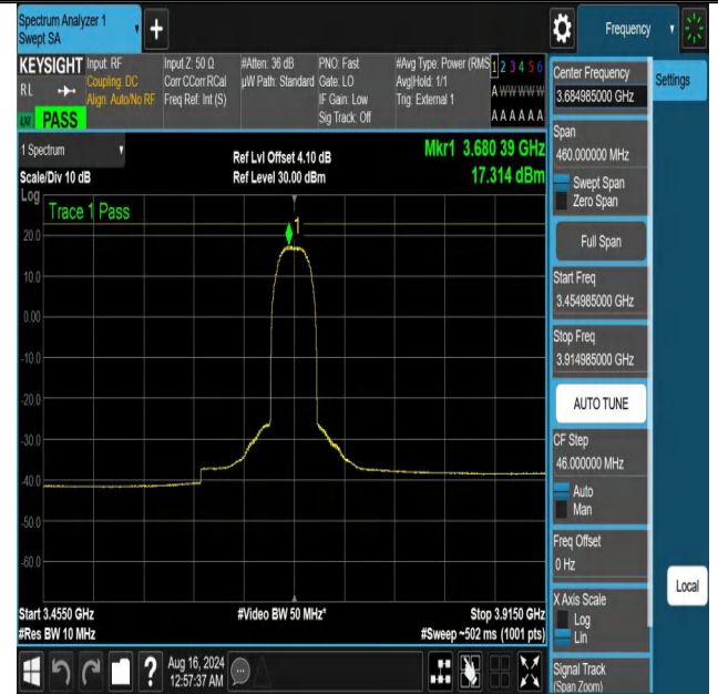
NTNV-DC_13A_n48A-PC3-30-5+30-M+H-N/A-N/A-DFT-PI2BPSK-O uter_Full-3454.985-3914.985-PASS
