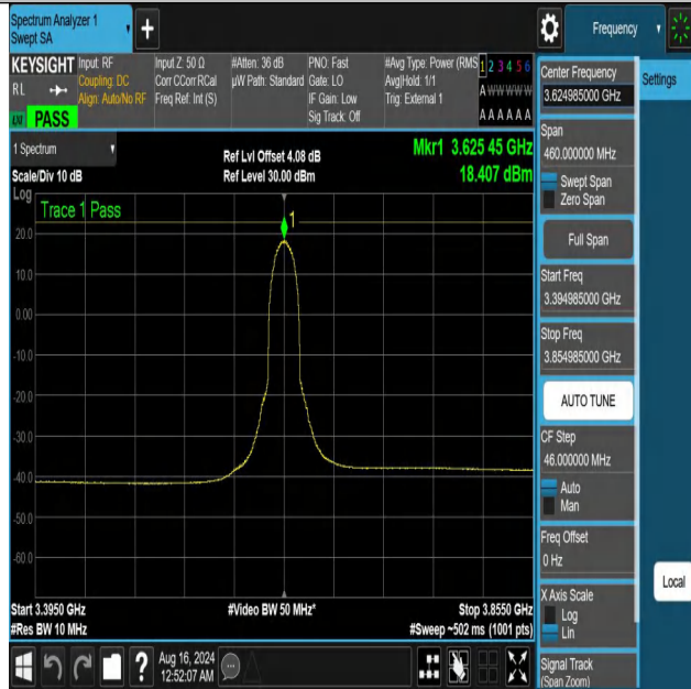
NTNV-DC_13A_n48A-PC3-30-5+30-M+M-N/A-N/A-CP-16QAM-Inner_Full-3394.985-3854.985-PASS
