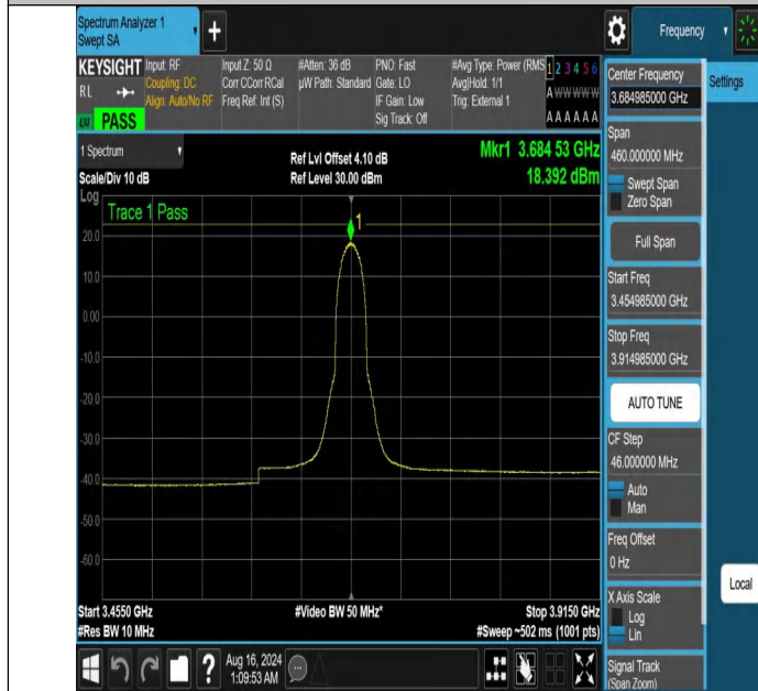
NTNV-DC_13A_n48A-PC3-30-5+30-M+H-N/A-N/A-CP-16QAM-Inner_Full-3454.985-3914.985-PASS
