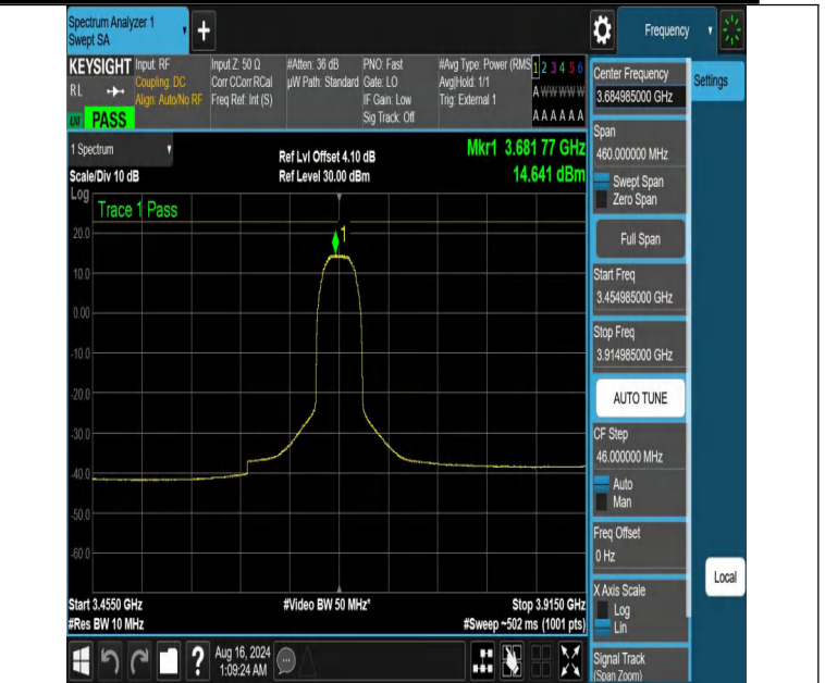
NTNV-DC_13A_n48A-PC3-30-5+30-M+H-N/A-N/A-CP-16QAM-Outer_Full-3454.985-3914.985-PASS
