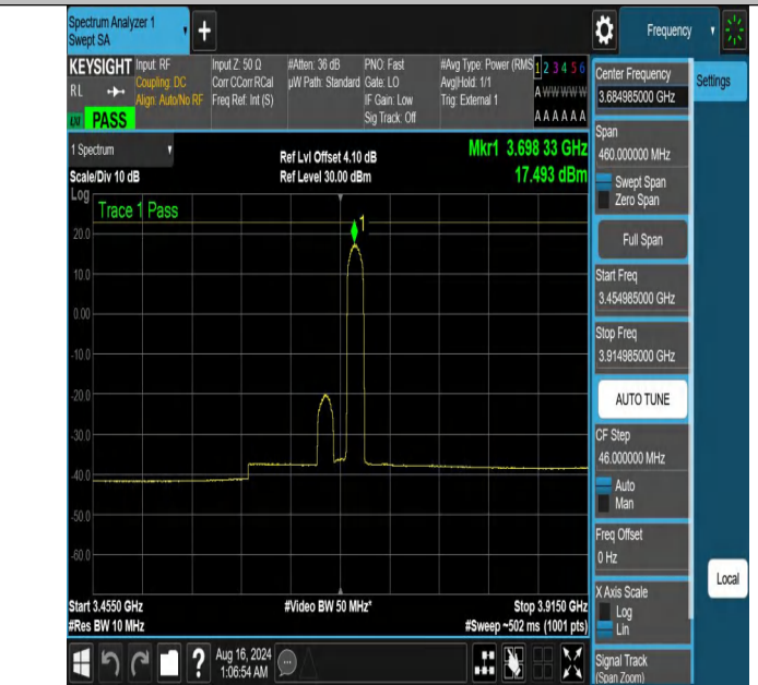
NTNV-DC_13A_n48A-PC3-30-5+30-M+H-N/A-N/A-DFT-256QAM-Edge_1RB_Right-3454.985-3914.985-PASS
