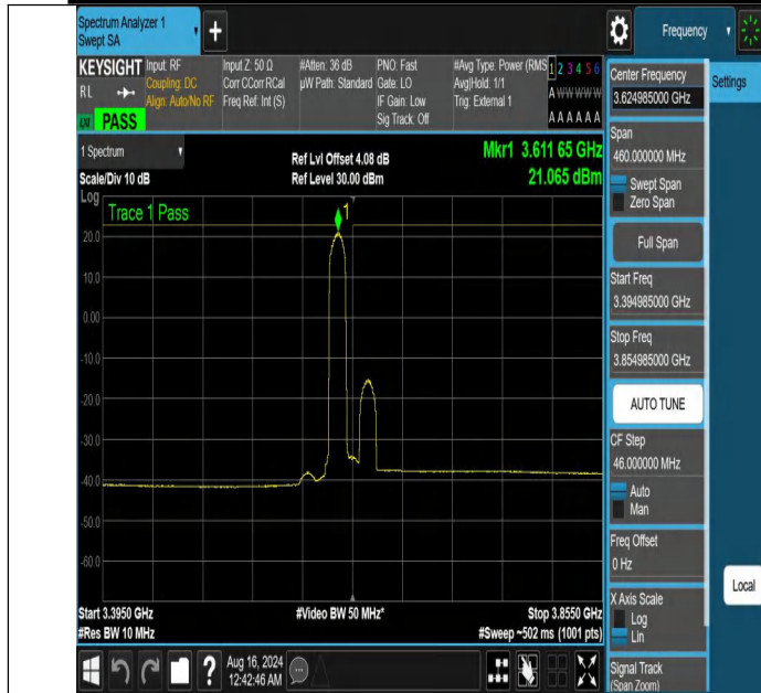
NTNV-DC_13A_n48A-PC3-30-5+30-M+M-N/A-N/A-DFT-QPSK-Ed ge_1RB_Left-3394.985-3854.985-PASS
