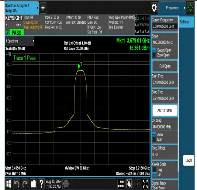
NTNV-DC_13A_n48A-PC3-30-5+30-M+H-N/A-N/A-DFT-64QAM-Ou ter_Full-3454.985-3914.985-PASS
