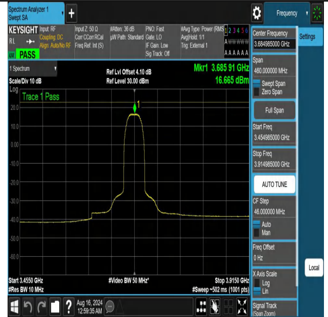
NTNV-DC_13A_n48A-PC3-30-5+30-M+H-N/A-N/A-DFT-QPSK-Oute r_Full-3454.985-3914.985-PASS
