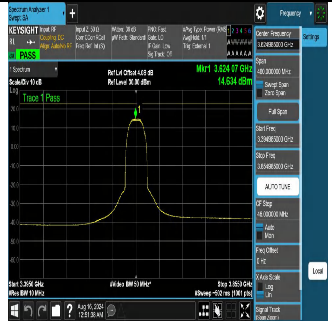
NTNV-DC_13A_n48A-PC3-30-5+30-M+M-N/A-N/A-CP-16QAM-Outer_Full-3394.985-3854.985-PASS
