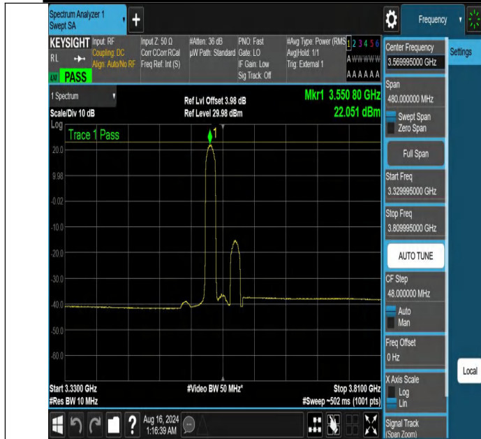
NTNV-DC_13A_n48A-PC3-30-5+40-M+L-N/A-N/A-DFT-PI2BPSK- Edge_1RB_Left-3329.995-3809.995-PASS
