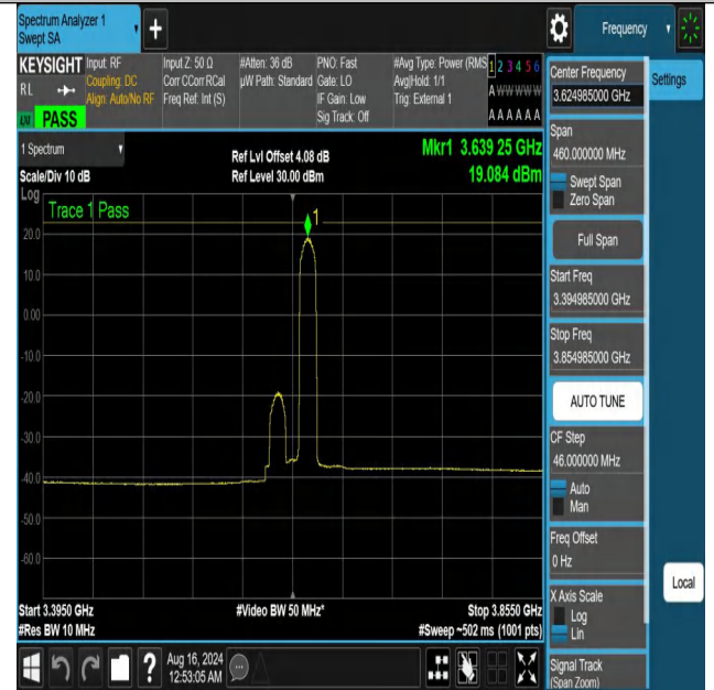
NTNV-DC_13A_n48A-PC3-30-5+30-M+M-N/A-N/A-CP-16QAM-Edge_1RB_Right-3394.985-3854.985-PASS
