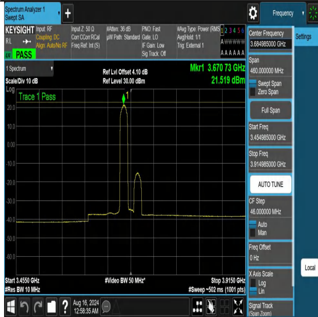
NTNV-DC_13A_n48A-PC3-30-5+30-M+H-N/A-N/A-DFT-PI2BPSK- Edge_1RB_Left-3454.985-3914.985-PASS
