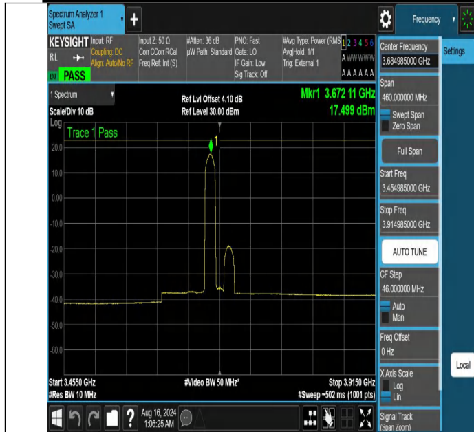
NTNV-DC_13A_n48A-PC3-30-5+30-M+H-N/A-N/A-DFT-256QAM-Edge_1RB_Left-3454.985-3914.985-PASS
