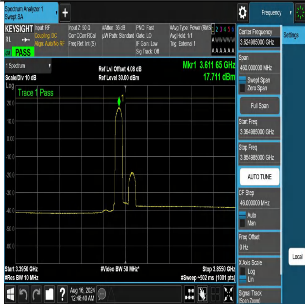
NTNV-DC_13A_n48A-PC3-30-5+30-M+M-N/A-N/A-DFT-256QAM-Edge_1RB_Left-3394.985-3854.985-PASS
