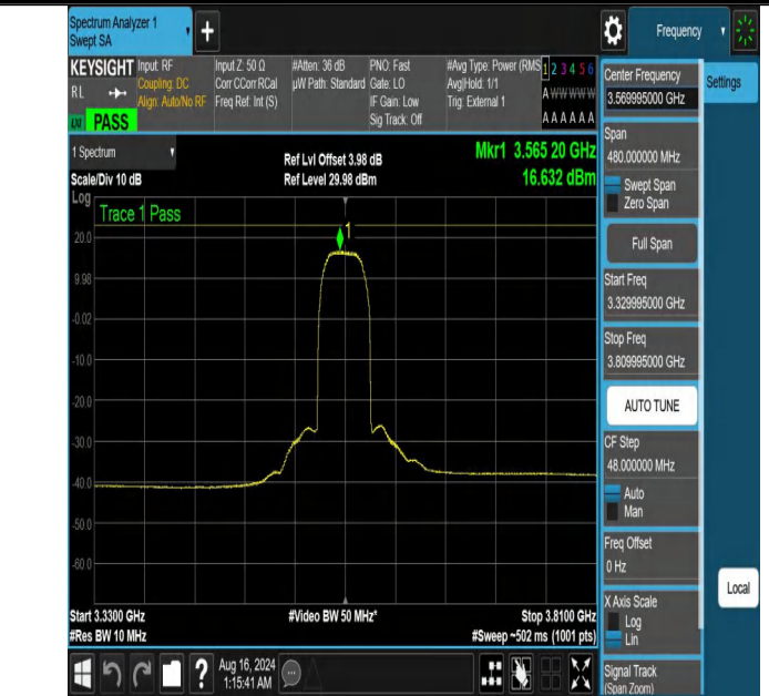
NTNV-DC_13A_n48A-PC3-30-5+40-M+L-N/A-N/A-DFT-PI2BPSK-O uter_Full-3329.995-3809.995-PASS
