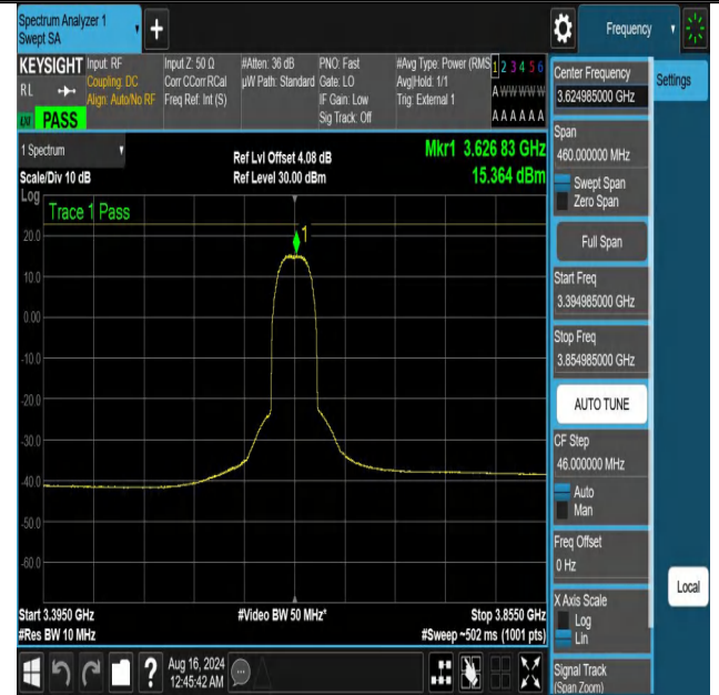
NTNV-DC_13A_n48A-PC3-30-5+30-M+M-N/A-N/A-DFT-64QAM-Ou ter_Full-3394.985-3854.985-PASS
