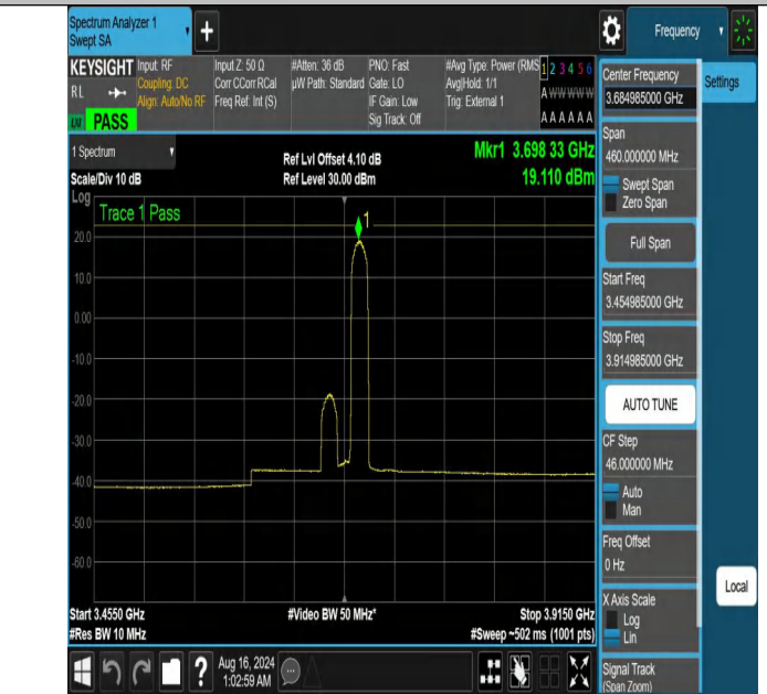
NTNV-DC_13A_n48A-PC3-30-5+30-M+H-N/A-N/A-DFT-16QAM-Ed ge_1RB_Right-3454.985-3914.985-PASS
