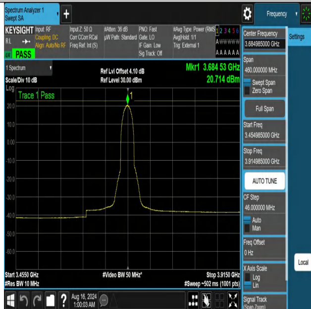
NTNV-DC_13A_n48A-PC3-30-5+30-M+H-N/A-N/A-DFT-QPSK-Inn er_Full-3454.985-3914.985-PASS
