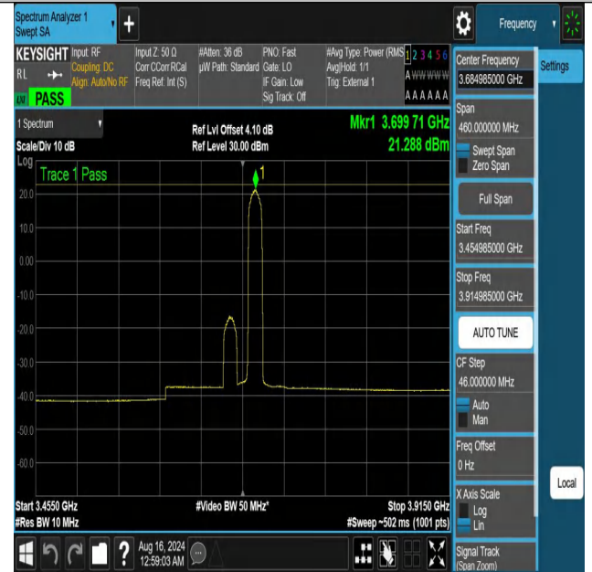
NTNV-DC_13A_n48A-PC3-30-5+30-M+H-N/A-N/A-DFT-PI2BPSK-E dge_1RB_Right-3454.985-3914.985-PASS
