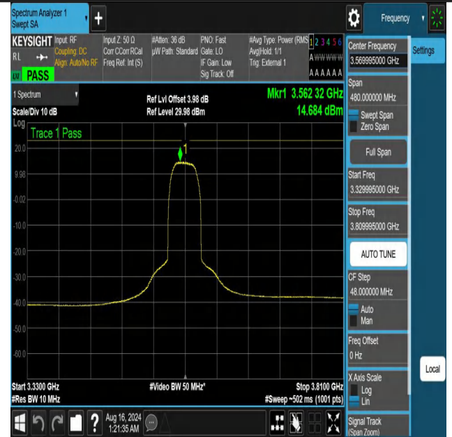
NTNV-DC_13A_n48A-PC3-30-5+40-M+L-N/A-N/A-DFT-64QAM-Out er_Full-3329.995-3809.995-PASS
