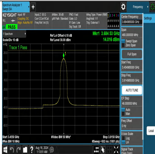
NTNV-DC_13A_n48A-PC3-30-5+30-M+H-N/A-N/A-CP-256QAM-In ner_Full-3454.985-3914.985-PASS
