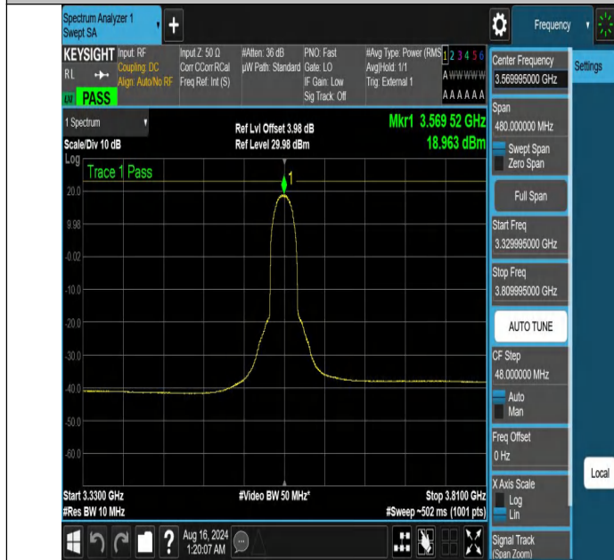
NTNV-DC_13A_n48A-PC3-30-5+40-M+L-N/A-N/A-DFT-16QAM-In ner_Full-3329.995-3809.995-PASS
