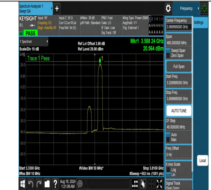
NTNV-DC_13A_n48A-PC3-30-5+40-M+L-N/A-N/A-DFT-16QAM-Ed ge_1RB_Right-3329.995-3809.995-PASS
