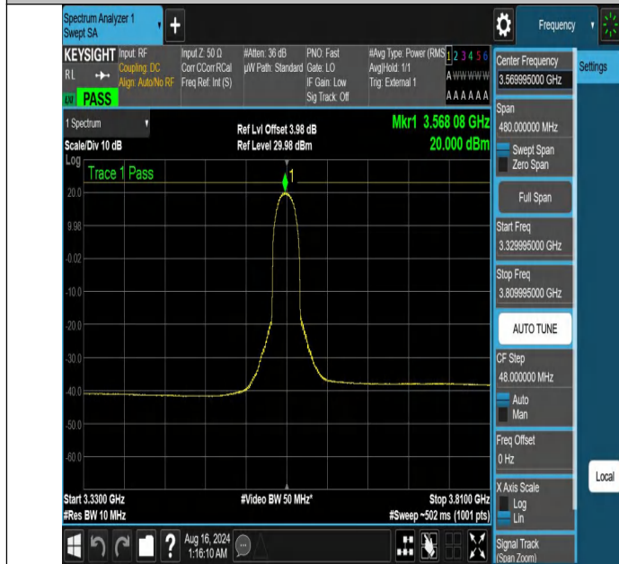
NTNV-DC_13A_n48A-PC3-30-5+40-M+L-N/A-N/A-DFT-PI2BPSK-I nner_Full-3329.995-3809.995-PASS
