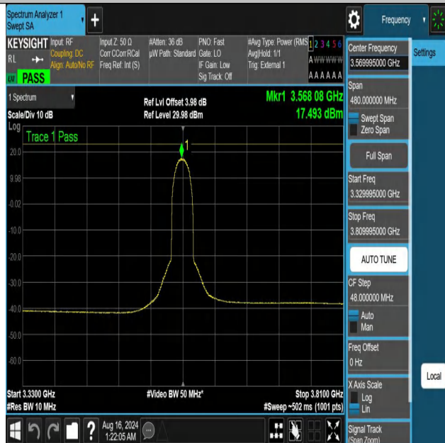
NTNV-DC_13A_n48A-PC3-30-5+40-M+L-N/A-N/A-DFT-64QAM-In ner_Full-3329.995-3809.995-PASS
