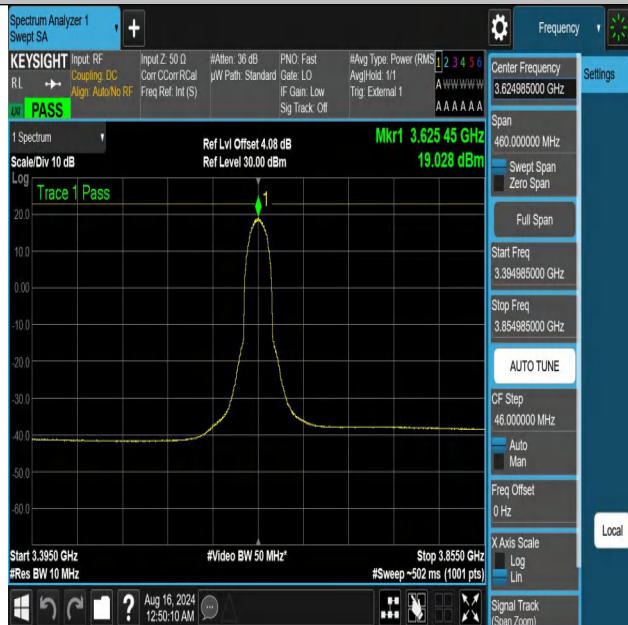
NTNV-DC_13A_n48A-PC3-30-5+30-M+M-N/A-N/A-CP-QPSK-Inne r_Full-3394.985-3854.985-PASS
