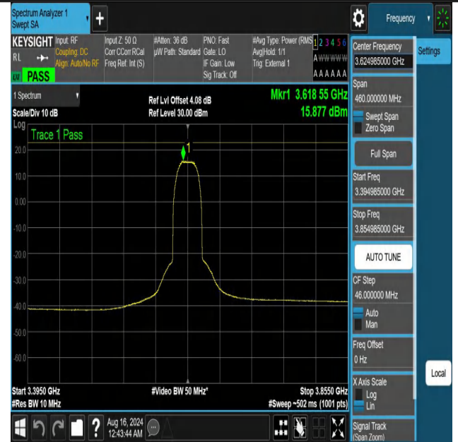
NTNV-DC_13A_n48A-PC3-30-5+30-M+M-N/A-N/A-DFT-16QAM-Ou ter_Full-3394.985-3854.985-PASS
