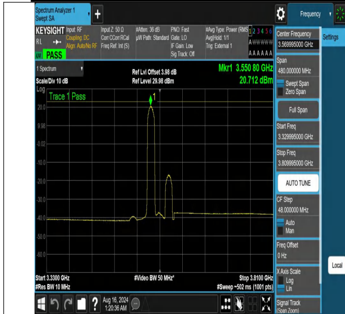
NTNV-DC_13A_n48A-PC3-30-5+40-M+L-N/A-N/A-DFT-16QAM-Ed ge_1RB_Left-3329.995-3809.995-PASS
