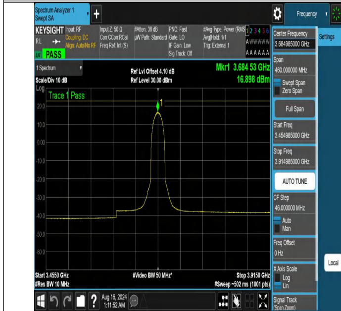
NTNV-DC_13A_n48A-PC3-30-5+30-M+H-N/A-N/A-CP-64QAM-Inner_Full-3454.985-3914.985-PASS
