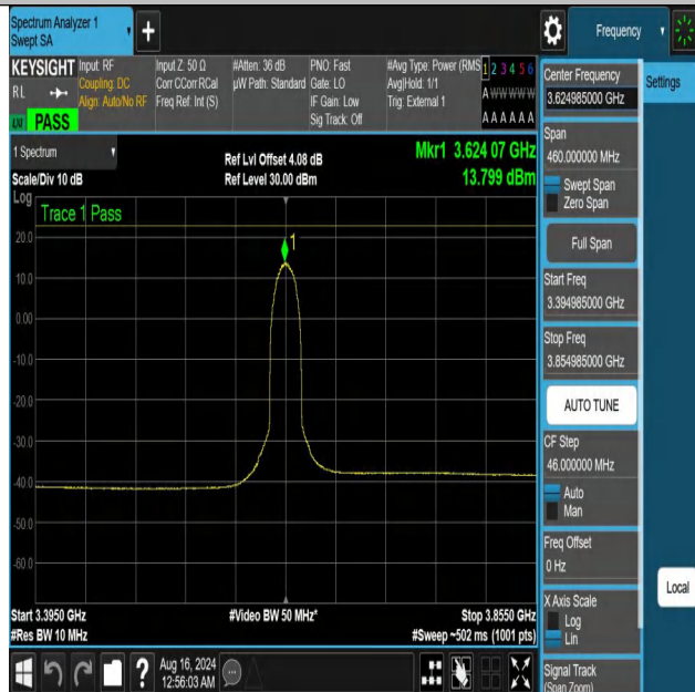
NTNV-DC_13A_n48A-PC3-30-5+30-M+M-N/A-N/A-CP-256QAM-In ner_Full-3394.985-3854.985-PASS
