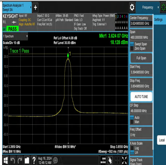
NTNV-DC_13A_n48A-PC3-30-5+30-M+M-N/A-N/A-DFT-64QAM-In ner_Full-3394.985-3854.985-PASS
