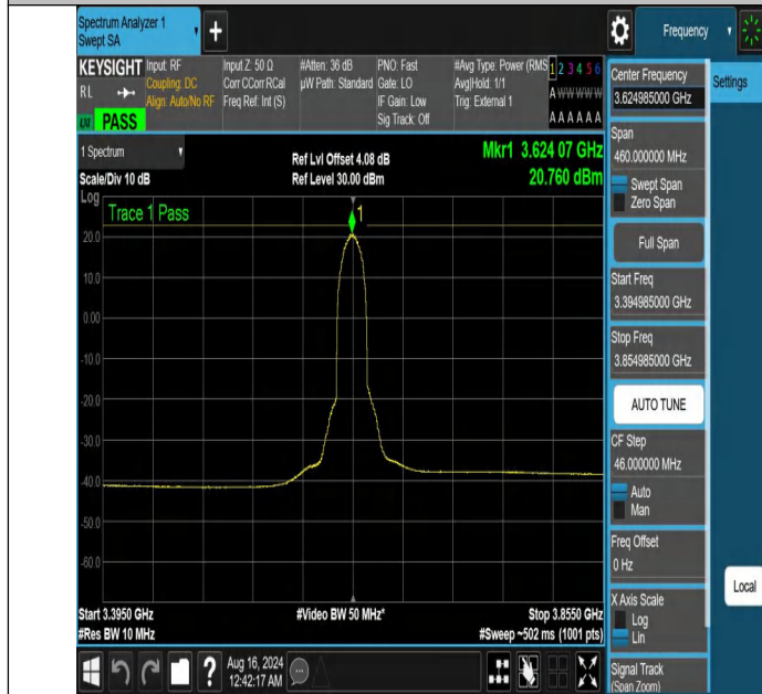
NTNV-DC_13A_n48A-PC3-30-5+30-M+M-N/A-N/A-DFT-QPSK-Inn er_Full-3394.985-3854.985-PASS
