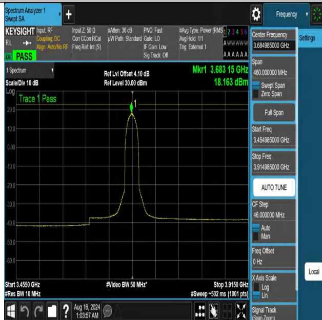
NTNV-DC_13A_n48A-PC3-30-5+30-M+H-N/A-N/A-DFT-64QAM-In ner_Full-3454.985-3914.985-PASS
