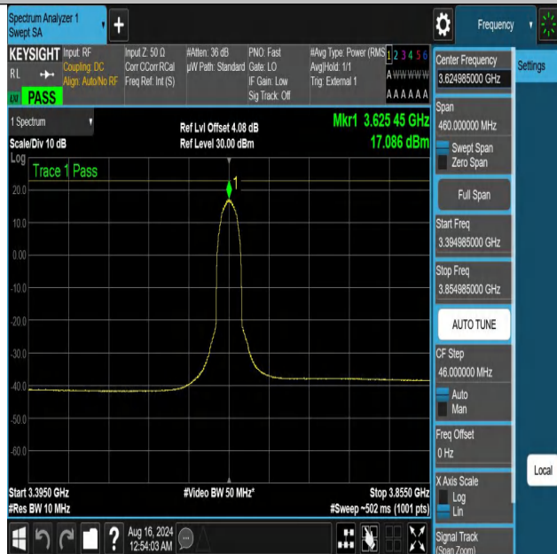
NTNV-DC_13A_n48A-PC3-30-5+30-M+M-N/A-N/A-CP-64QAM-Inner_Full-3394.985-3854.985-PASS
