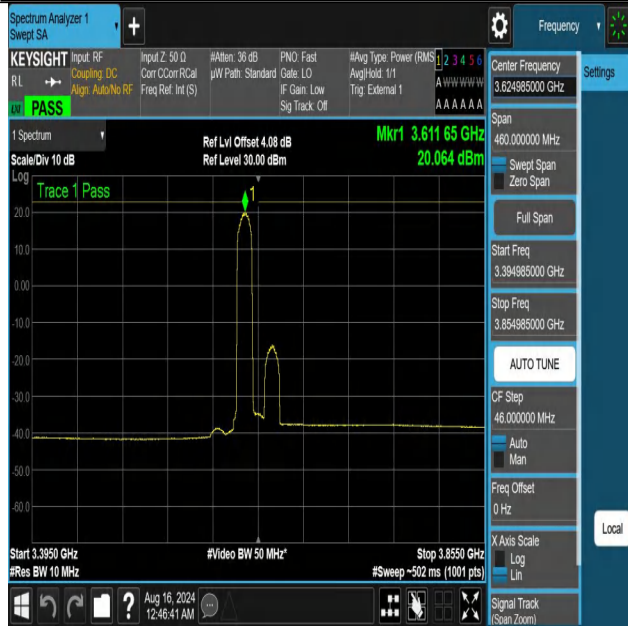
NTNV-DC_13A_n48A-PC3-30-5+30-M+M-N/A-N/A-DFT-64QAM-E dge_1RB_Left-3394.985-3854.985-PASS
