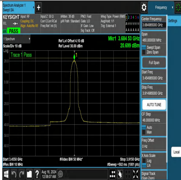
NTNV-DC_13A_n48A-PC3-30-5+30-M+H-N/A-N/A-DFT-PI2BPSK-I nner_Full-3454.985-3914.985-PASS
