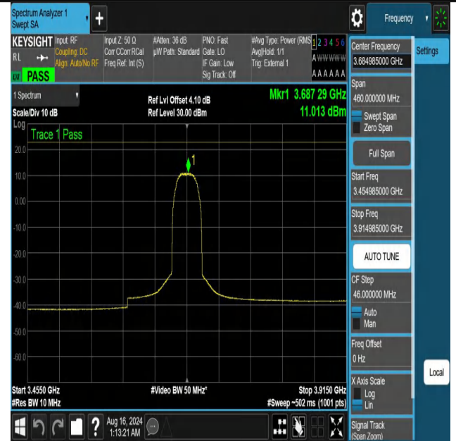
NTNV-DC_13A_n48A-PC3-30-5+30-M+H-N/A-N/A-CP-256QAM-Ou ter_Full-3454.985-3914.985-PASS
