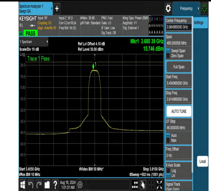
NTNV-DC_13A_n48A-PC3-30-5+30-M+H-N/A-N/A-DFT-16QAM-Ou ter_Full-3454.985-3914.985-PASS
