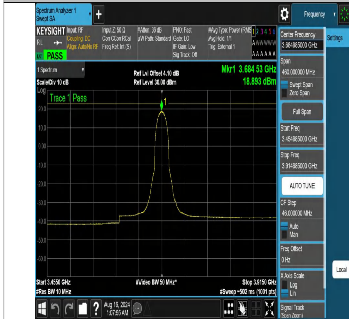
NTNV-DC_13A_n48A-PC3-30-5+30-M+H-N/A-N/A-CP-QPSK-Inner _Full-3454.985-3914.985-PASS
