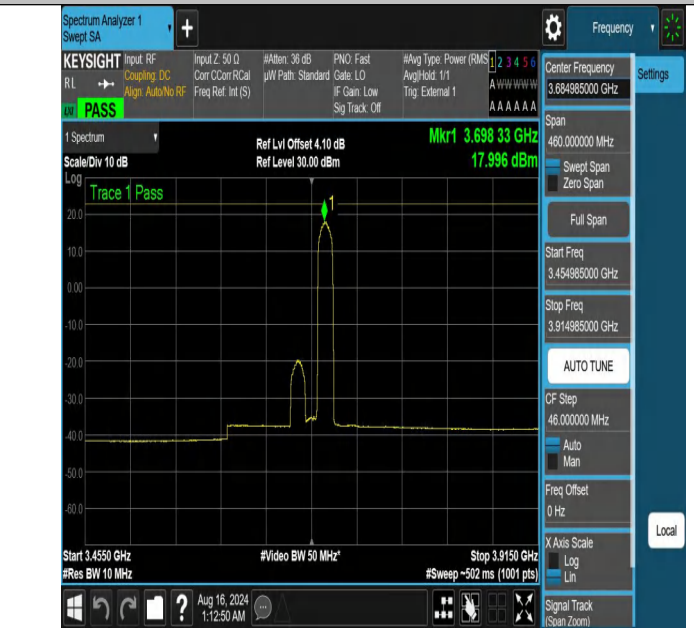
NTNV-DC_13A_n48A-PC3-30-5+30-M+H-N/A-N/A-CP-64QAM-Edge_1RB_Right-3454.985-3914.985-PASS
