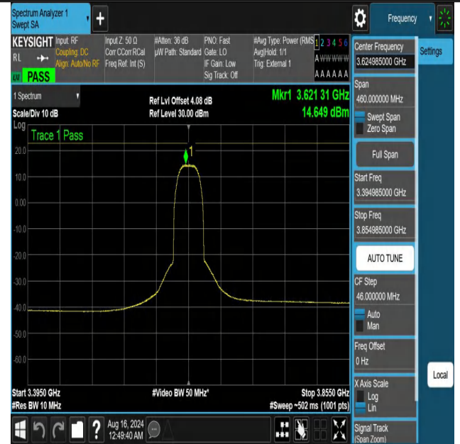
NTNV-DC_13A_n48A-PC3-30-5+30-M+M-N/A-N/A-CP-QPSK-Outer _Full-3394.985-3854.985-PASS
