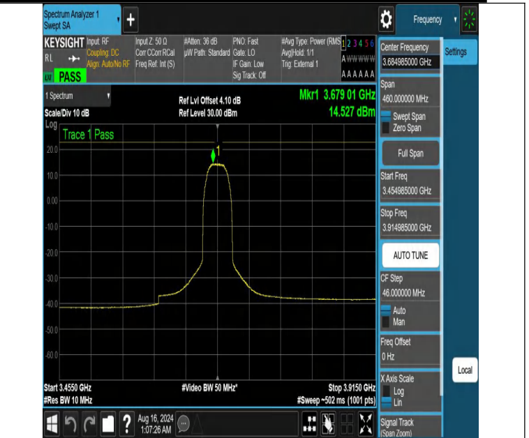
NTNV-DC_13A_n48A-PC3-30-5+30-M+H-N/A-N/A-CP-QPSK-Outer _Full-3454.985-3914.985-PASS
