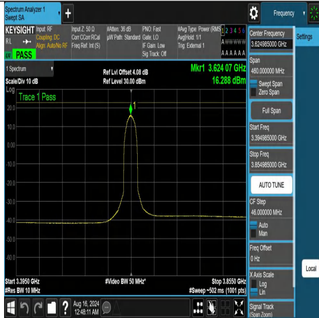
NTNV-DC_13A_n48A-PC3-30-5+30-M+M-N/A-N/A-DFT-256QAM-Inner_Full-3394.985-3854.985-PASS
