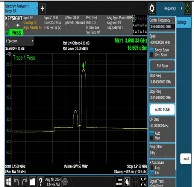
NTNV-DC_13A_n48A-PC3-30-5+30-M+H-N/A-N/A-CP-256QAM-Ed ge_1RB_Right-3454.985-3914.985-PASS
