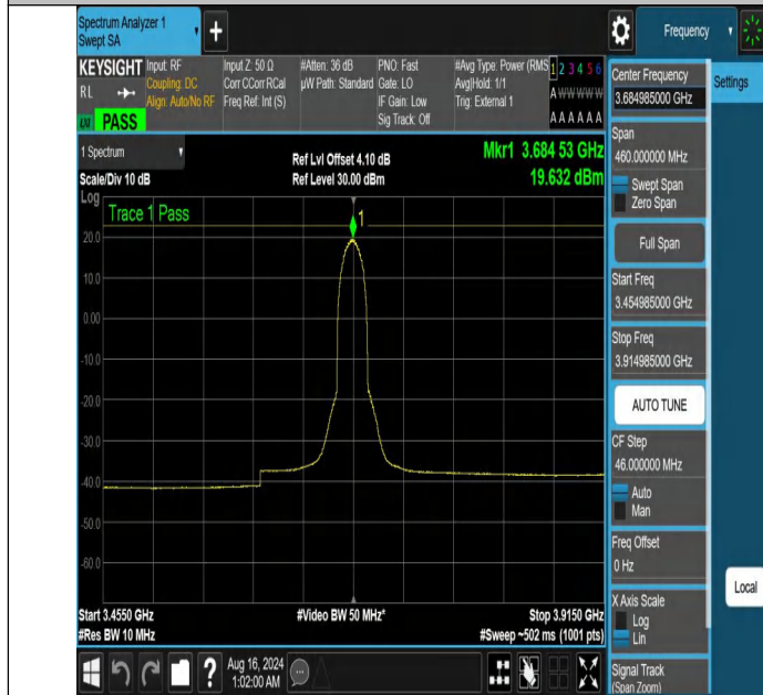
NTNV-DC_13A_n48A-PC3-30-5+30-M+H-N/A-N/A-DFT-16QAM-In ner_Full-3454.985-3914.985-PASS
