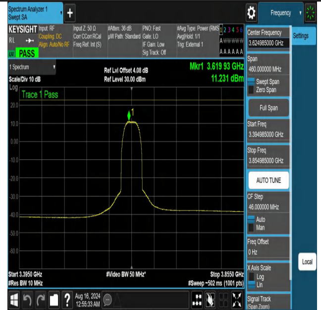
NTNV-DC_13A_n48A-PC3-30-5+30-M+M-N/A-N/A-CP-256QAM-Ou ter_Full-3394.985-3854.985-PASS
