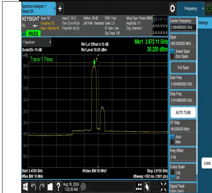
NTNV-DC_13A_n48A-PC3-30-5+30-M+H-N/A-N/A-DFT-16QAM-E dge_1RB_Left-3454.985-3914.985-PASS
