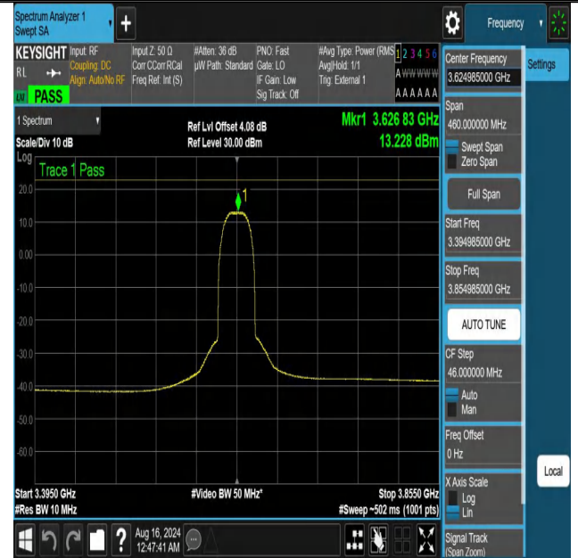
NTNV-DC_13A_n48A-PC3-30-5+30-M+M-N/A-N/A-DFT-256QAM-Outer_Full-3394.985-3854.985-PASS
