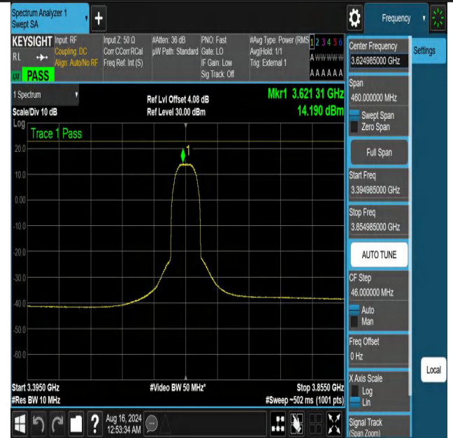
NTNV-DC_13A_n48A-PC3-30-5+30-M+M-N/A-N/A-CP-64QAM-Outer_Full-3394.985-3854.985-PASS
