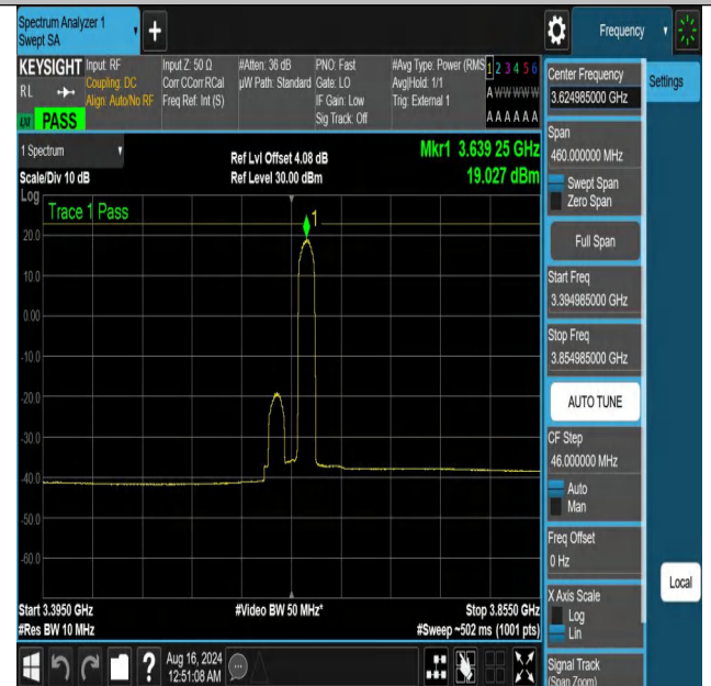
NTNV-DC_13A_n48A-PC3-30-5+30-M+M-N/A-N/A-CP-QPSK-Edge _1RB_Right-3394.985-3854.985-PASS
