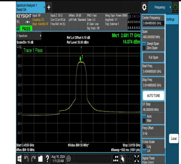
NTNV-DC_13A_n48A-PC3-30-5+30-M+H-N/A-N/A-CP-64QAM-Outer_Full-3454.985-3914.985-PASS
