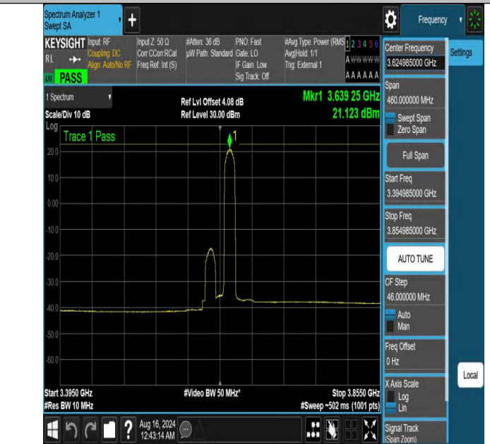
NTNV-DC_13A_n48A-PC3-30-5+30-M+M-N/A-N/A-DFT-QPSK-Edg e_1RB_Right-3394.985-3854.985-PASS
