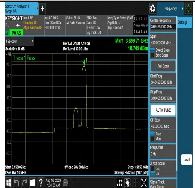
NTNV-DC_13A_n48A-PC3-30-5+30-M+H-N/A-N/A-DFT-64QAM-Ed ge_1RB_Right-3454.985-3914.985-PASS
