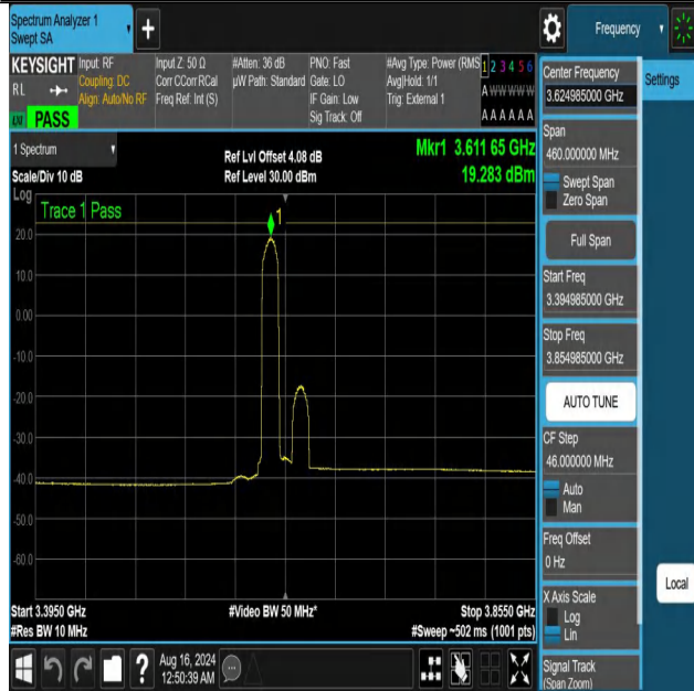
NTNV-DC_13A_n48A-PC3-30-5+30-M+M-N/A-N/A-CP-QPSK-Edge e_1RB_Left-3394.985-3854.985-PASS
