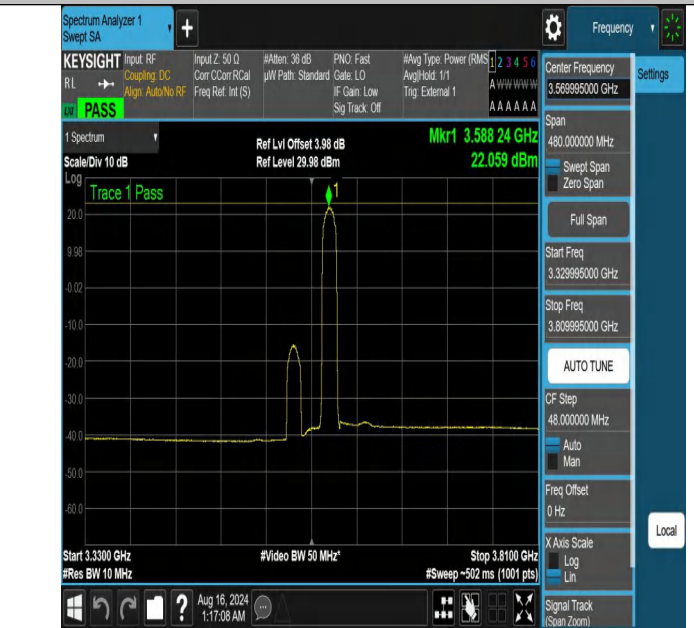
NTNV-DC_13A_n48A-PC3-30-5+40-M+L-N/A-N/A-DFT-PI2BPSK-E dge_1RB_Right-3329.995-3809.995-PASS
