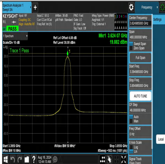
NTNV-DC_13A_n48A-PC3-30-5+30-M+M-N/A-N/A-DFT-16QAM-In ner_Full-3394.985-3854.985-PASS
