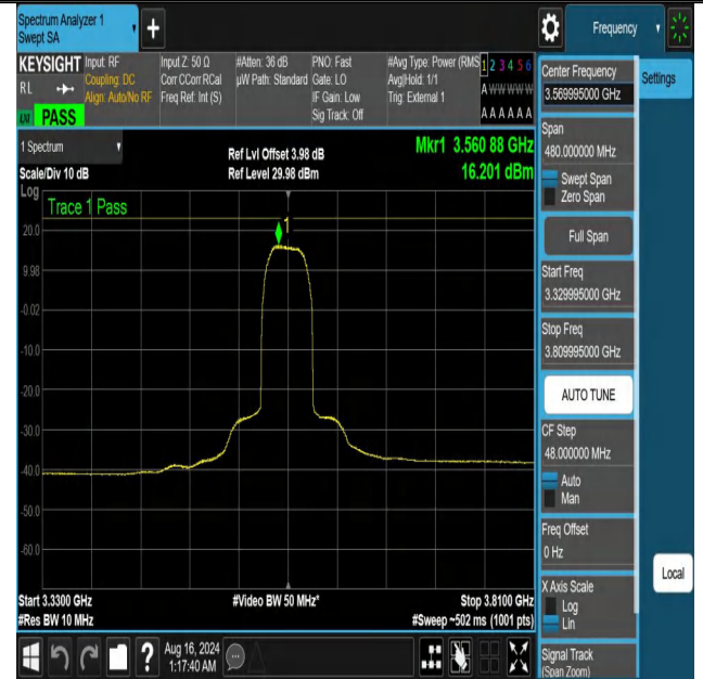
NTNV-DC_13A_n48A-PC3-30-5+40-M+L-N/A-N/A-DFT-QPSK-Oute r_Full-3329.995-3809.995-PASS
