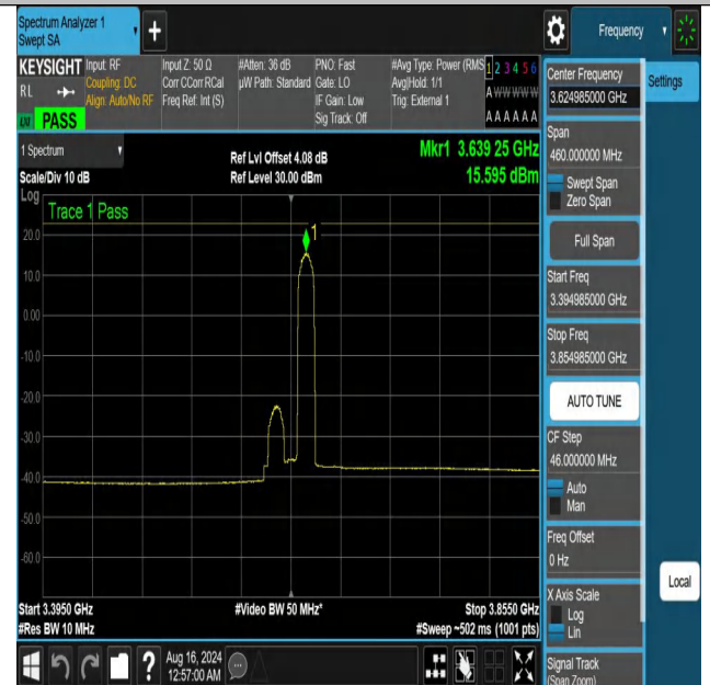
NTNV-DC_13A_n48A-PC3-30-5+30-M+M-N/A-N/A-CP-256QAM-Ed ge_1RB_Right-3394.985-3854.985-PASS
