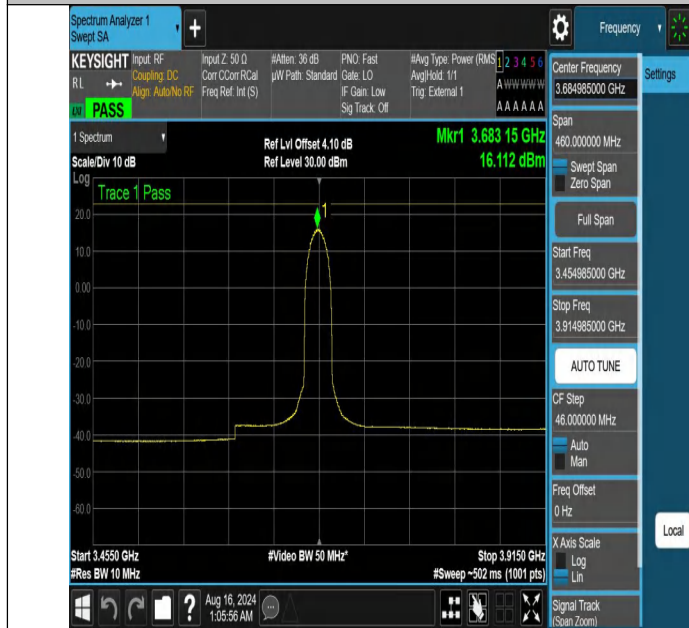
NTNV-DC_13A_n48A-PC3-30-5+30-M+H-N/A-N/A-DFT-256QAM-Inner_Full-3454.985-3914.985-PASS
