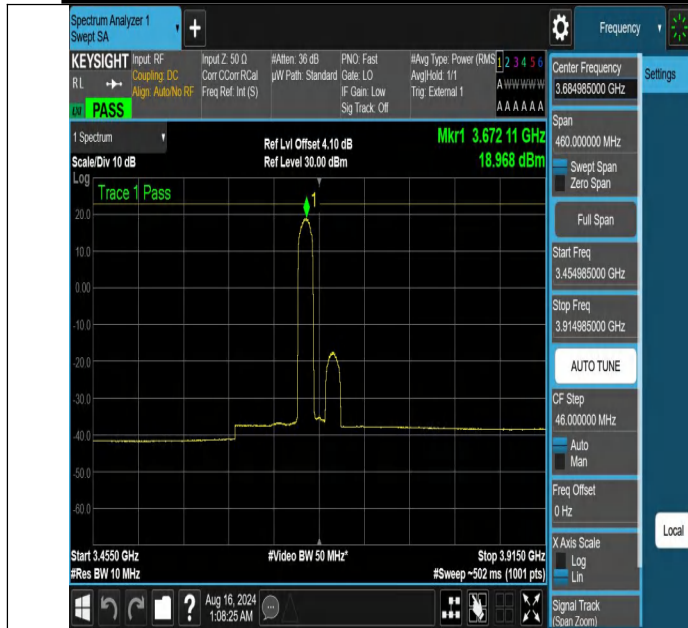
NTNV-DC_13A_n48A-PC3-30-5+30-M+H-N/A-N/A-CP-QPSK-Edge e_1RB_Left-3454.985-3914.985-PASS
