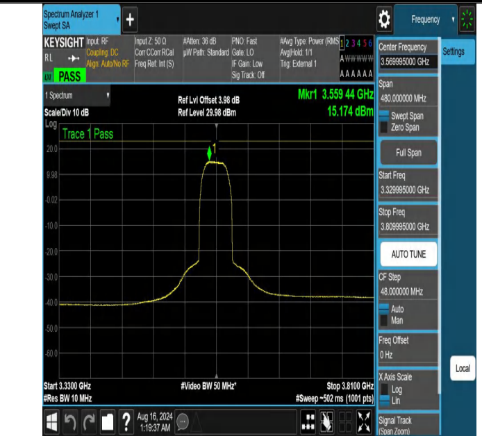
NTNV-DC_13A_n48A-PC3-30-5+40-M+L-N/A-N/A-DFT-16QAM-Out er_Full-3329.995-3809.995-PASS
