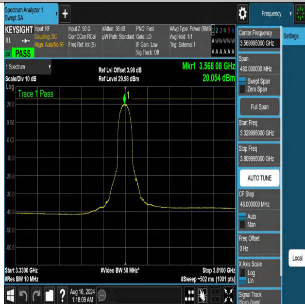
NTNV-DC_13A_n48A-PC3-30-5+40-M+L-N/A-N/A-DFT-QPSK-Inne r_Full-3329.995-3809.995-PASS
