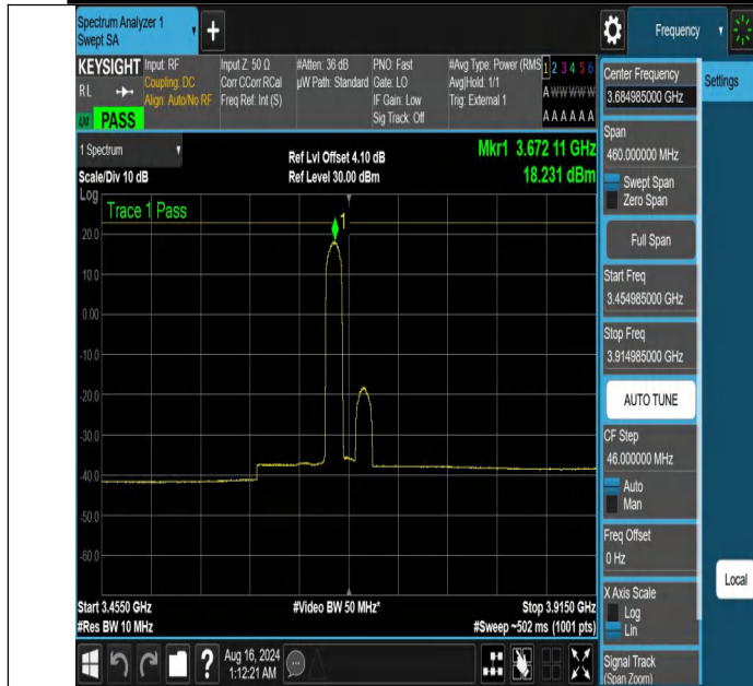
NTNV-DC_13A_n48A-PC3-30-5+30-M+H-N/A-N/A-CP-64QAM-Edge_1RB_Left-3454.985-3914.985-PASS
