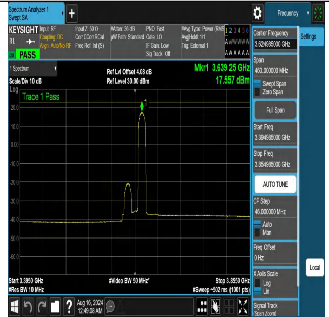
NTNV-DC_13A_n48A-PC3-30-5+30-M+M-N/A-N/A-DFT-256QAM-Edge_1RB_Right-3394.985-3854.985-PASS
