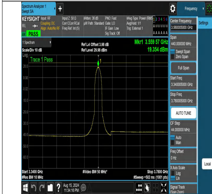
NTNV-DC_13A_n48A-PC3-30-5+20-M+L-N/A-N/A-DFT-64QAM-In ner_Full-3340.005-3780.005-PASS
