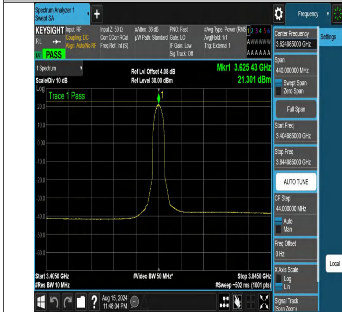
NTNV-DC_13A_n48A-PC3-30-5+20-M+M-N/A-N/A-DFT-QPSK-Inner_Full-3404.985-3844.985-PASS
