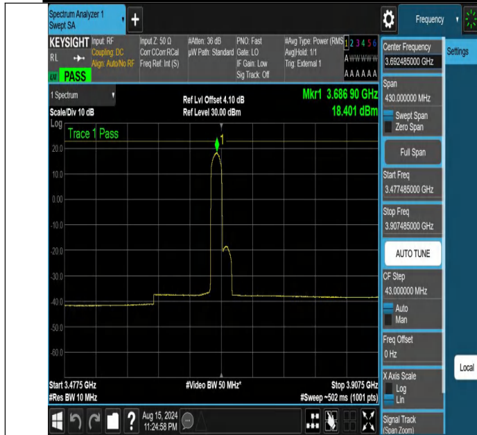
NTNV-DC_13A_n48A-PC3-30-5+15-M+H-N/A-N/A-CP-64QAM-Edge_1RB_Left-3477.485-3907.485-PASS
