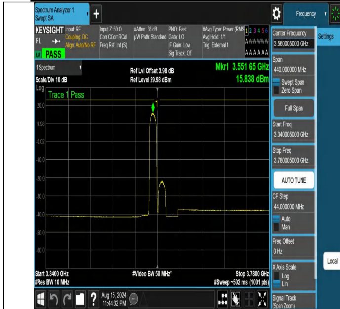
NTNV-DC_13A_n48A-PC3-30-5+20-M+L-N/A-N/A-CP-256QAM-Ed ge_1RB_Left-3340.005-3780.005-PASS
