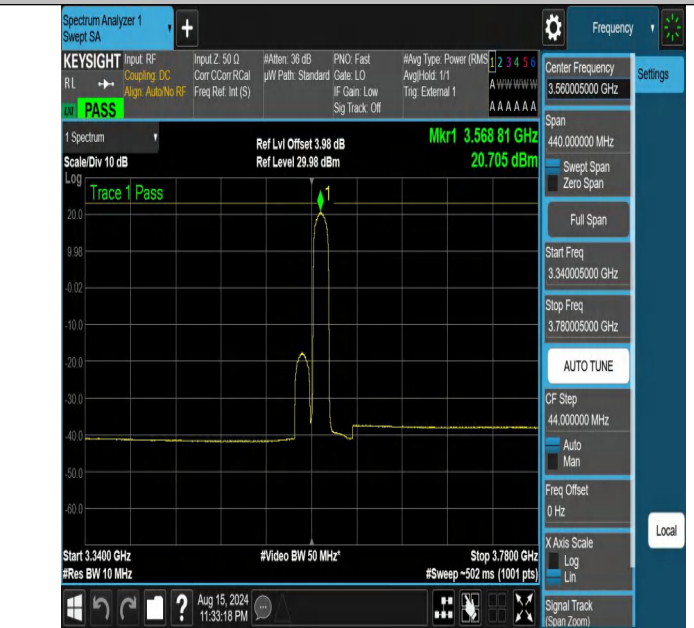
NTNV-DC_13A_n48A-PC3-30-5+20-M+L-N/A-N/A-DFT-16QAM-Ed ge_1RB_Right-3340.005-3780.005-PASS
