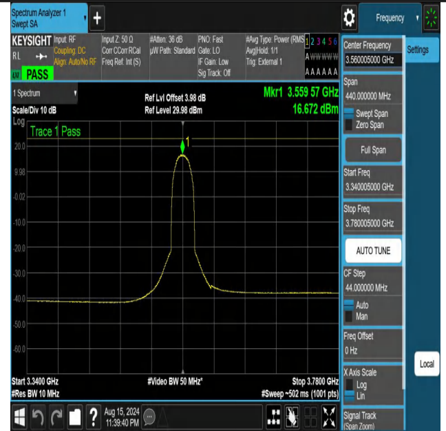
NTNV-DC_13A_n48A-PC3-30-5+20-M+L-N/A-N/A-CP-16QAM-Oute r_Full-3340.005-3780.005-PASS
