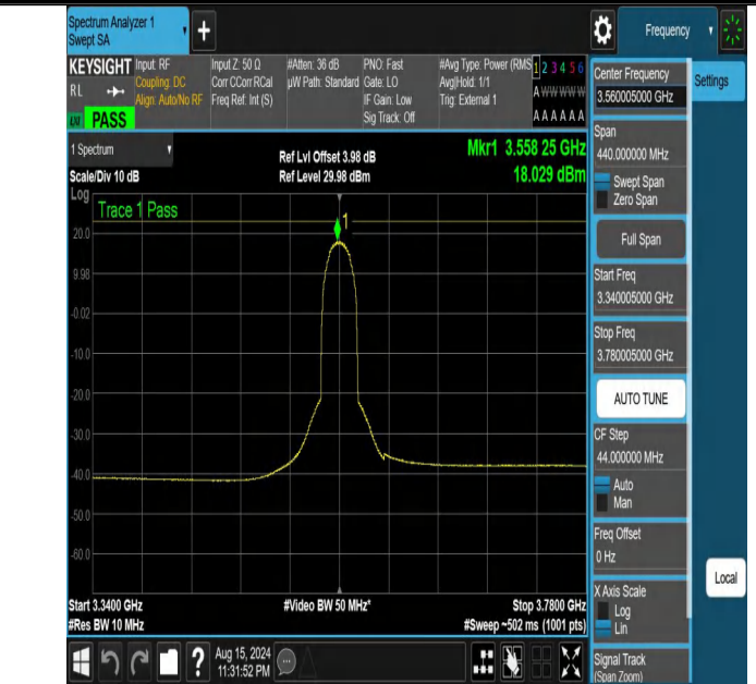
NTNV-DC_13A_n48A-PC3-30-5+20-M+L-N/A-N/A-DFT-16QAM-Out er_Full-3340.005-3780.005-PASS
