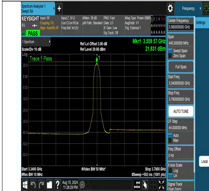
NTNV-DC_13A_n48A-PC3-30-5+20-M+L-N/A-N/A-DFT-PI2BPSK-I nner_Full-3340.005-3780.005-PASS
