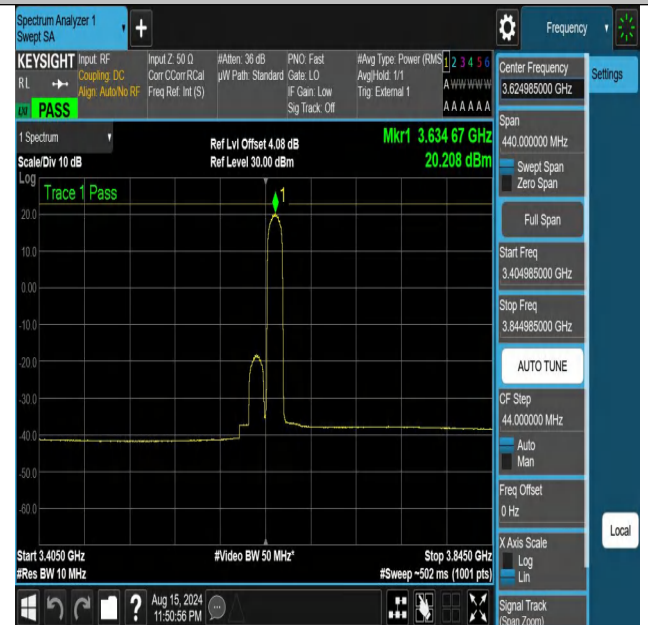
NTNV-DC_13A_n48A-PC3-30-5+20-M+M-N/A-N/A-DFT-16QAM-Ed ge_1RB_Right-3404.985-3844.985-PASS
