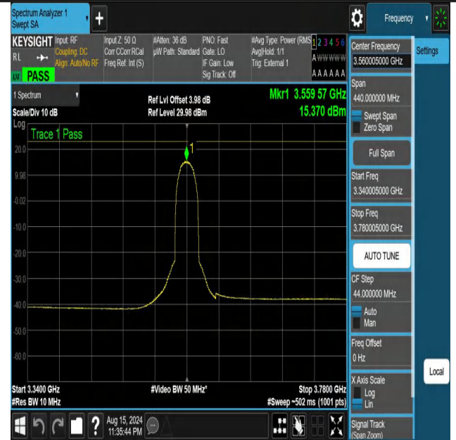
NTNV-DC_13A_n48A-PC3-30-5+20-M+L-N/A-N/A-DFT-256QAM-O uter_Full-3340.005-3780.005-PASS
