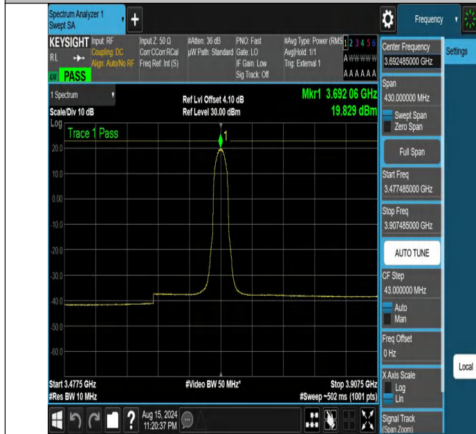
NTNV-DC_13A_n48A-PC3-30-5+15-M+H-N/A-N/A-CP-QPSK-Inner _Full-3477.485-3907.485-PASS
