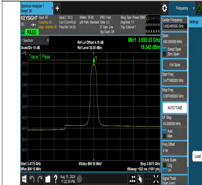
NTNV-DC_13A_n48A-PC3-30-5+15-M+H-N/A-N/A-CP-16QAM-Inner_Full-3477.485-3907.485-PASS
