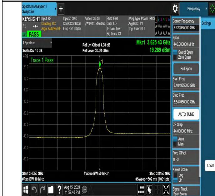
NTNV-DC_13A_n48A-PC3-30-5+20-M+M-N/A-N/A-CP-16QAM-Inner_Full-3404.985-3844.985-PASS
