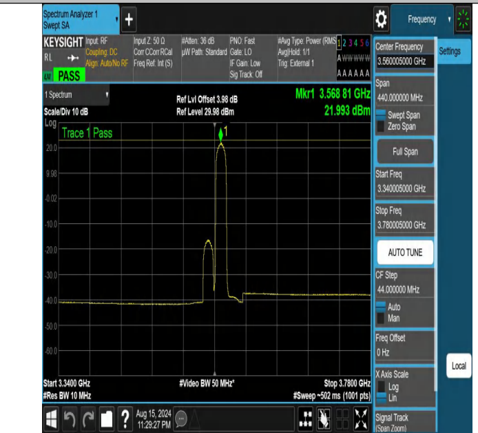
NTNV-DC_13A_n48A-PC3-30-5+20-M+L-N/A-N/A-DFT-PI2BPSK-E dge_1RB_Right-3340.005-3780.005-PASS
