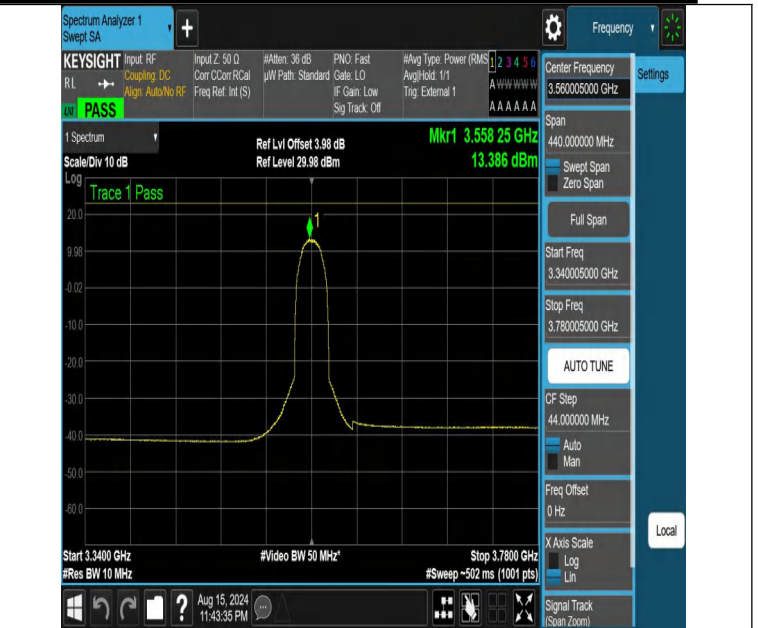
NTNV-DC_13A_n48A-PC3-30-5+20-M+L-N/A-N/A-CP-256QAM-Out er_Full-3340.005-3780.005-PASS
