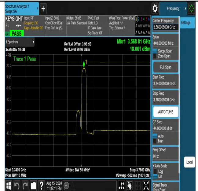
NTNV-DC_13A_n48A-PC3-30-5+20-M+L-N/A-N/A-DFT-256QAM-E dge_1RB_Right-3340.005-3780.005-PASS
