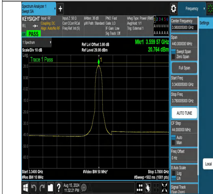
NTNV-DC_13A_n48A-PC3-30-5+20-M+L-N/A-N/A-DFT-16QAM-In ner_Full-3340.005-3780.005-PASS
