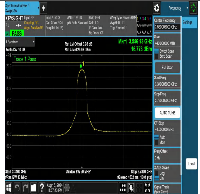
NTNV-DC_13A_n48A-PC3-30-5+20-M+L-N/A-N/A-CP-QPSK-Outer _Full-3340.005-3780.005-PASS
