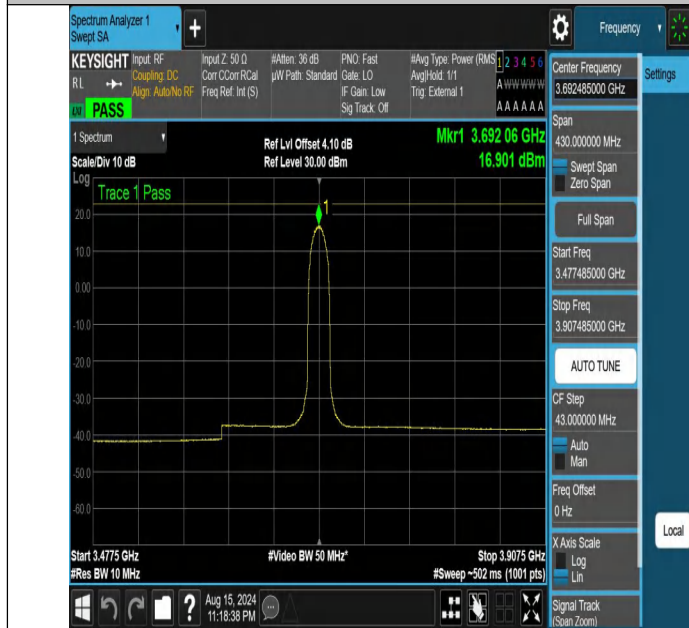
NTNV-DC_13A_n48A-PC3-30-5+15-M+H-N/A-N/A-DFT-256QAM-Inner_Full-3477.485-3907.485-PASS
