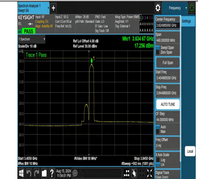
NTNV-DC_13A_n48A-PC3-30-5+20-M+M-N/A-N/A-DFT-256QAM-Edge_1RB_Right-3404.985-3844.985-PASS
