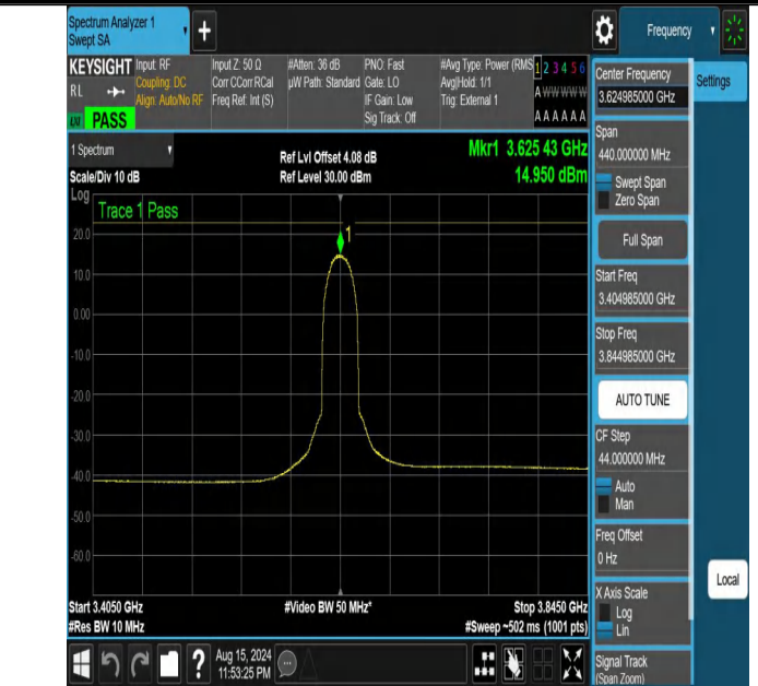
NTNV-DC_13A_n48A-PC3-30-5+20-M+M-N/A-N/A-DFT-256QAM-Outer_Full-3404.985-3844.985-PASS
