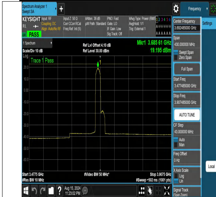
NTNV-DC_13A_n48A-PC3-30-5+15-M+H-N/A-N/A-CP-16QAM-Edge_1RB_Left-3477.485-3907.485-PASS
