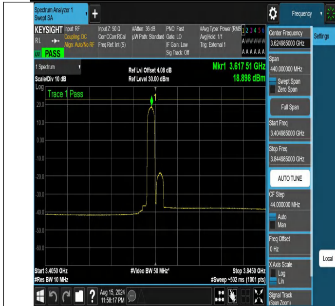
NTNV-DC_13A_n48A-PC3-30-5+20-M+M-N/A-N/A-CP-16QAM-Edge_1RB_Left-3404.985-3844.985-PASS
