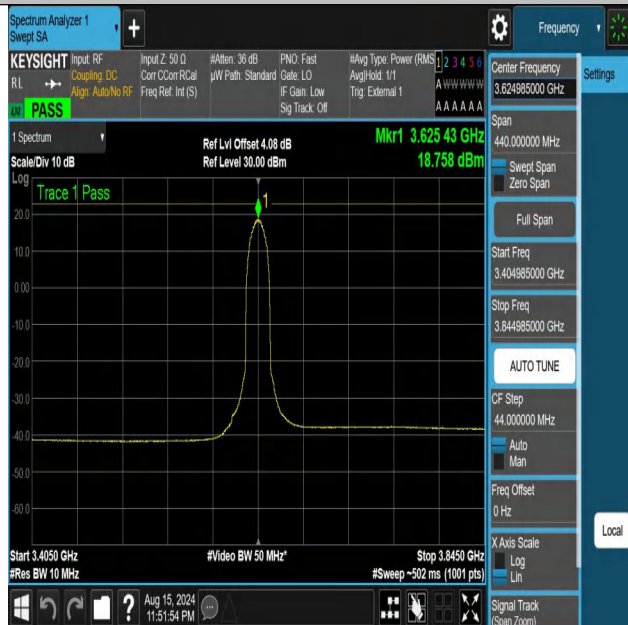
NTNV-DC_13A_n48A-PC3-30-5+20-M+M-N/A-N/A-DFT-64QAM-In ner_Full-3404.985-3844.985-PASS
