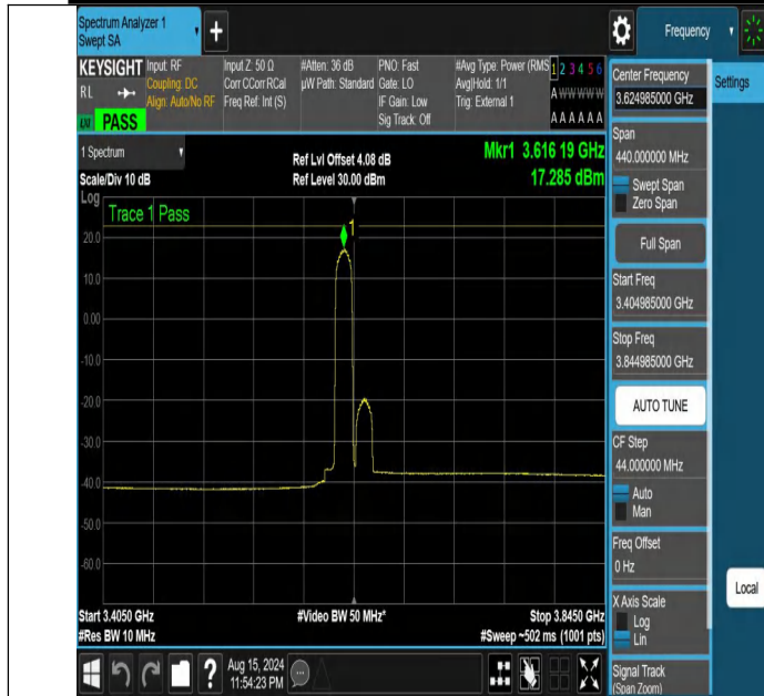
NTNV-DC_13A_n48A-PC3-30-5+20-M+M-N/A-N/A-DFT-256QAM-Edge_1RB_Left-3404.985-3844.985-PASS
