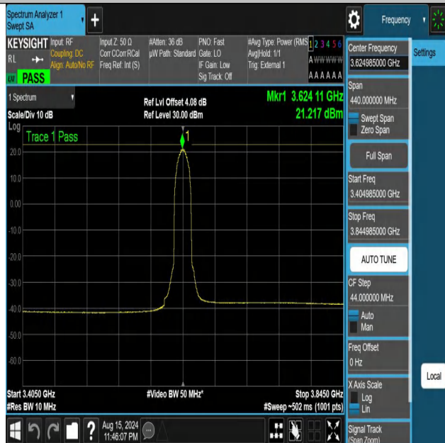
NTNV-DC_13A_n48A-PC3-30-5+20-M+M-N/A-N/A-DFT-PI2BPSK-I nner_Full-3404.985-3844.985-PASS
