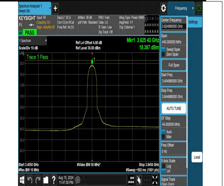
NTNV-DC_13A_n48A-PC3-30-5+20-M+M-N/A-N/A-DFT-QPSK-Outer_Full-3404.985-3844.985-PASS
