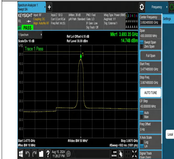
NTNV-DC_13A_n48A-PC3-30-5+15-M+H-N/A-N/A-CP-256QAM-In ner_Full-3477.485-3907.485-PASS
