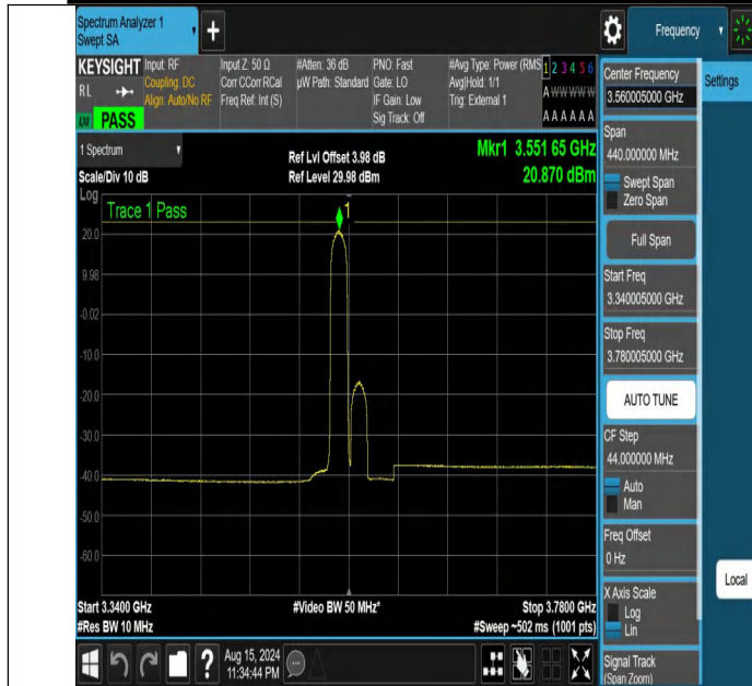
NTNV-DC_13A_n48A-PC3-30-5+20-M+L-N/A-N/A-DFT-64QAM-Ed ge_1RB_Left-3340.005-3780.005-PASS
