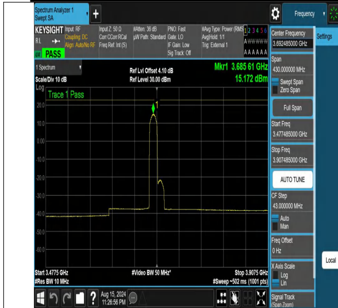
NTNV-DC_13A_n48A-PC3-30-5+15-M+H-N/A-N/A-CP-256QAM-E dge_1RB_Left-3477.485-3907.485-PASS
