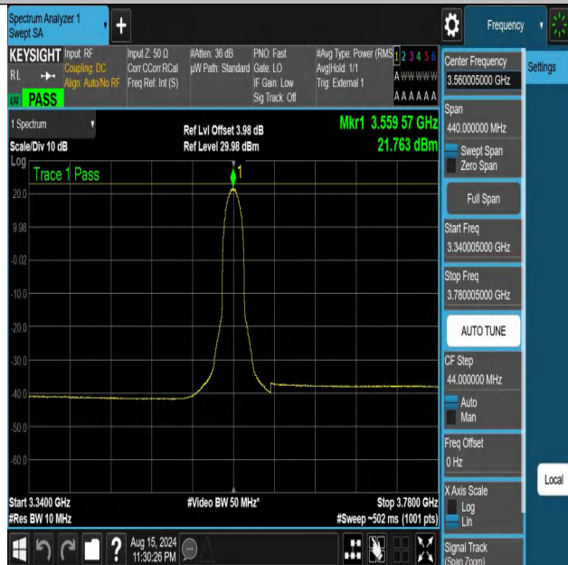
NTNV-DC_13A_n48A-PC3-30-5+20-M+L-N/A-N/A-DFT-QPSK-Inne r_Full-3340.005-3780.005-PASS
