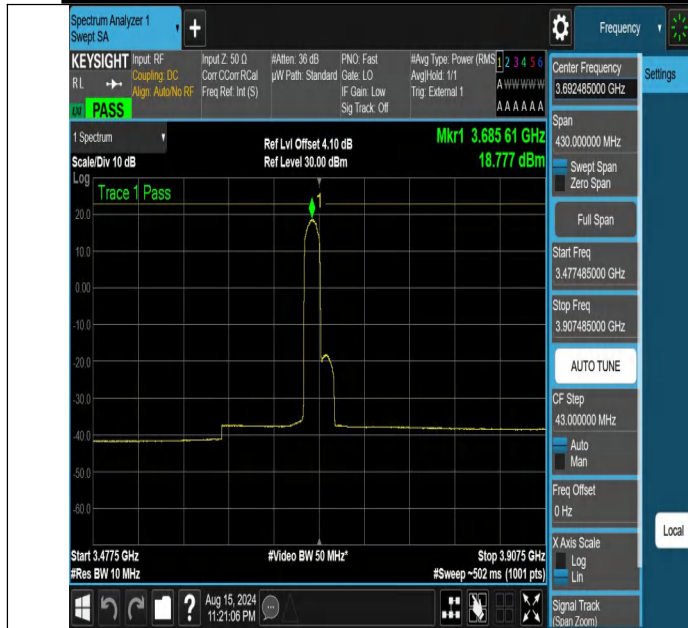
NTNV-DC_13A_n48A-PC3-30-5+15-M+H-N/A-N/A-CP-QPSK-Edge e_1RB_Left-3477.485-3907.485-PASS
