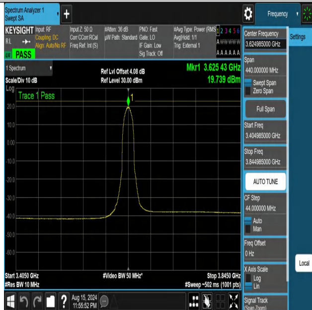
NTNV-DC_13A_n48A-PC3-30-5+20-M+M-N/A-N/A-CP-QPSK-Inne r_Full-3404.985-3844.985-PASS
