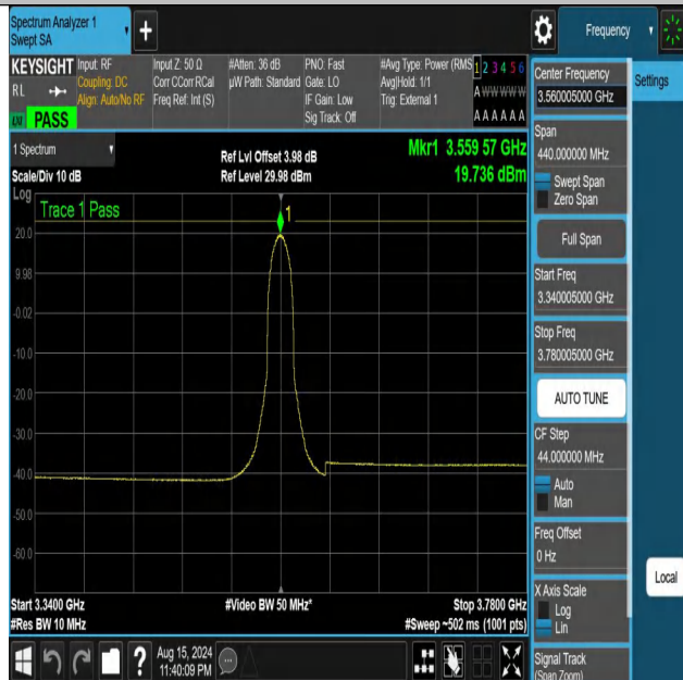
NTNV-DC_13A_n48A-PC3-30-5+20-M+L-N/A-N/A-CP-16QAM-Inn er_Full-3340.005-3780.005-PASS
