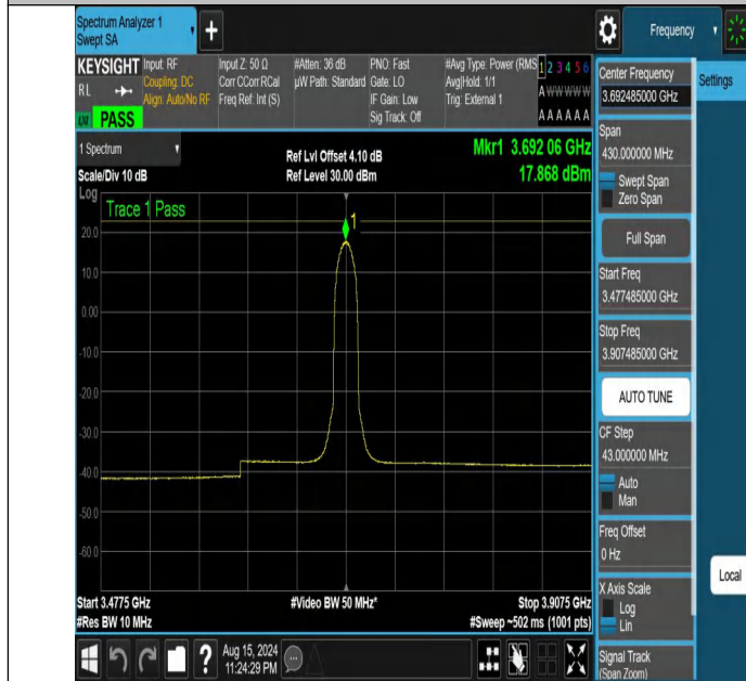
NTNV-DC_13A_n48A-PC3-30-5+15-M+H-N/A-N/A-CP-64QAM-Inner_Full-3477.485-3907.485-PASS
