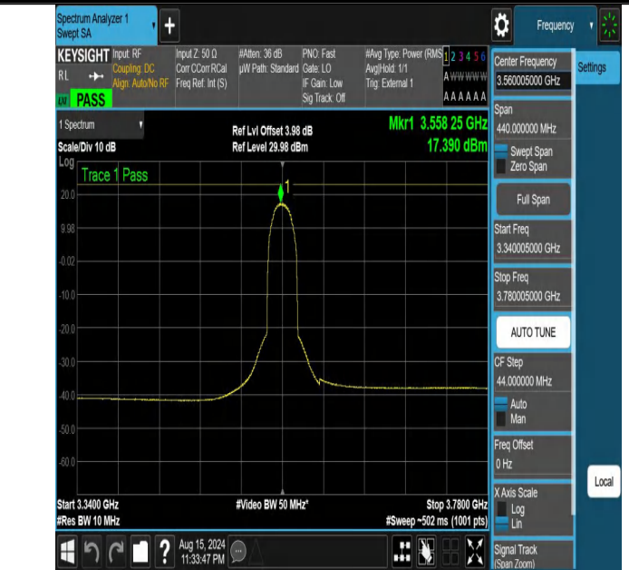
NTNV-DC_13A_n48A-PC3-30-5+20-M+L-N/A-N/A-DFT-64QAM-Out er_Full-3340.005-3780.005-PASS
