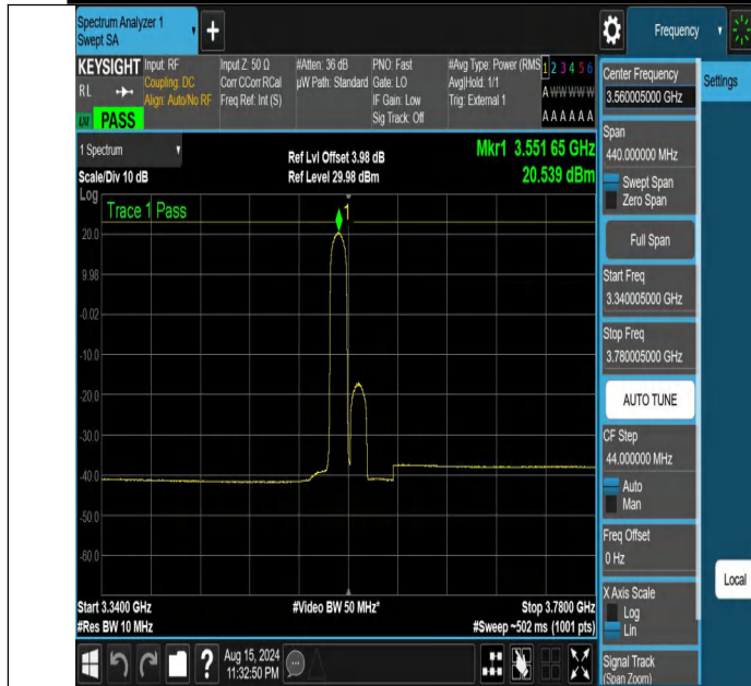
NTNV-DC_13A_n48A-PC3-30-5+20-M+L-N/A-N/A-DFT-16QAM-Ed ge_1RB_Left-3340.005-3780.005-PASS
