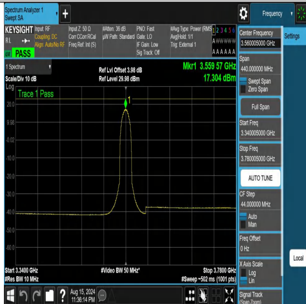
NTNV-DC_13A_n48A-PC3-30-5+20-M+L-N/A-N/A-DFT-256QAM-I nner_Full-3340.005-3780.005-PASS
