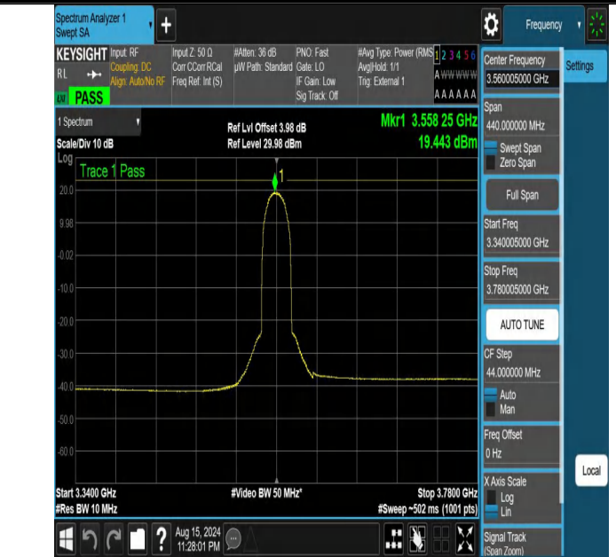
NTNV-DC_13A_n48A-PC3-30-5+20-M+L-N/A-N/A-DFT-PI2BPSK-O uter_Full-3340.005-3780.005-PASS
