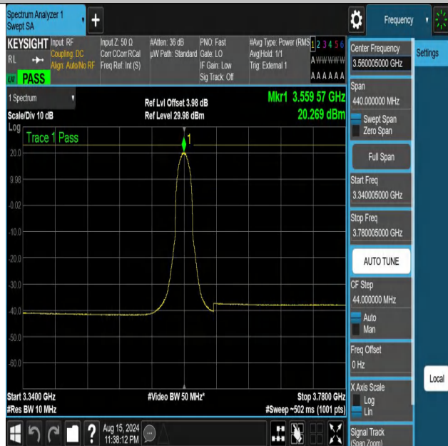
NTNV-DC_13A_n48A-PC3-30-5+20-M+L-N/A-N/A-CP-QPSK-Inner _Full-3340.005-3780.005-PASS
