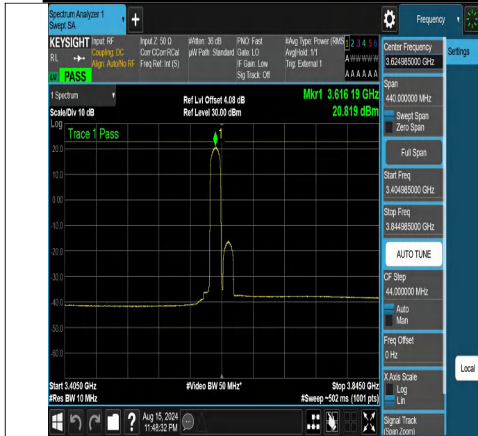
NTNV-DC_13A_n48A-PC3-30-5+20-M+M-N/A-N/A-DFT-QPSK-Edge_1RB_Left-3404.985-3844.985-PASS
