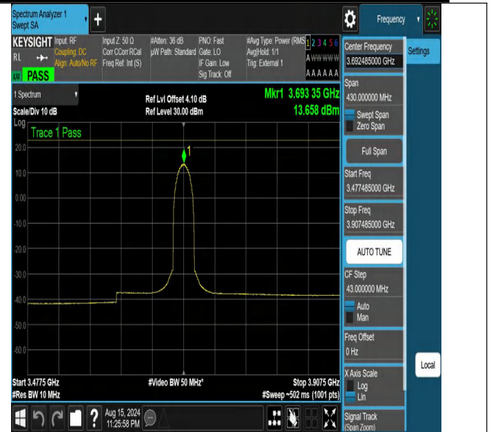
NTNV-DC_13A_n48A-PC3-30-5+15-M+H-N/A-N/A-CP-256QAM-Ou ter_Full-3477.485-3907.485-PASS
