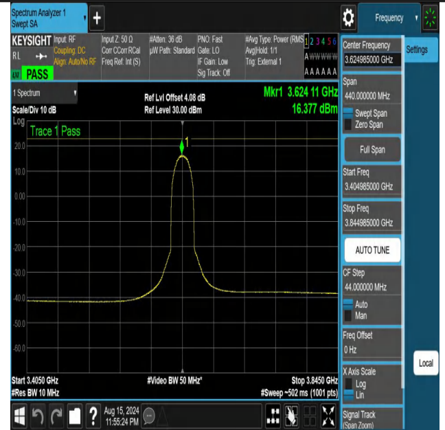
NTNV-DC_13A_n48A-PC3-30-5+20-M+M-N/A-N/A-CP-QPSK-Outer _Full-3404.985-3844.985-PASS
