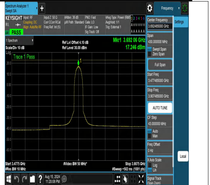
NTNV-DC_13A_n48A-PC3-30-5+15-M+H-N/A-N/A-CP-QPSK-Outer _Full-3477.485-3907.485-PASS
