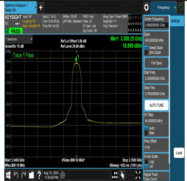
NTNV-DC_13A_n48A-PC3-30-5+20-M+L-N/A-N/A-DFT-QPSK-Oute r_Full-3340.005-3780.005-PASS
