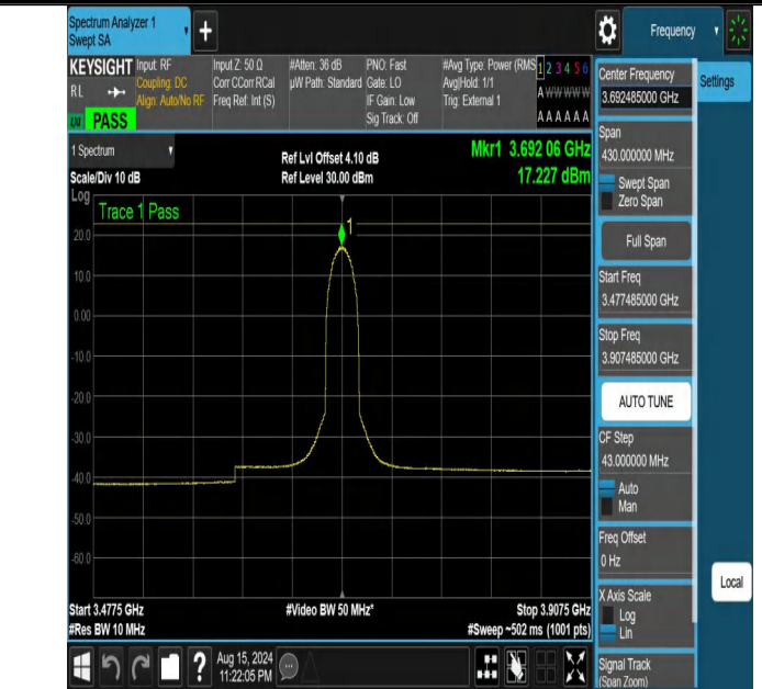
NTNV-DC_13A_n48A-PC3-30-5+15-M+H-N/A-N/A-CP-16QAM-Outer_Full-3477.485-3907.485-PASS
