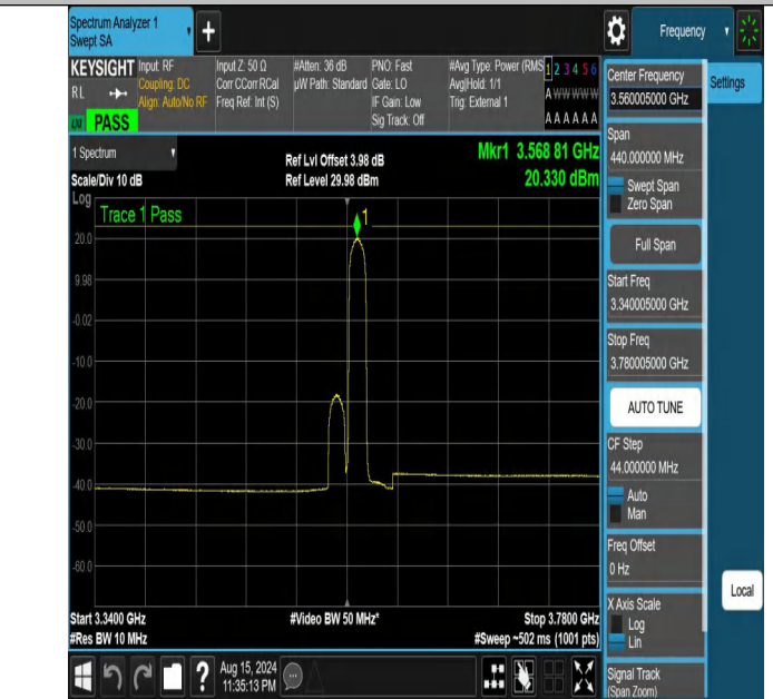
NTNV-DC_13A_n48A-PC3-30-5+20-M+L-N/A-N/A-DFT-64QAM-Ed ge_1RB_Right-3340.005-3780.005-PASS
