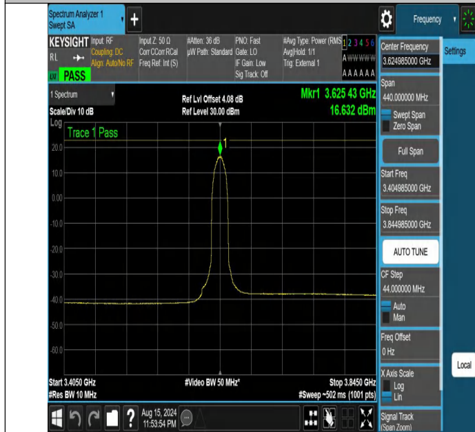
NTNV-DC_13A_n48A-PC3-30-5+20-M+M-N/A-N/A-DFT-256QAM-Inner_Full-3404.985-3844.985-PASS
