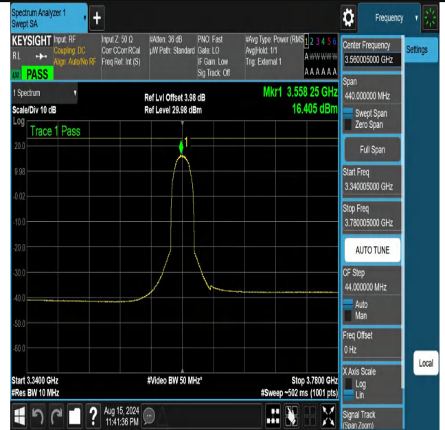
NTNV-DC_13A_n48A-PC3-30-5+20-M+L-N/A-N/A-CP-64QAM-Outer_Full-3340.005-3780.005-PASS
