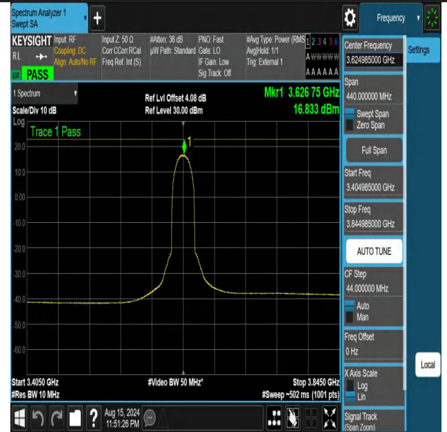
NTNV-DC_13A_n48A-PC3-30-5+20-M+M-N/A-N/A-DFT-64QAM-Ou ter_Full-3404.985-3844.985-PASS
