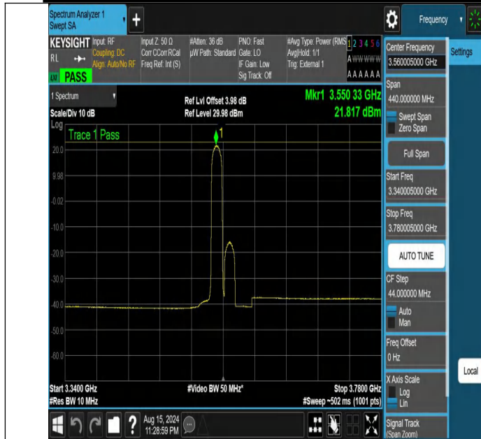
NTNV-DC_13A_n48A-PC3-30-5+20-M+L-N/A-N/A-DFT-PI2BPSK- Edge_1RB_Left-3340.005-3780.005-PASS
