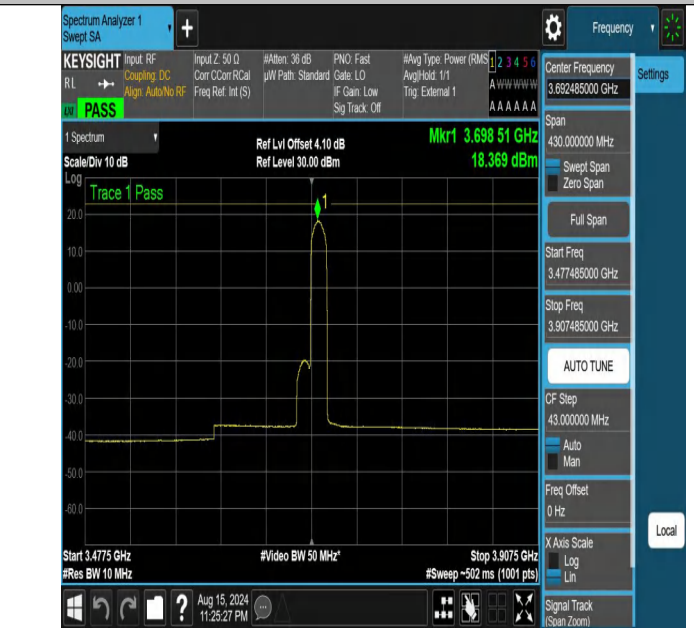
NTNV-DC_13A_n48A-PC3-30-5+15-M+H-N/A-N/A-CP-64QAM-Edge_1RB_Right-3477.485-3907.485-PASS
