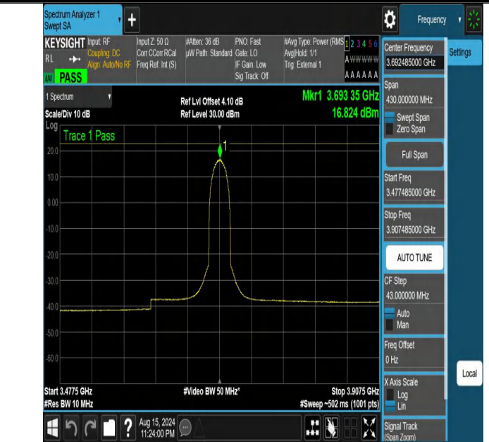
NTNV-DC_13A_n48A-PC3-30-5+15-M+H-N/A-N/A-CP-64QAM-Outer_Full-3477.485-3907.485-PASS
