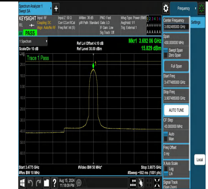
NTNV-DC_13A_n48A-PC3-30-5+15-M+H-N/A-N/A-DFT-256QAM-Outer_Full-3477.485-3907.485-PASS
