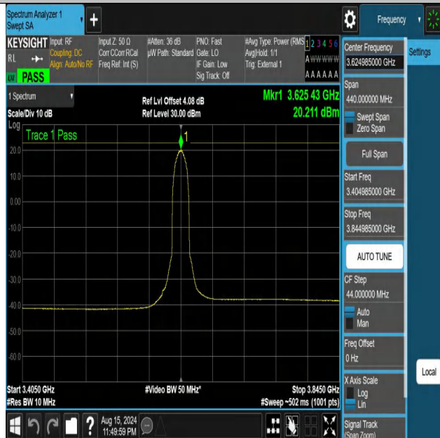
NTNV-DC_13A_n48A-PC3-30-5+20-M+M-N/A-N/A-DFT-16QAM-In ner_Full-3404.985-3844.985-PASS
