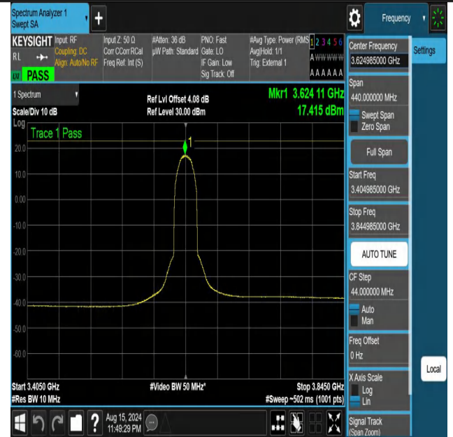
NTNV-DC_13A_n48A-PC3-30-5+20-M+M-N/A-N/A-DFT-16QAM-Ou ter_Full-3404.985-3844.985-PASS
