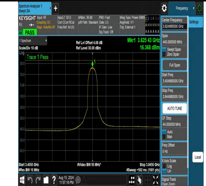
NTNV-DC_13A_n48A-PC3-30-5+20-M+M-N/A-N/A-CP-16QAM-Outer_Full-3404.985-3844.985-PASS
