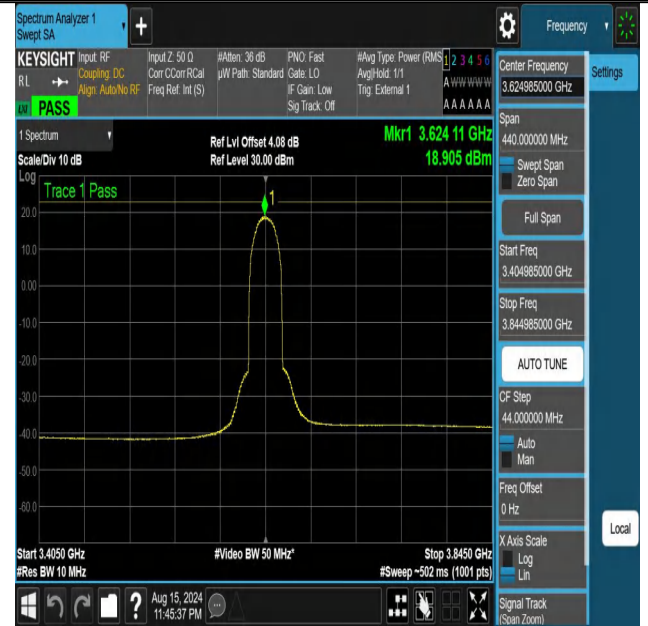
NTNV-DC_13A_n48A-PC3-30-5+20-M+M-N/A-N/A-DFT-PI2BPSK- Outer_Full-3404.985-3844.985-PASS
