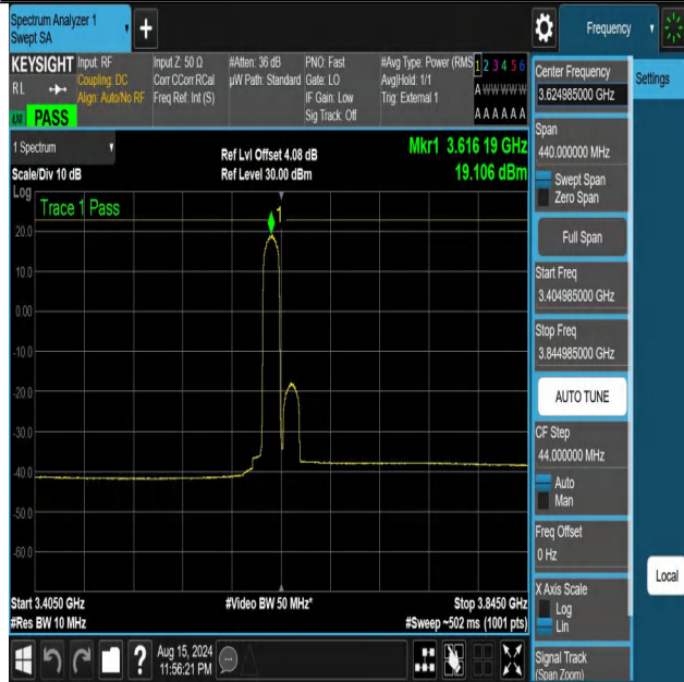
NTNV-DC_13A_n48A-PC3-30-5+20-M+M-N/A-N/A-CP-QPSK-Edge e_1RB_Left-3404.985-3844.985-PASS
