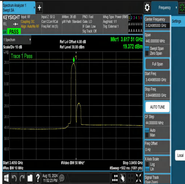
NTNV-DC_13A_n48A-PC3-30-5+20-M+M-N/A-N/A-DFT-64QAM-E dge_1RB_Left-3404.985-3844.985-PASS
