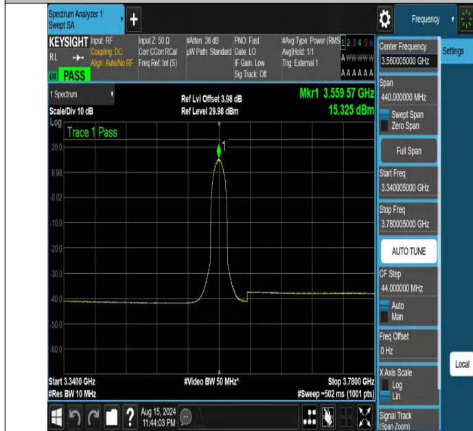
NTNV-DC_13A_n48A-PC3-30-5+20-M+L-N/A-N/A-CP-256QAM-In ner_Full-3340.005-3780.005-PASS
