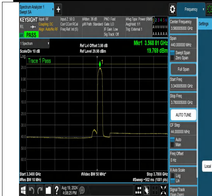
NTNV-N48-PC3-30-20-L-DFT-64QAM-Edge_1RB_Right-3340.00 5-3780.005-Ant1-PASS
