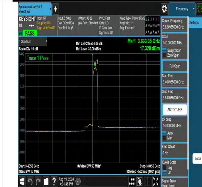
NTNV-N48-PC3-30-20-M-DFT-256QAM-Edge_1RB_Right-3404.985-3844.985-Ant1-PASS
