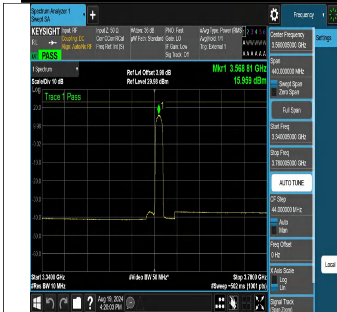
NTNV-N48-PC3-30-20-L-CP-256QAM-Edge_1RB_Right-3340.00 5-3780.005-Ant1-PASS
