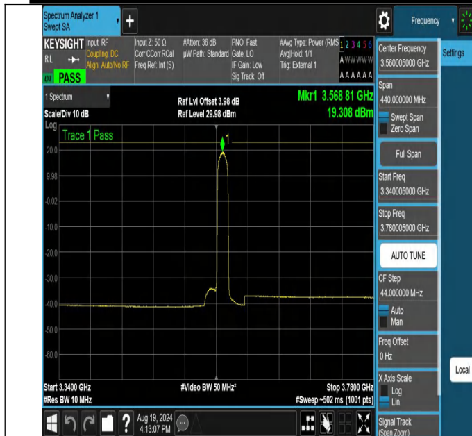
NTNV-N48-PC3-30-20-L-CP-QPSK-Edge_1RB_Right-3340.005-3780.005-Ant1-PASS
