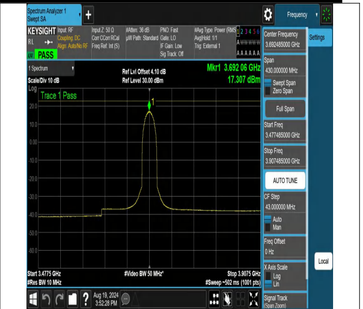
NTN-N48-PC3-30-15-H-CP-16QAM-Outer_Full-3477.485-3907.485-Ant1-PASS
