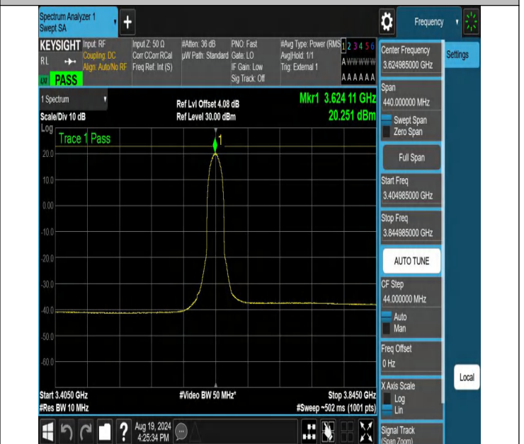
NTNV-N48-PC3-30-20-M-DFT-16QAM-Inner_Full-3404.985-3844. 985-Ant1-PASS
