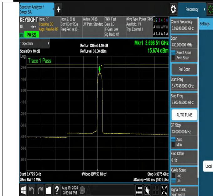
NTNV-N48-PC3-30-15-H-CP-256QAM-Edge_1RB_Right-3477.48 5-3907.485-Ant1-PASS
