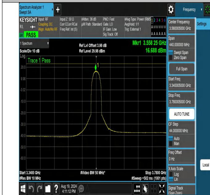
NTNV-N48-PC3-30-20-L-CP-QPSK-Outer_Full-3340.005-3780.00 5-Ant1-PASS
