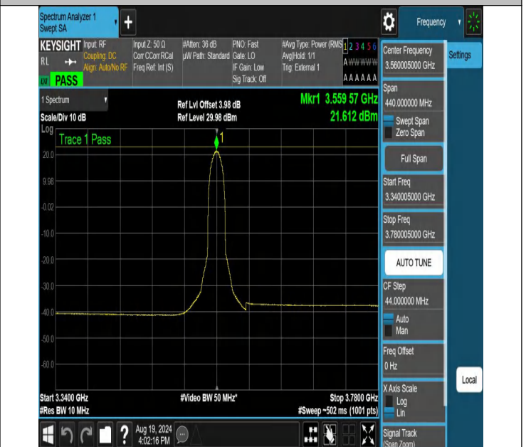
NTNV-N48-PC3-30-20-L-DFT-QPSK-Inner_Full-3340.005-3780.005-Ant1-PASS
