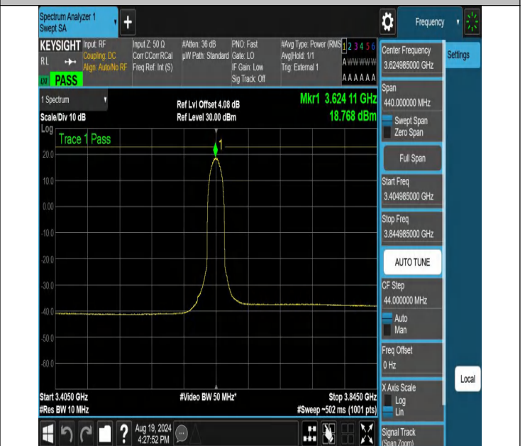
NTNV-N48-PC3-30-20-M-DFT-64QAM-Inner_Full-3404.985-3844.985-Ant1-PASS
