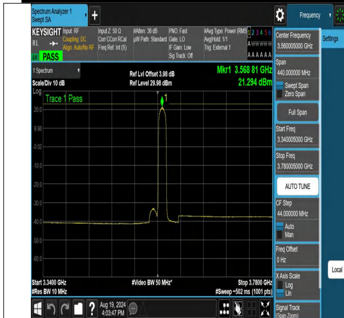
NTNV-N48-PC3-30-20-L-DFT-QPSK-Edge_1RB_Right-3340.005-3780.005-Ant1-PASS
