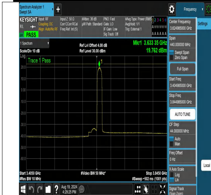
NTNV-N48-PC3-30-20-M-DFT-64QAM-Edge_1RB_Right-3404.98 5-3844.985-Ant1-PASS
