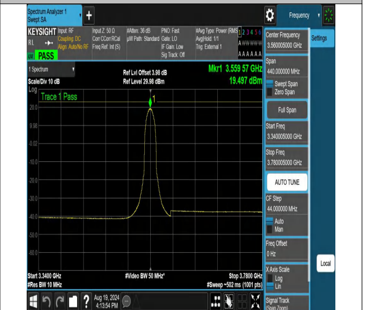
NTNV-N48-PC3-30-20-L-CP-16QAM-Inner_Full-3340.005-3780.005-Ant1-PASS
