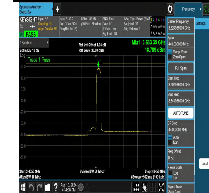
NTNV-N48-PC3-30-20-M-CP-QPSK-Edge_1RB_Right-3404.985-3844.985-Ant1-PASS
