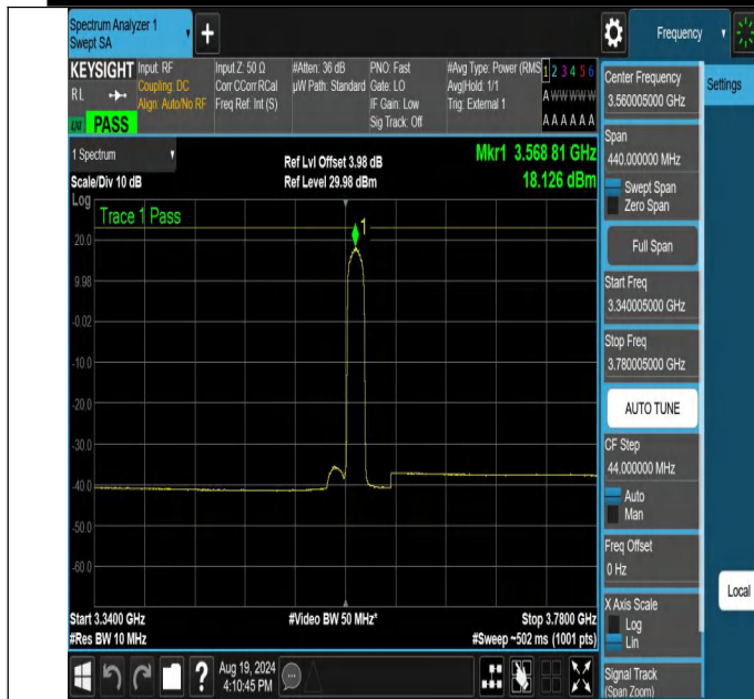
NTNV-N48-PC3-30-20-L-DFT-256QAM-Edge_1RB_Right-3340.0 05-3780.005-Ant1-PASS
