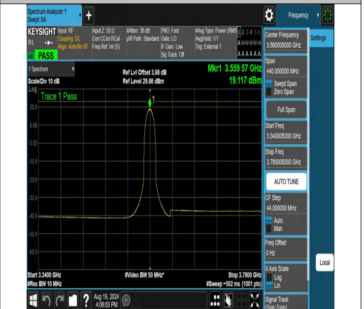
NTNV-N48-PC3-30-20-L-DFT-64QAM-Inner_Full-3340.005-3780. 005-Ant1-PASS
