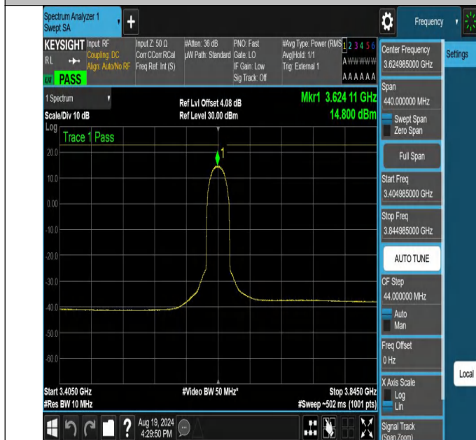
NTNV-N48-PC3-30-20-M-DFT-256QAM-Outer_Full-3404.985-384 4.985-Ant1-PASS
