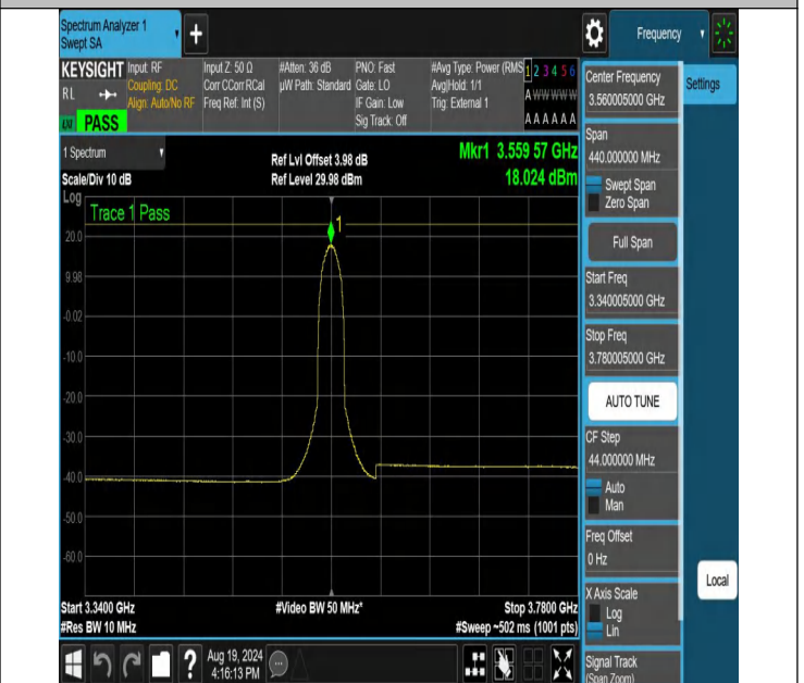
NTNV-N48-PC3-30-20-L-CP-64QAM-Inner_Full-3340.005-3780.005-Ant1-PASS
