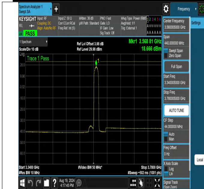
NTNV-N48-PC3-30-20-L-CP-64QAM-Edge_1RB_Right-3340.005-3780.005-Ant1-PASS
