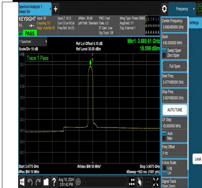
NTN-N48-PC3-30-15-H-CP-QPSK-Edge_1RB_Left-3477.485-3907.485-Ant1-PASS
