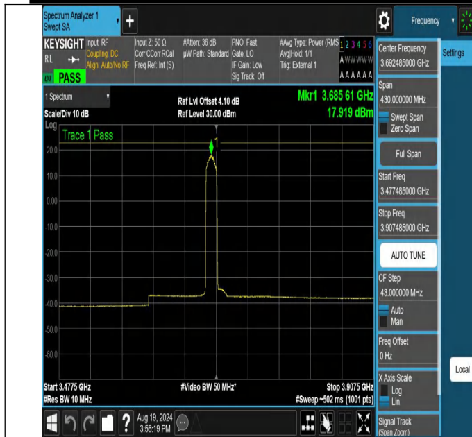
NTN-N48-PC3-30-15-H-CP-64QAM-Edge_1RB_Left-3477.485-3907.485-Ant1-PASS
