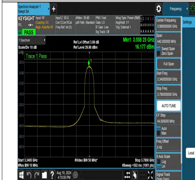
NTNV-N48-PC3-30-20-L-CP-64QAM-Outer_Full-3340.005-3780.005-Ant1-PASS
