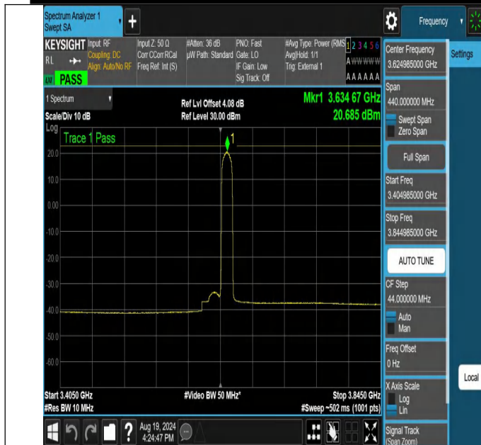
NTNV-N48-PC3-30-20-M-DFT-QPSK-Edge_1RB_Right-3404.985 -3844.985-Ant1-PASS
