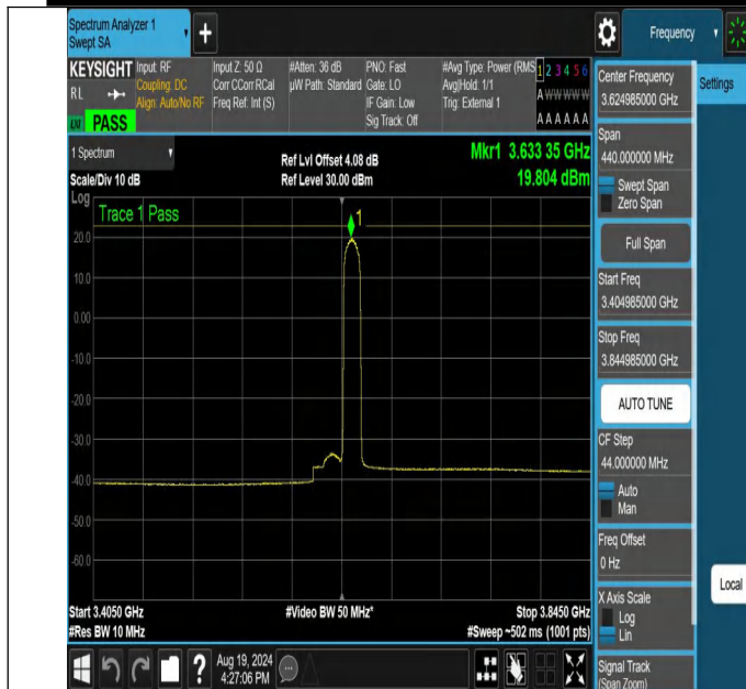
NTNV-N48-PC3-30-20-M-DFT-16QAM-Edge_1RB_Right-3404.985-3844.985-Ant1-PASS
