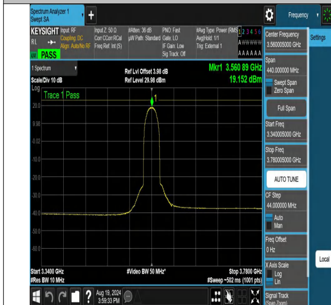
NTNV-N48-PC3-30-20-L-DFT-BPSK-Outer_Full-3340.005-3780.0 05-Ant1-PASS
