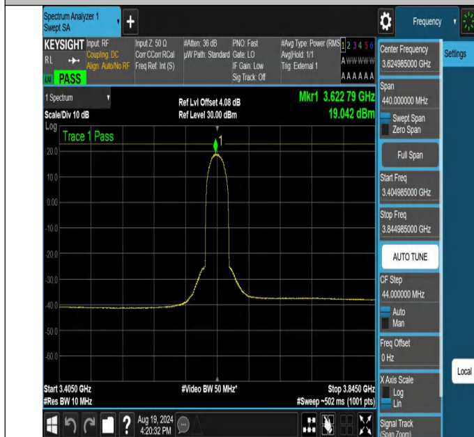
NTNV-N48-PC3-30-20-M-DFT-BPSK-Outer_Full-3404.985-3844.9 85-Ant1-PASS
