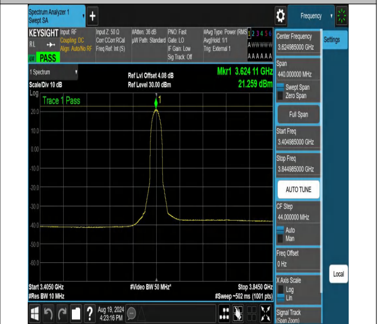
NTNV-N48-PC3-30-20-M-DFT-QPSK-Inner_Full-3404.985-3844.985-Ant1-PASS
