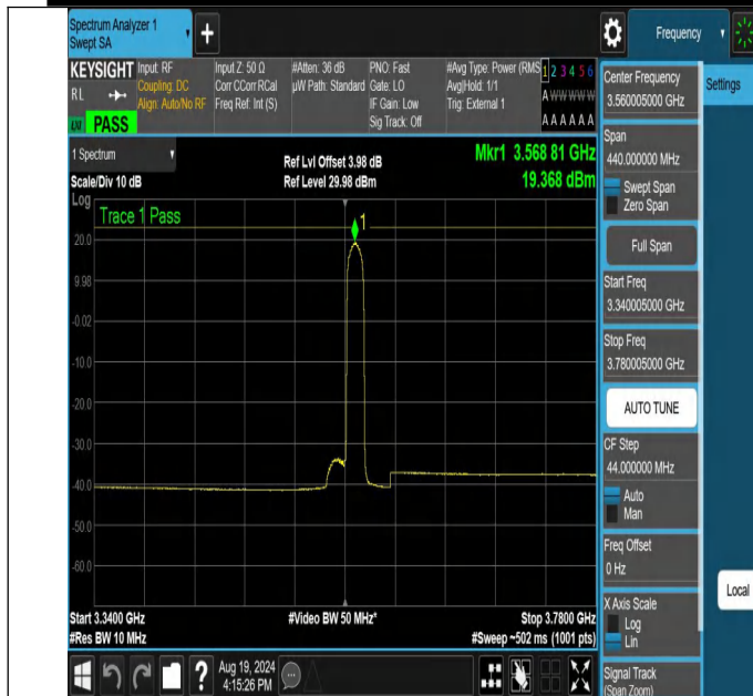
NTNV-N48-PC3-30-20-L-CP-16QAM-Edge_1RB_Right-3340.005-3780.005-Ant1-PASS
