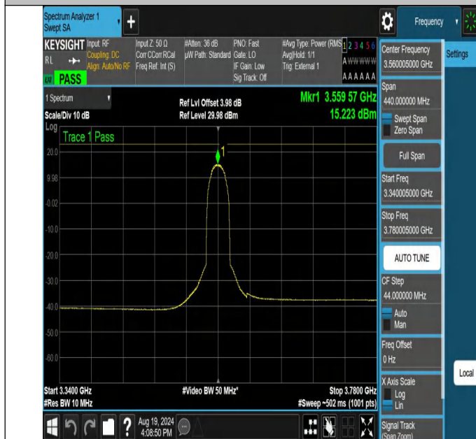
NTNV-N48-PC3-30-20-L-DFT-256QAM-Outer_Full-3340.005-3780.005-Ant1-PASS
