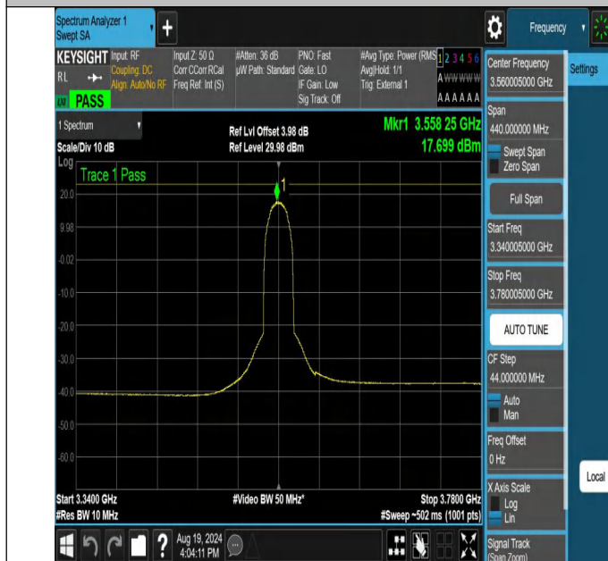
NTNV-N48-PC3-30-20-L-DFT-16QAM-Outer_Full-3340.005-3780.005-Ant1-PASS
