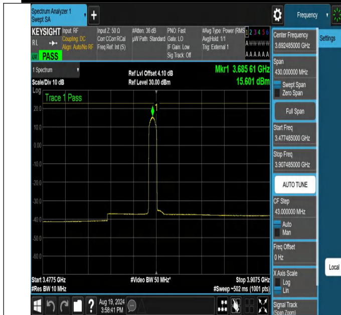
NTNV-N48-PC3-30-15-H-CP-256QAM-Edge_1RB_Left-3477.485-3907.485-Ant1-PASS
