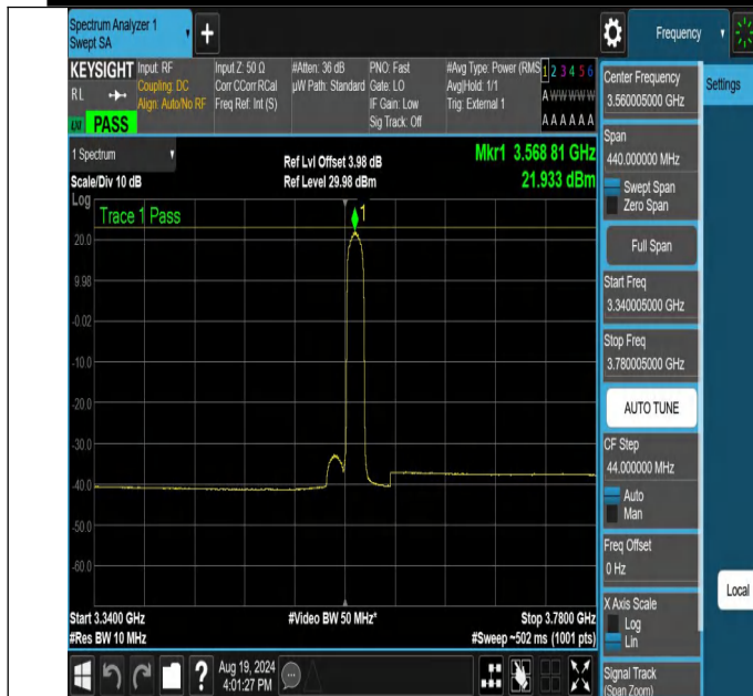
NTNV-N48-PC3-30-20-L-DFT-BPSK-Edge_1RB_Right-3340.005-3780.005-Ant1-PASS
