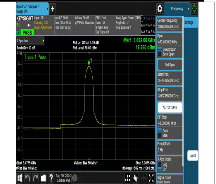
NTN-N48-PC3-30-15-H-CP-QPSK-Outer_Full-3477.485-3907.485-Ant1-PASS
