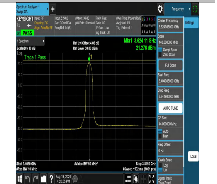
NTNV-N48-PC3-30-20-M-DFT-BPSK-Inner_Full-3404.985-3844.9 85-Ant1-PASS
