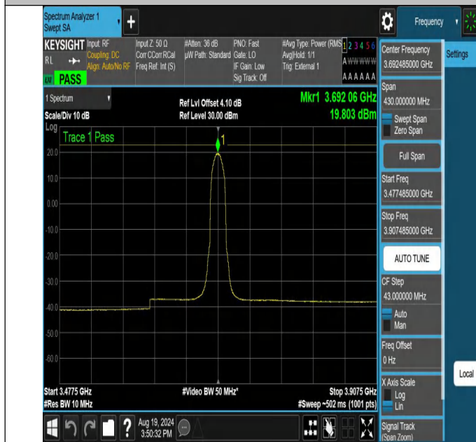
NTN-N48-PC3-30-15-H-CP-QPSK-Inner_Full-3477.485-3907.485-Ant1-PASS
