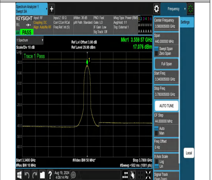
NTNV-N48-PC3-30-20-L-DFT-256QAM-Inner_Full-3340.005-3780.005-Ant1-PASS
