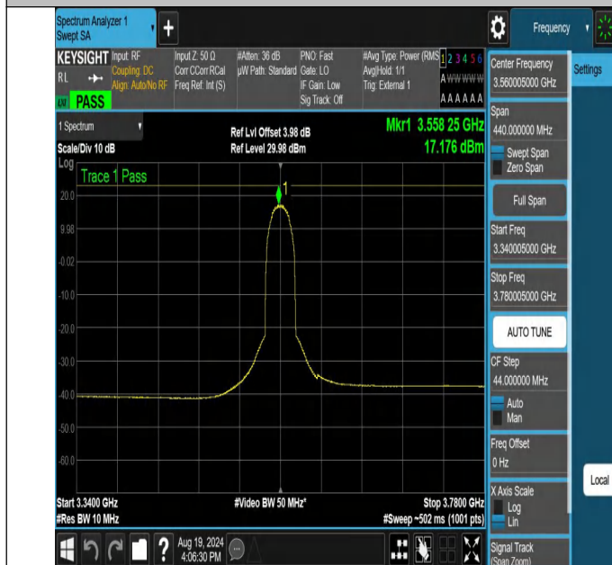
NTNV-N48-PC3-30-20-L-DFT-64QAM-Outer_Full-3340.005-3780. 005-Ant1-PASS
