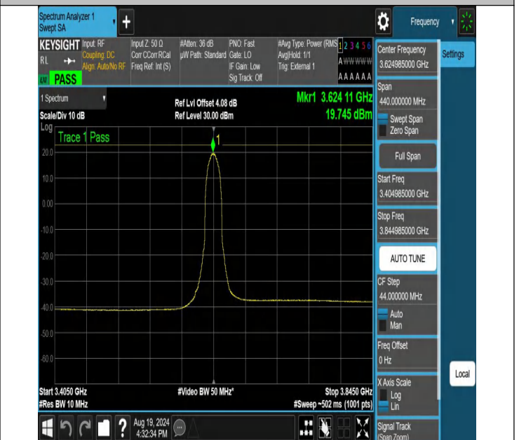
NTNV-N48-PC3-30-20-M-CP-QPSK-Inner_Full-3404.985-3844.985-Ant1-PASS
