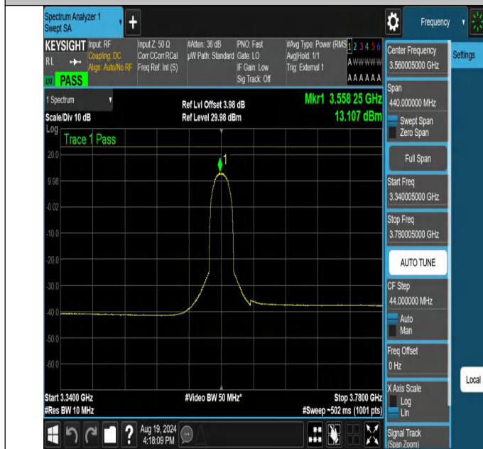
NTNV-N48-PC3-30-20-L-CP-256QAM-Outer_Full-3340.005-3780.005-Ant1-PASS
