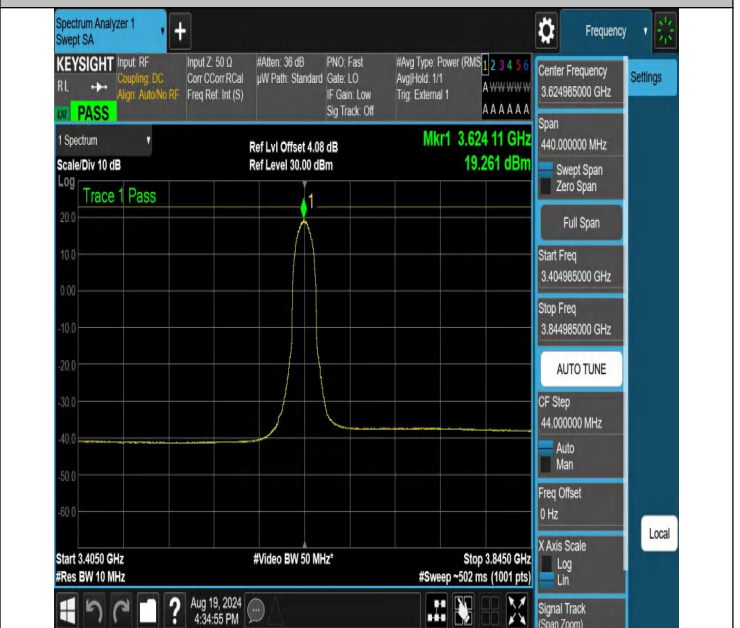
NTNV-N48-PC3-30-20-M-CP-16QAM-Inner_Full-3404.985-3844.985-Ant1-PASS
