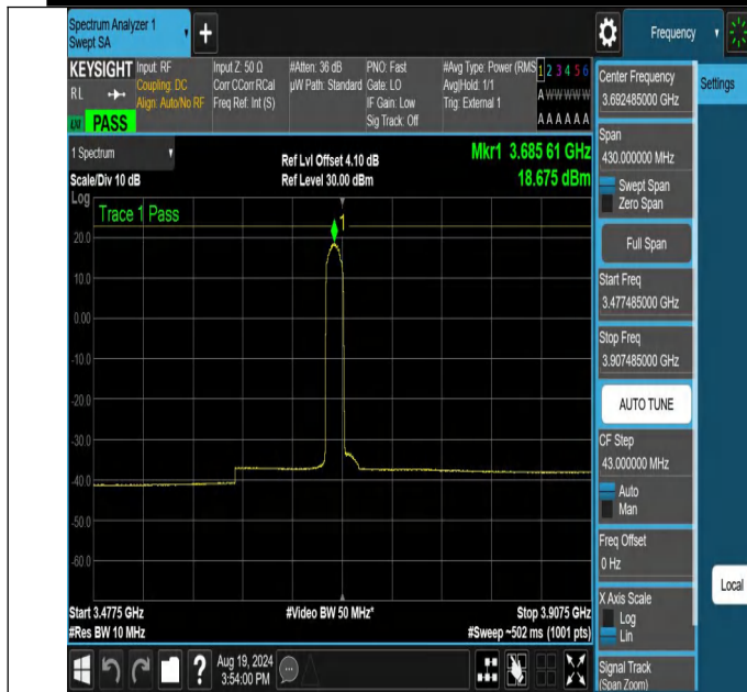
NTN-N48-PC3-30-15-H-CP-16QAM-Edge_1RB_Left-3477.485-3907.485-Ant1-PASS
