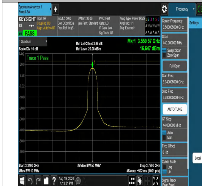
NTNV-N48-PC3-30-20-L-CP-16QAM-Outer_Full-3340.005-3780.005-Ant1-PASS
