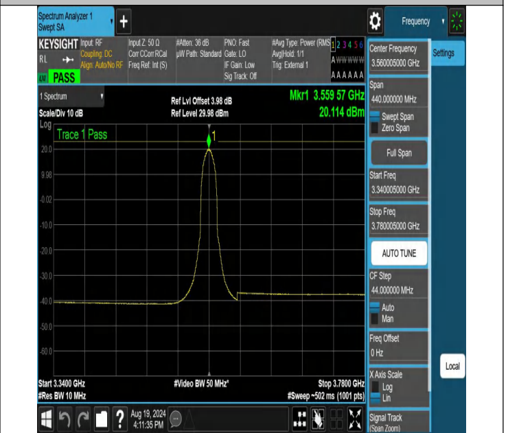
NTNV-N48-PC3-30-20-L-CP-QPSK-Inner_Full-3340.005-3780.00 5-Ant1-PASS
