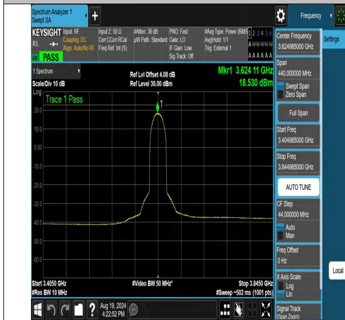
NTNV-N48-PC3-30-20-M-DFT-QPSK-Outer_Full-3404.985-3844.985-Ant1-PASS
