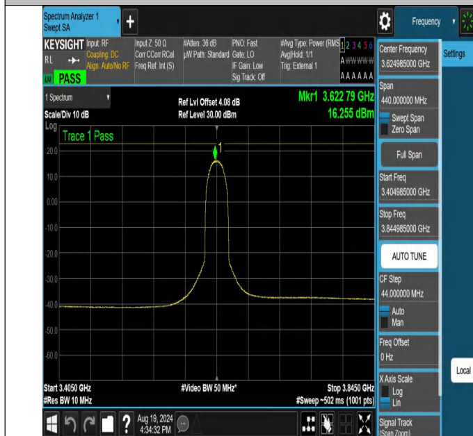
NTNV-N48-PC3-30-20-M-CP-16QAM-Outer_Full-3404.985-3844.985-Ant1-PASS
