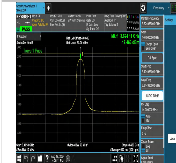
NTNV-N48-PC3-30-20-M-DFT-16QAM-Outer_Full-3404.985-3844. .985-Ant1-PASS
