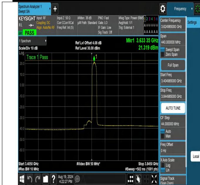
NTNV-N48-PC3-30-20-M-DFT-BPSK-Edge_1RB_Right-3404.985-3844.985-Ant1-PASS
