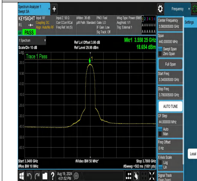
NTNV-N48-PC3-30-20-L-DFT-QPSK-Outer_Full-3340.005-3780.005-Ant1-PASS
