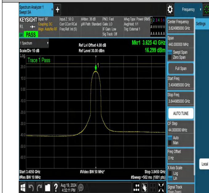
NTNV-N48-PC3-30-20-M-CP-QPSK-Outer_Full-3404.985-3844.985-Ant1-PASS
