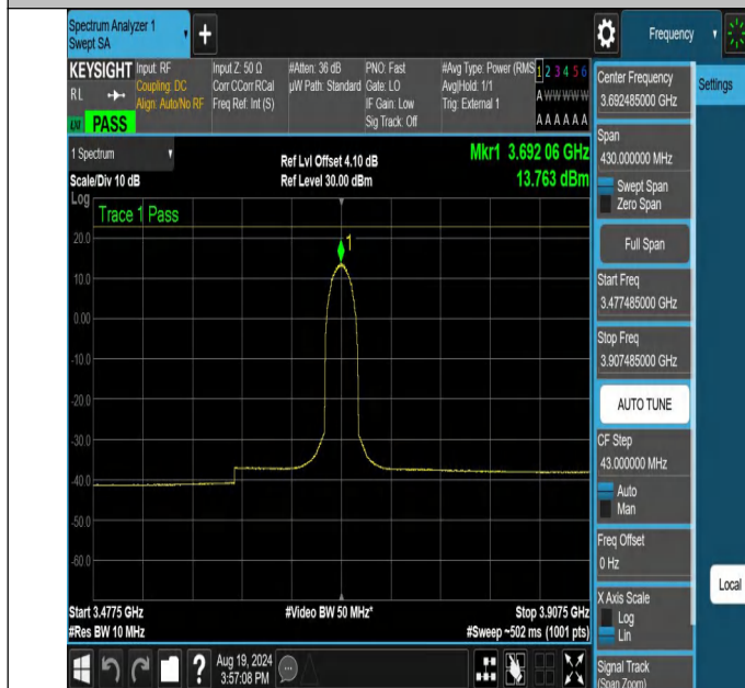
NTNV-N48-PC3-30-15-H-CP-256QAM-Outer_Full-3477.485-3907.485-Ant1-PASS
