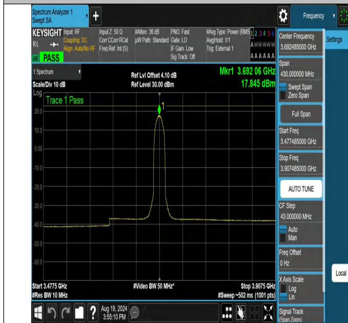
NTN-N48-PC3-30-15-H-CP-64QAM-Inner_Full-3477.485-3907.485-Ant1-PASS
