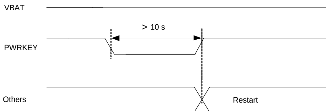
Figure 9: Power-down Timing
