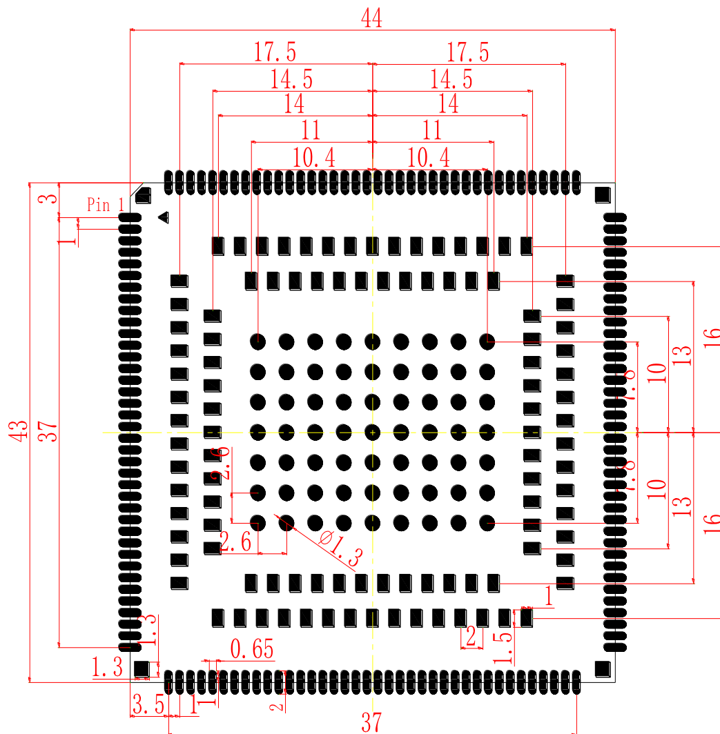
Figure 42: Recommended Footprint
