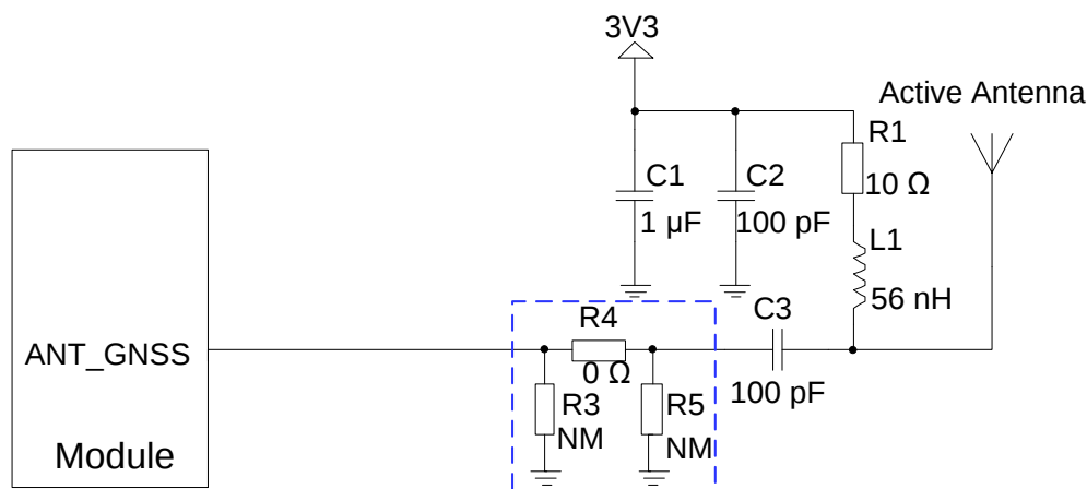
Figure 31: Reference Design for GNSS Active Antenna
