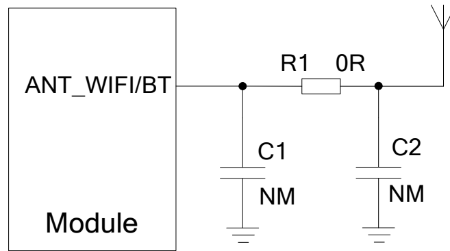
Figure 32: Reference Design for Wi-Fi/Bluetooth Antenna
