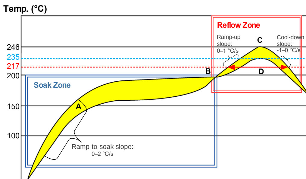
Figure 44: Recommended Reflow Soldering Thermal Profile
