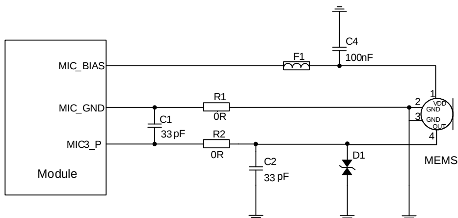
Figure 24: Reference Design for MEMS Microphone Interface
