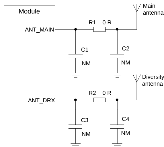
Figure 29: Reference Design for RF Antenna Interfaces
