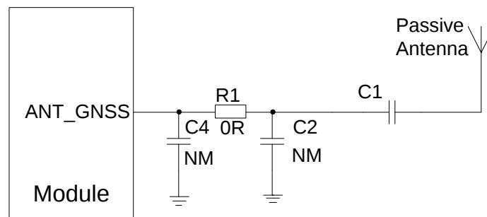
Figure 30: Reference Design for GNSS Passive Antenna
