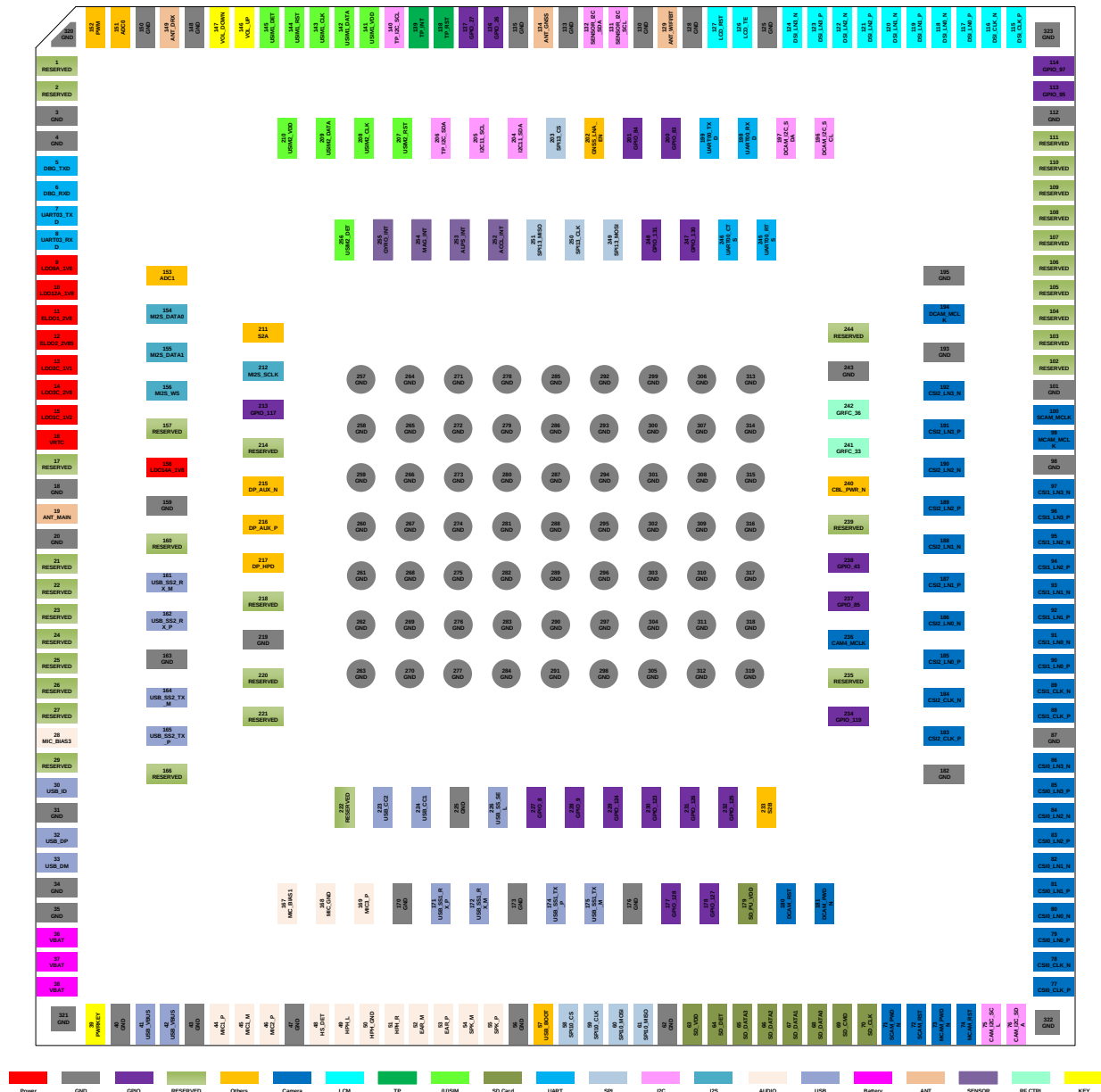
Figure 1: Pin Assignment
