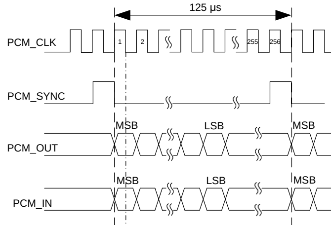
Figure 24: Primary Mode Timing
