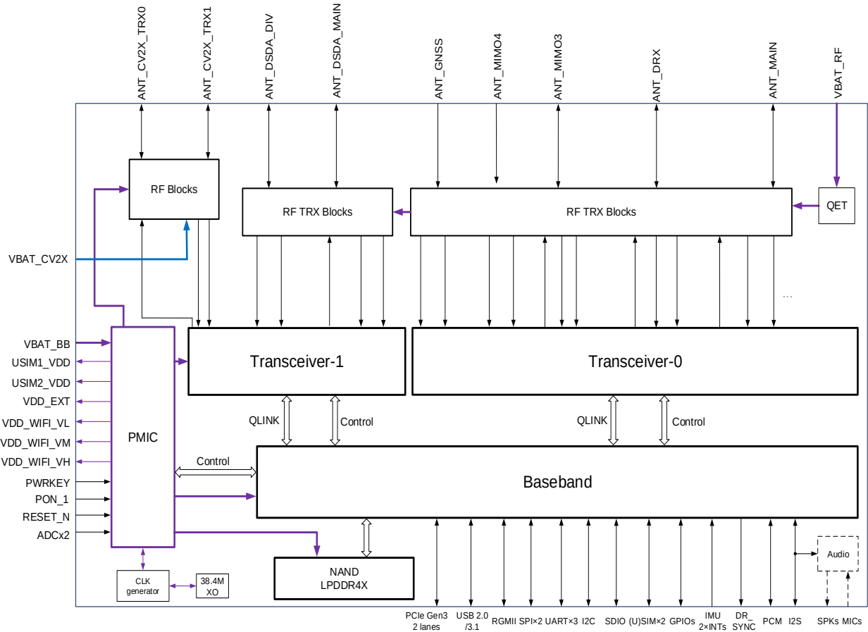
Figure 1: Functional Diagram
