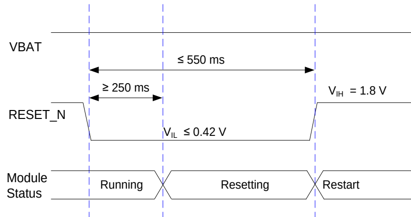
Figure 16: Reset Timing
