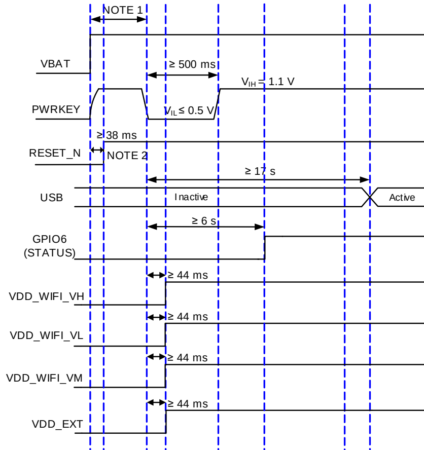
Figure 12: Power-up Timing
