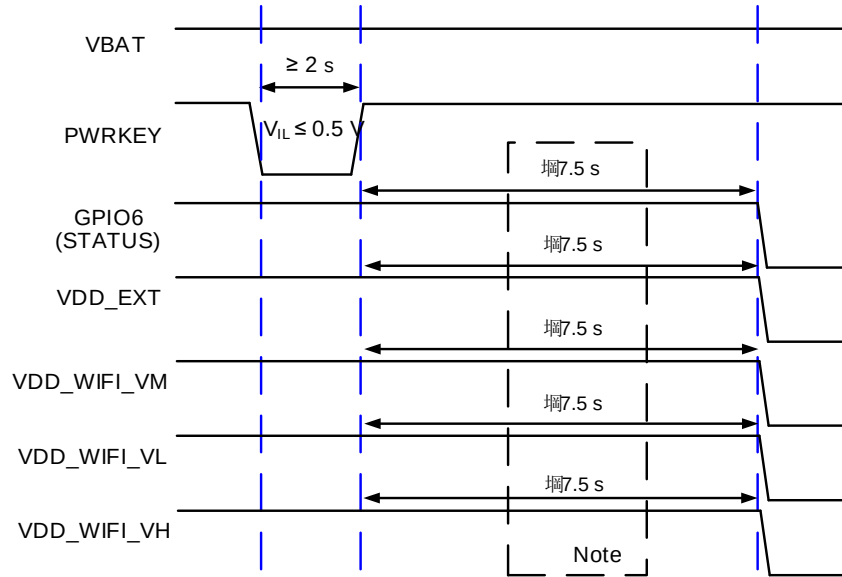
Figure 13: Power-down Timing
