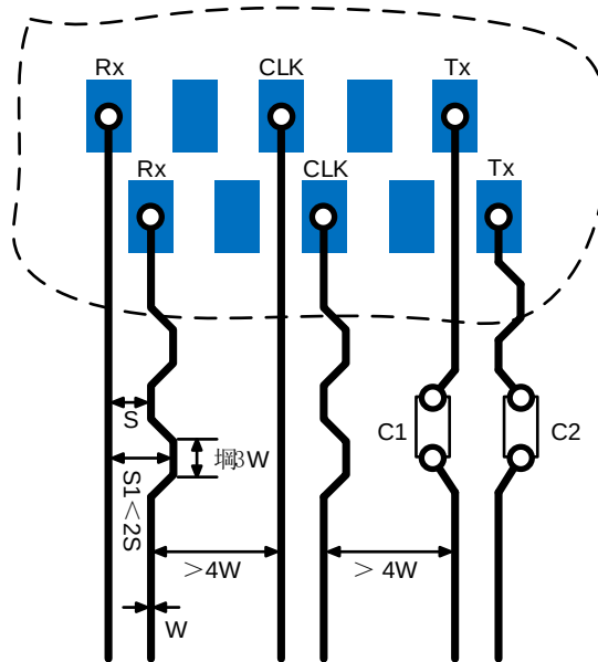
Figure 28: PCIe Trace Requirements
