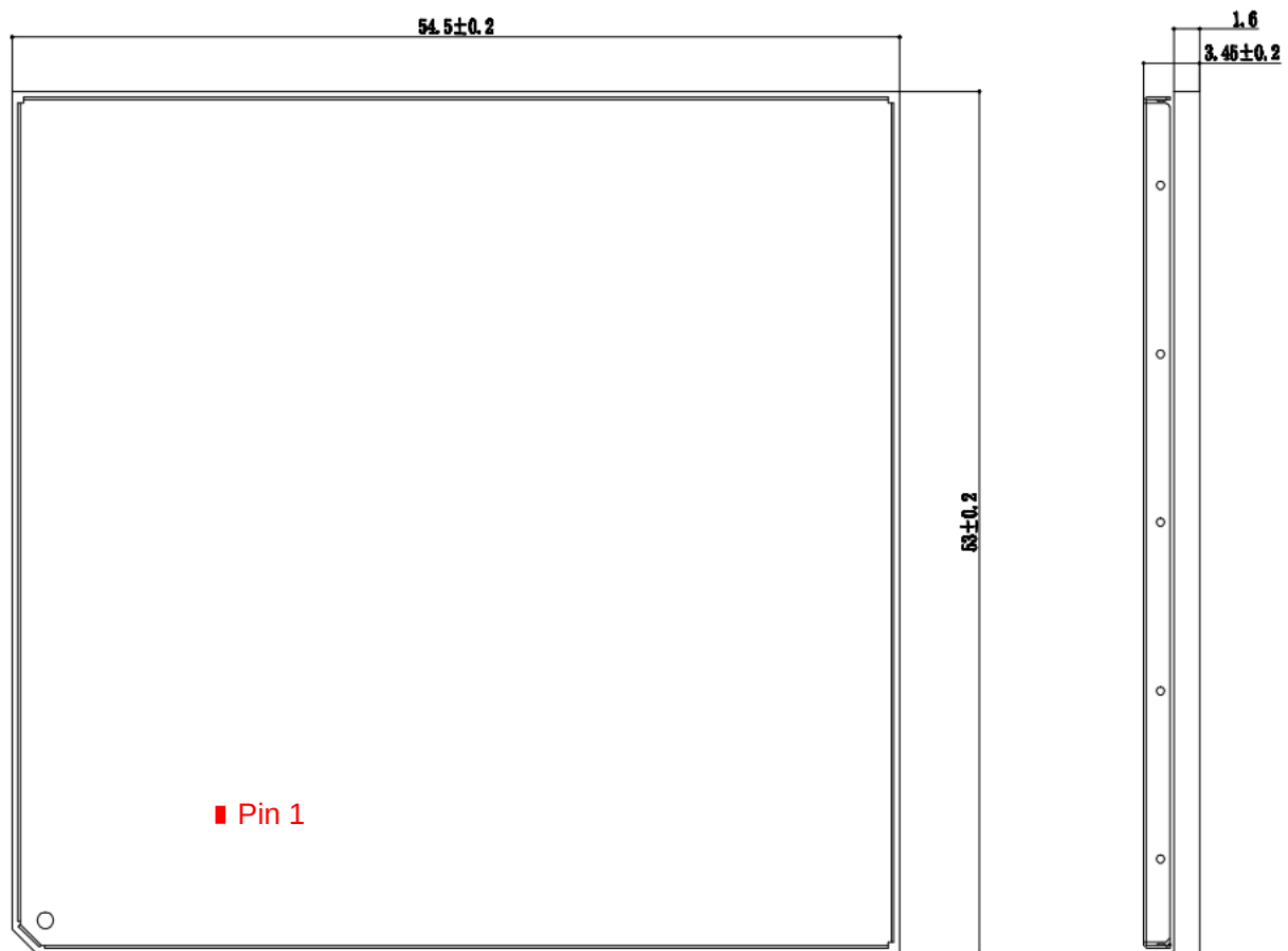
Figure 48: Module Top and Side Dimensions
