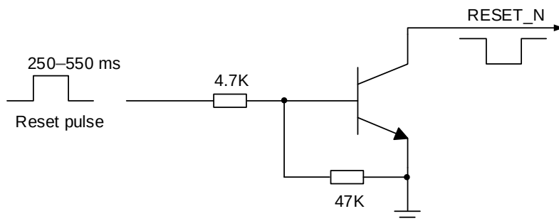
Figure 14: Reference Circuit of RESET_N by Using Driving Circuit
