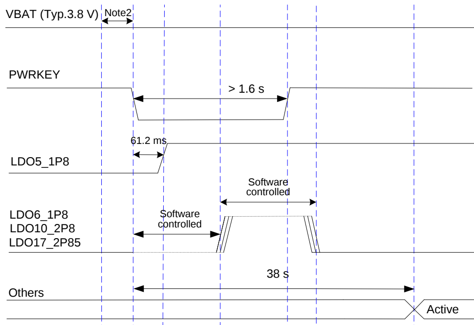
Figure 8: Power-up Timing
