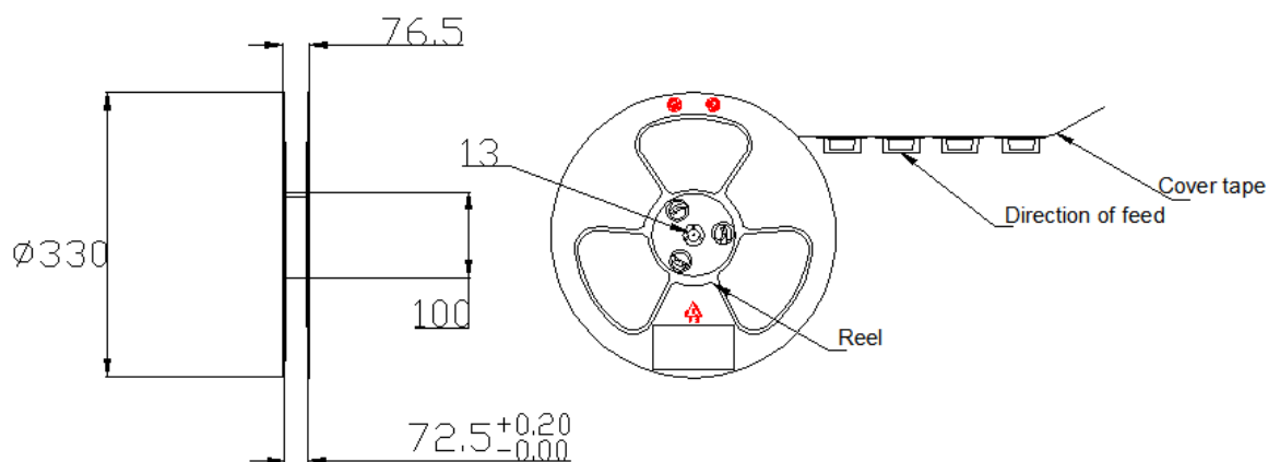
Figure 48: Reel Dimensions
