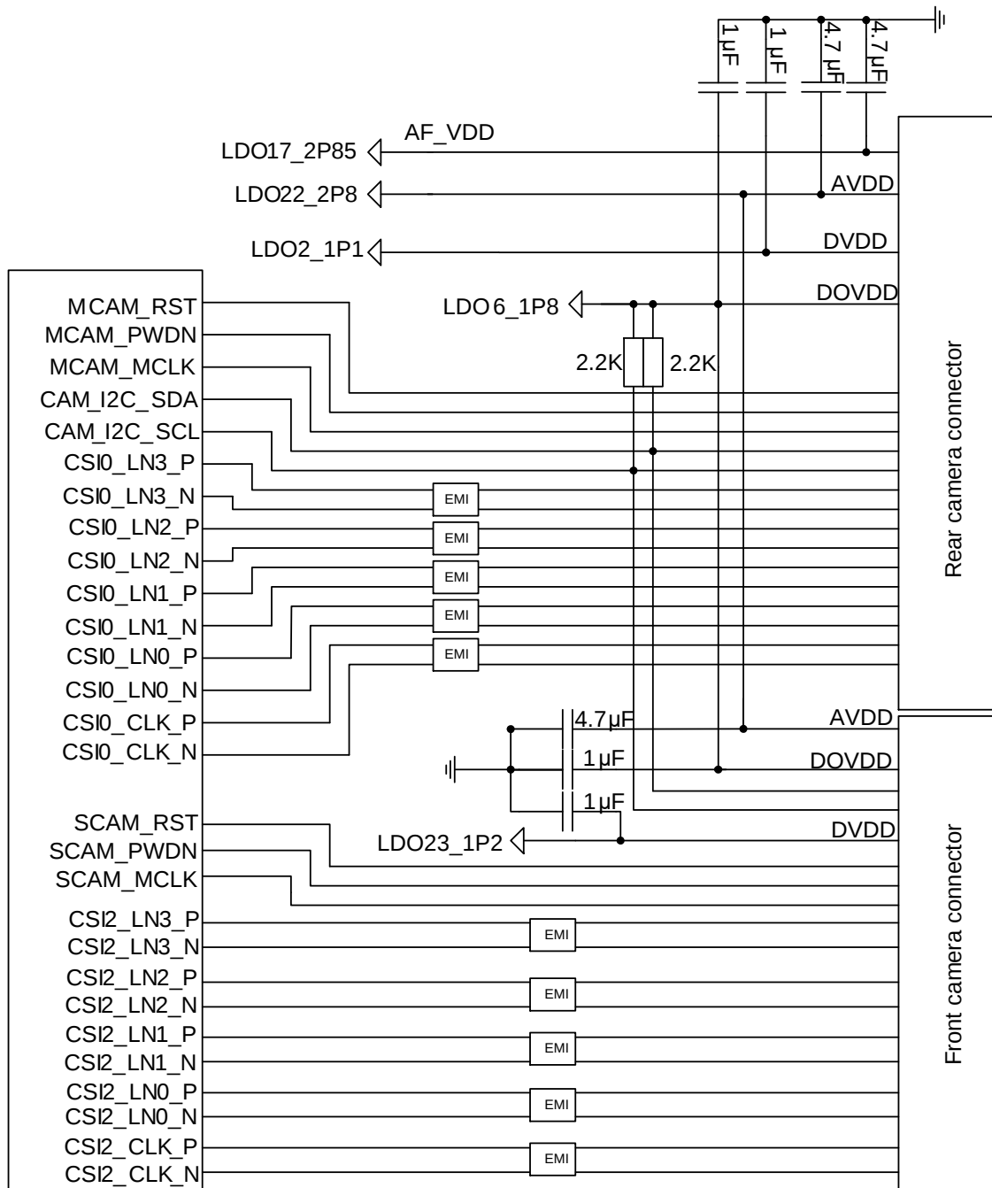
Figure 22: Reference Design for Dual Camera Application
