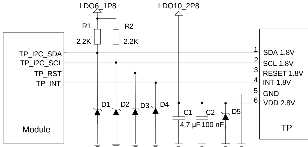
Figure 21: Reference Design for Touch Panel Interface
