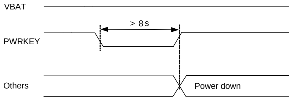
Figure 9: Power-off Timing
