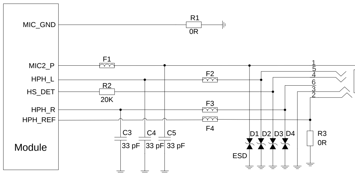
Figure 27: Reference Design for Headphone Interface with Normally Open Jack
