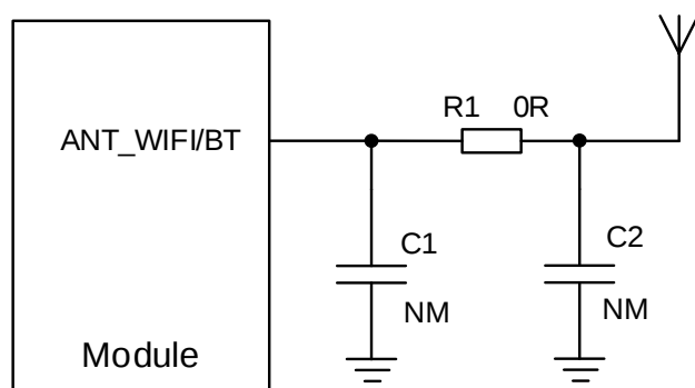
Figure 35: Reference Circuit Design for Wi-Fi/BT Antenna Interface
