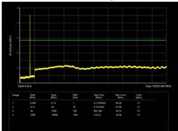
LTE Band 71 15MHz CH-High 9kHz~10GHz
