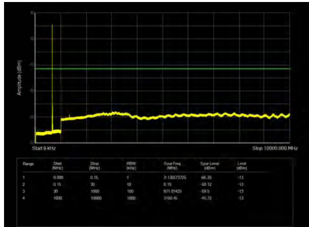
LTE Band 71 20MHz CH- Middle 9kHz~10GHz
