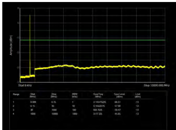
LTE Band 71 20MHz CH- High 9kHz~10GHz
